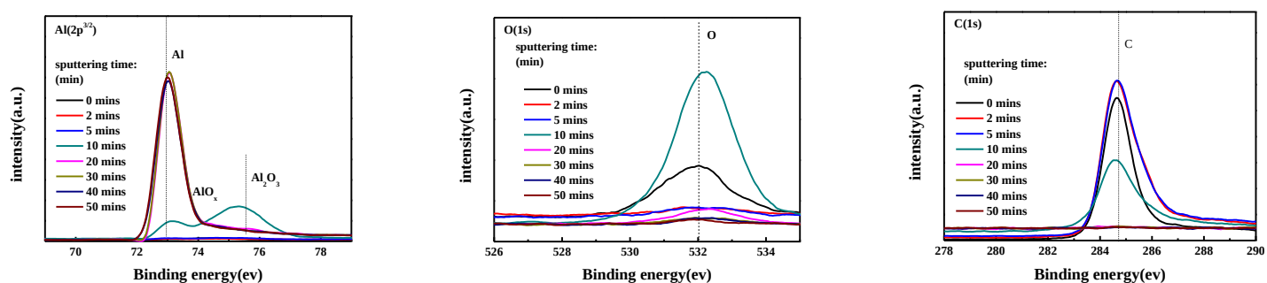
Figure 4(a-c). XPS spectrum of second treated foil in different orbital. Al( 2p^{3/2} )(a), O(1s)(b) and C(1s)(c).
