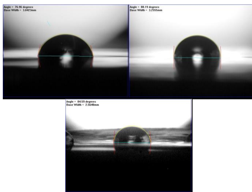
Figure 5(a-d). contact angel of Al(a), first treated(b), second treated Al(c).
