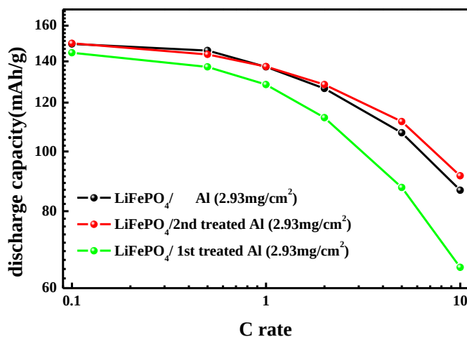
Figure 8. Rate capacity of LFPO electrode with different current collector.
