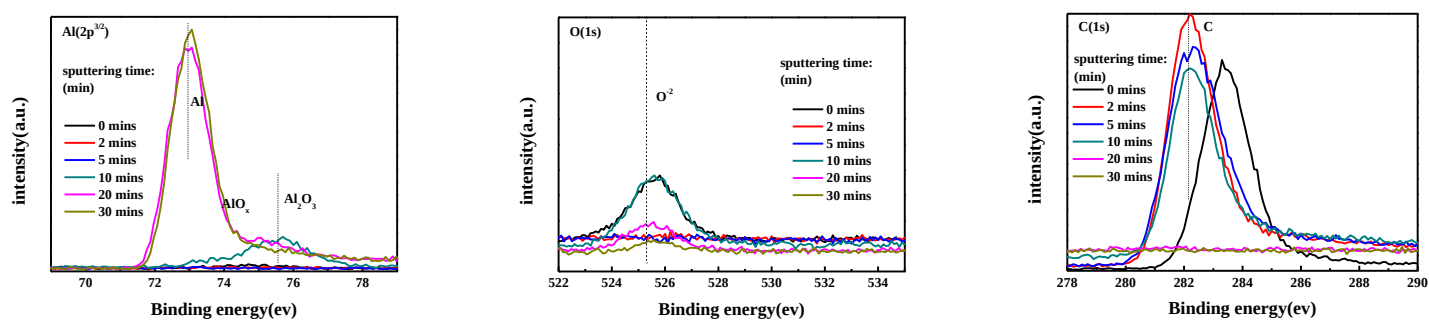
Figure 3(a-c). XPS spectrum of first treated foil in different orbital. Al( 2p^{3/2} )(a), O(1s)(b) and C(1s)(c).
