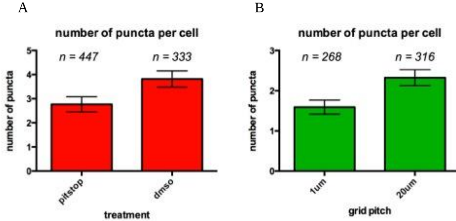
Figure 6. Plots of total internal number of ephrinA1 puncta, which is a readout of the rate of endocytosis of the receptor/ligand pair. A. Number of internal ephrinA1 puncta of cells adhered to an ephrinA1 supported membrane. Cells were treated with the small molecule inhibitor, Pitstop2, or DMSO as a control. B. Number of internal ephrinA1 puncta of cells adhered to an ephrinA1 supported membrane with either 1 \mu m or 20 \mu m gridded substrates. P < 0.05 for both experiments. The number of cells n is reported for each condition.
