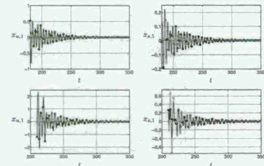
Figure 5.1.18: States of the system with observer-based control; the states reconstructed (---, x ) by a 22-mode observer quickly converge to the actual states (—, \delta ). The initial conditions used are those corresponding to t = 180, 210 (top and bottom) of the uncontrolled case shown in Fig. 5.1.17.
