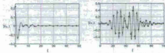
Figure 5.1.11: Comparison of the outputs y_{a,1} and y_{a,2} of a 12-mode reduced-order model (—) with the projection of data from the linearized simulation (---). The control gain is obtained using LQR, and the initial condition is that obtained by an impulsive input to the system. Control is turned on at t = 0 .
