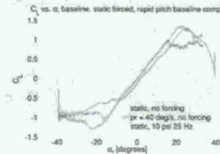
Fig. 3.4.4: Lift dependence on angle of attack. Forcing on at 25 Hz, C_p = .0074 and pitch rates \dot{\alpha}/dt = 0.9 and 40 deg/sec. Forcing in the "static" case produces same lift coefficient as the dynamic case.
