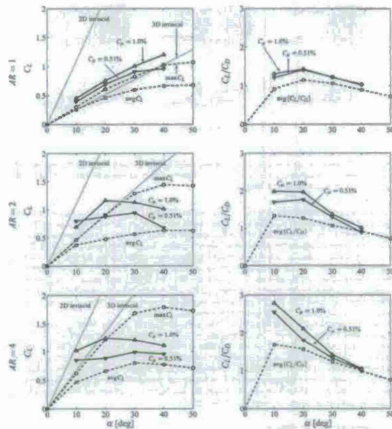
Figure 6.2.6: Time-average lift coefficients and lift-to-drag ratios for wings of AR = 1, 2 , and 4 for cases without actuation ( \square ) and with actuation for C_b = 0.51\% ( \circ ) and 1.0\% ( \triangle ). Shown also are the maximum lift for unactuated case ( - ) and the inviscid limits ( --- ).
