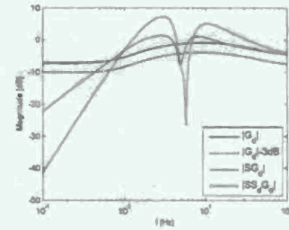
Fig. 3.6.7: Frequency response of the plant output to sinusoidal disturbances in the flow speed for the uncontrolled plant (blue line), the feedback controlled plant (green line) and the feedback controlled plant augmented by a feedforward disturbance compensation (red line).
