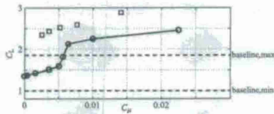
Figure 5.2.15: Average lift of optimized control ( \square ) and closed-loop sinusoidal forcing ( \circ ) at different values of C_\mu at \alpha = 40^\circ .
