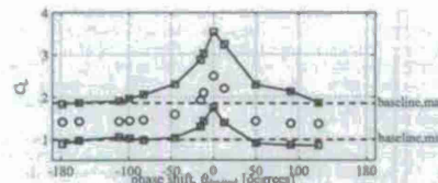
Figure 5.2.17: Maximum and minimum lift ( \square ) and average lift ( \diamond ) of phase-locked limit cycles at different phase shift with optimized waveform ( N_k = 10 ) at \alpha = 40^\circ . Maximum and minimum lift of baseline ( \circ ) case is shown as a reference.
