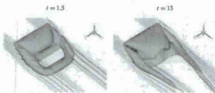
Figure 4.1.13: Top view of vortical structure behind a rectangular plate of AR = 2 and \alpha = 30^\circ represented by an iso-surface of Q = 1 for Re = 100 at different times. Streamlines are overlaid with color contour indicating the local velocity norm from blue to red in increasing magnitude. Flow direction from top left to bottom right.
