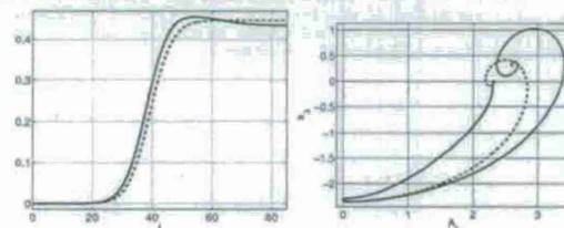
Figure 4.7.2: A subgrid model for a LOGM comprising of the leading attractor POD mode pair and the shift mode. The turbulence energy state u_T = \sqrt{K^2} , is well approximated by slaving it to the squared leading oscillations amplitude (left). A LOGM containing nonlinear subgrid model (right, dashed) eliminates the over-prediction of the NSE attractor (right, solid) amplitude and reduces the transient overshoot of the original LOGM (right, dotted). The remaining mismatch is the result of model deformation, as discussed below.
