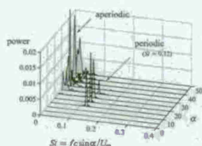
Figure 6.1.7: Power spectra of the lift force for a rectangular plate of AR = 3 in flows of Re = 500 at various angles of attack.
