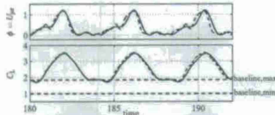
Figure 5.2.16: Comparison between feedback control cases with optimized waveform at \alpha = 40^\circ : N_k = 10 (dashed) and N_k = 4 (solid).
