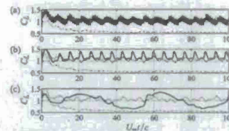
Figure 6.3.2: Time trace of lift ( --- ) for (a) \omega_b/\omega_k = 4 , (b) \omega_b/\omega_k = 0.75 , and (c) \omega_b/\omega_k = 0.1 with the unactuated and \omega_b/\omega_k = 1 results superposed as ( --- ) and ( --- ), respectively.
