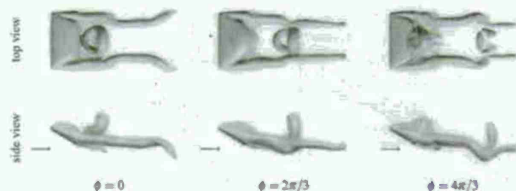
Figure 6.3.3: Snapshots of the periodically time-varying wake structures shown at one-third phase intervals for the periodically actuated case with \omega_{act}/\omega_h = 0.75 . Shown are the iso-surfaces of \|\omega\|_2 = 3 (light gray) and Q = 2.5 . Arrows indicate the flow direction.
