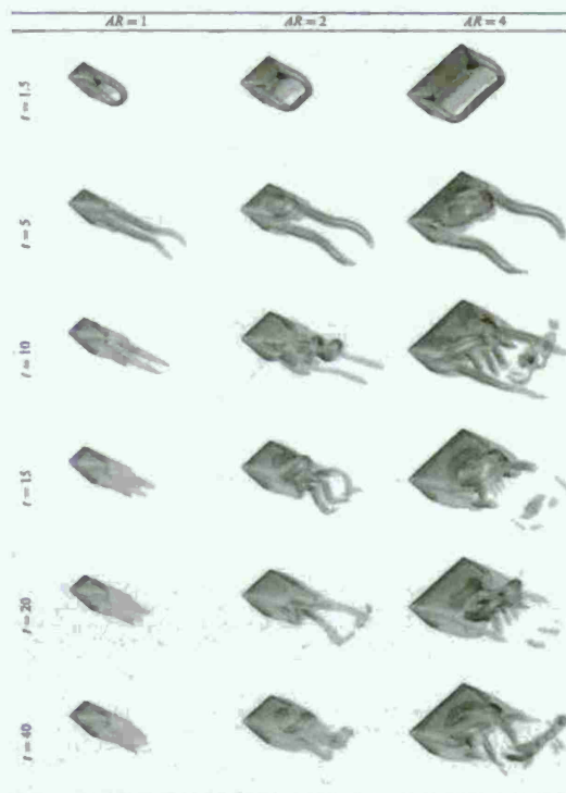
Figure 6.1.2: Top-port views of the wake vortices behind rectangular plates of AR = 1, 2 , and 4 at \alpha = 30^\circ and Re = 300 . Shown are the iso-surface of \|\omega\| = 1.5 in light gray with vortex cores highlighted by the iso-surface of Q = 3 in dark gray.
