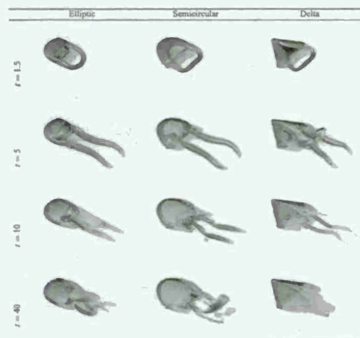
Figure 6.1.10: Top-port views of the wake vortices behind different planform geometries at \alpha = 30^\circ and Re = 300 with the iso-surface of |\mathbf{u}|u| = 3 in light gray with vortex cores highlighted by the iso-surface of Q = 3 in dark gray.
