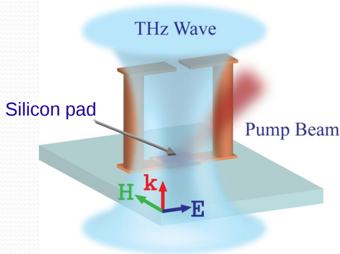
Double splits ring resonator
