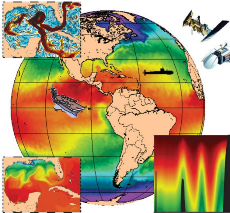
Figure 9. Global NCOM assimilates satellite measurements of sea surface temp. and elevation to produce forecasts of temperature, salinity, elevation and currents that support Navy operations (From NRL Stennis 2006)
