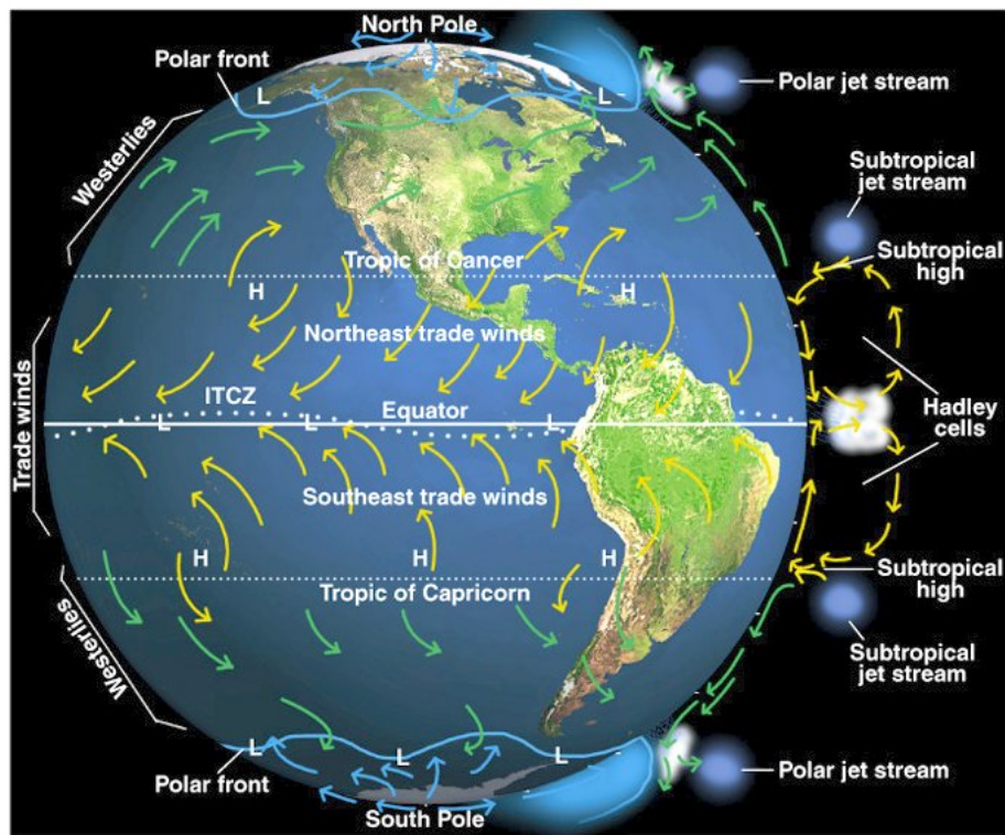
Figure 3. Global wind patterns (From Scripster 2012)
