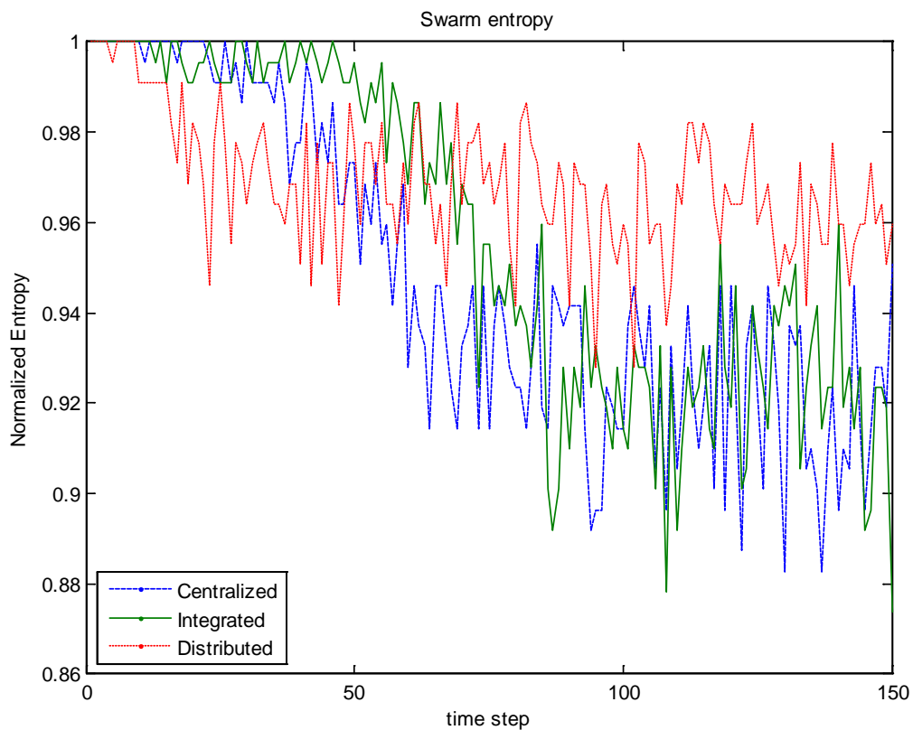
Figure 27 Spatial entropy over time for the “Rally-integration” scenario.
