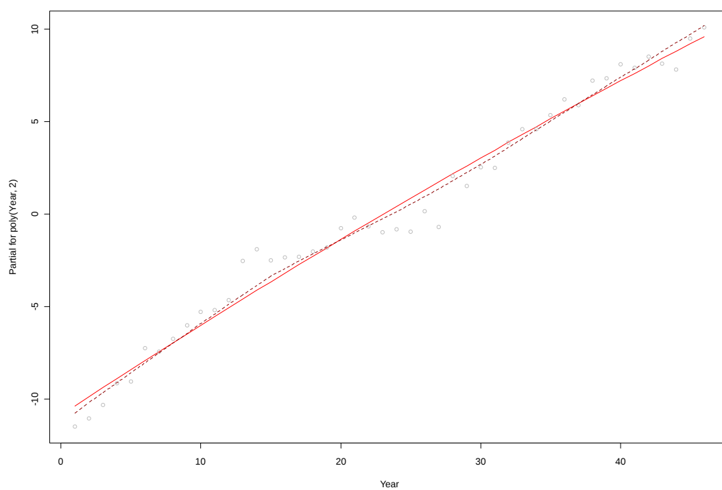
Figure 21. R partial residual plots of JSTOR^{0.5} \sim Year vs. JSTOR^{0.5} \sim poly(Year, 2) .
