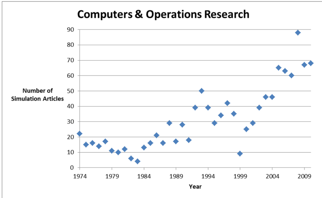
Figure 10. Computers & Operations Research simulation articles over time.
