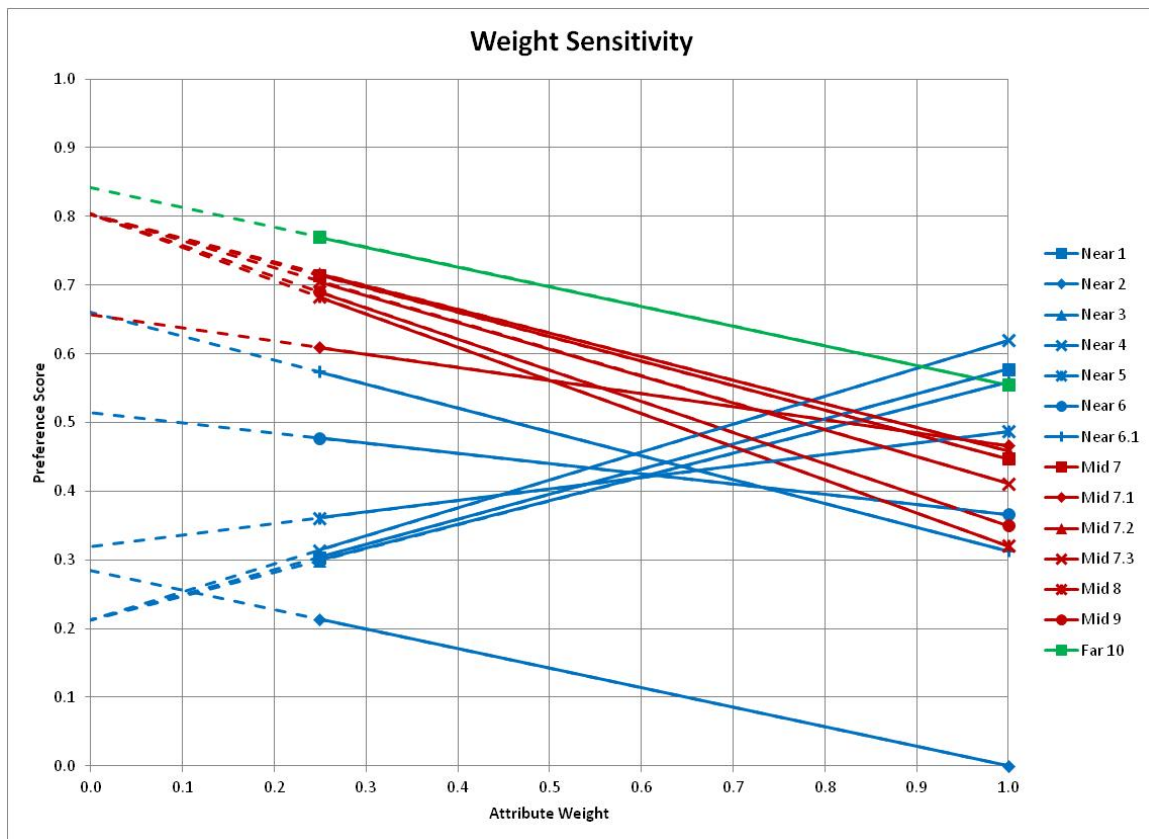
Figure 25. Weight Sensitivity
