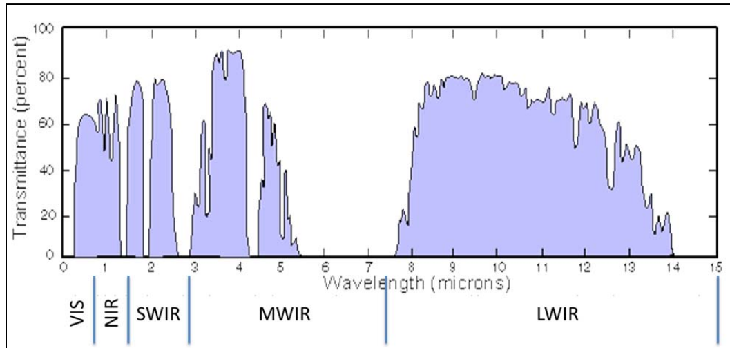
Figure 38. Atmospheric Absorption and Wavebands, After [23]
