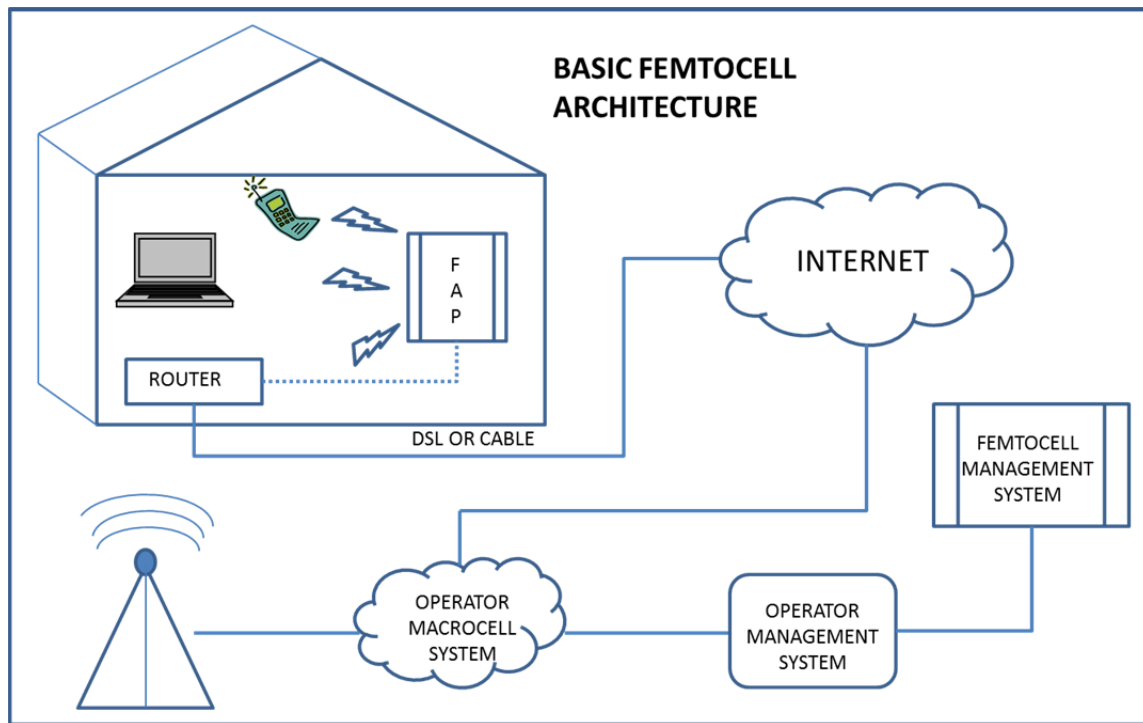
Figure 2. Basic femtocell architecture
