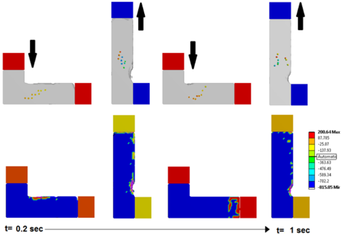
Figure 3.11 ECAP 4 pass Route C results at 0.7 T_{\text{Melt}} at a strain rate of 10^{-6} \text{ sec}^{-1} with a C_f = 0.9 and the corresponding hydrostatic pressure.
