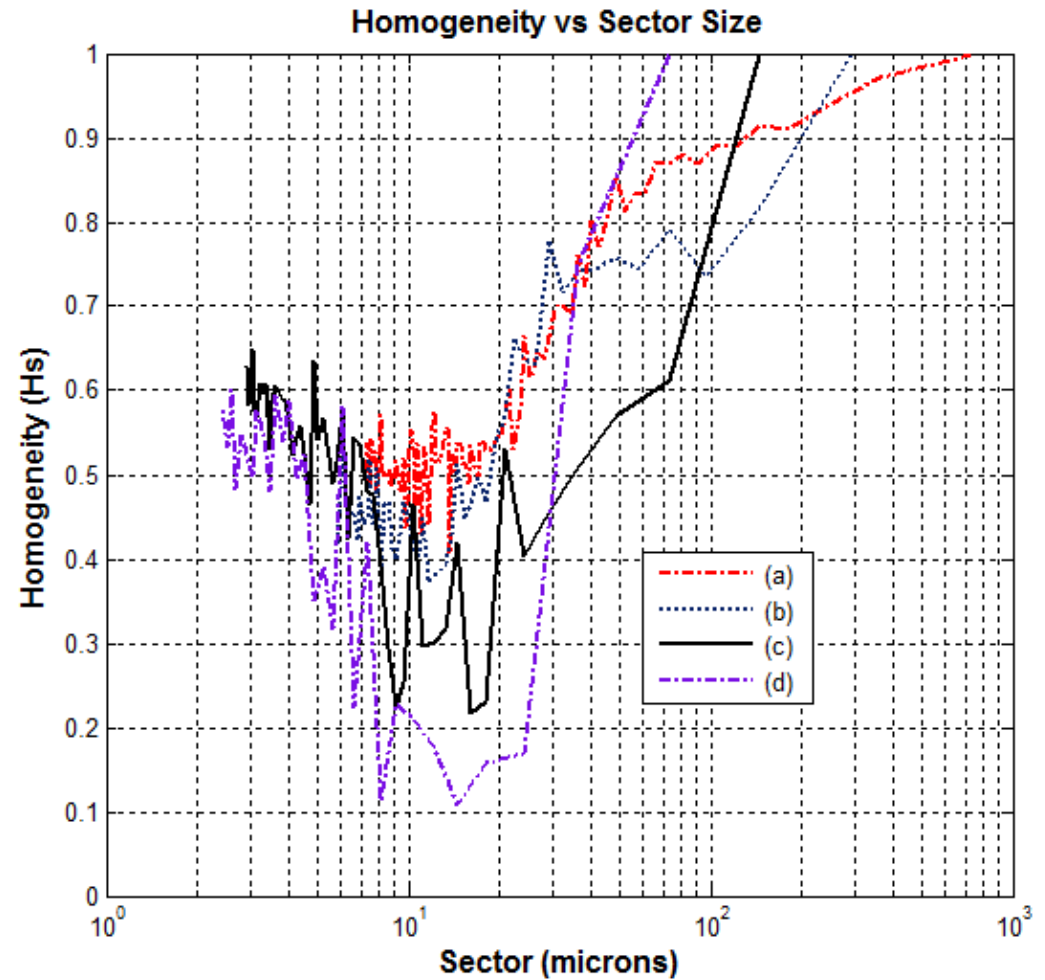
Figure 5.8 The calculated Homogeneity ( H_s ) based on the measured parameter values for (a) AA356 where (b),(c), and (d) are 2, 5, and 10 times smaller in area than (a). Measurements were obtained over a wide range of sector sizes, at different sites but for the same as-cast material. The plot illustrates the index sensitivity to the number of particles in the image.
