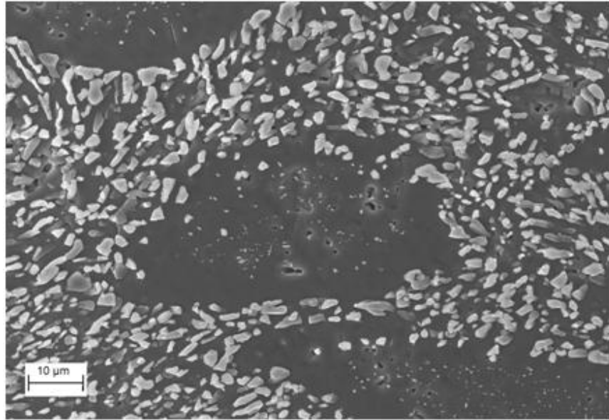
Figure 3.19 Two pass 300°C Al-7% Si secondary electron image of the flow plane after Route C.
