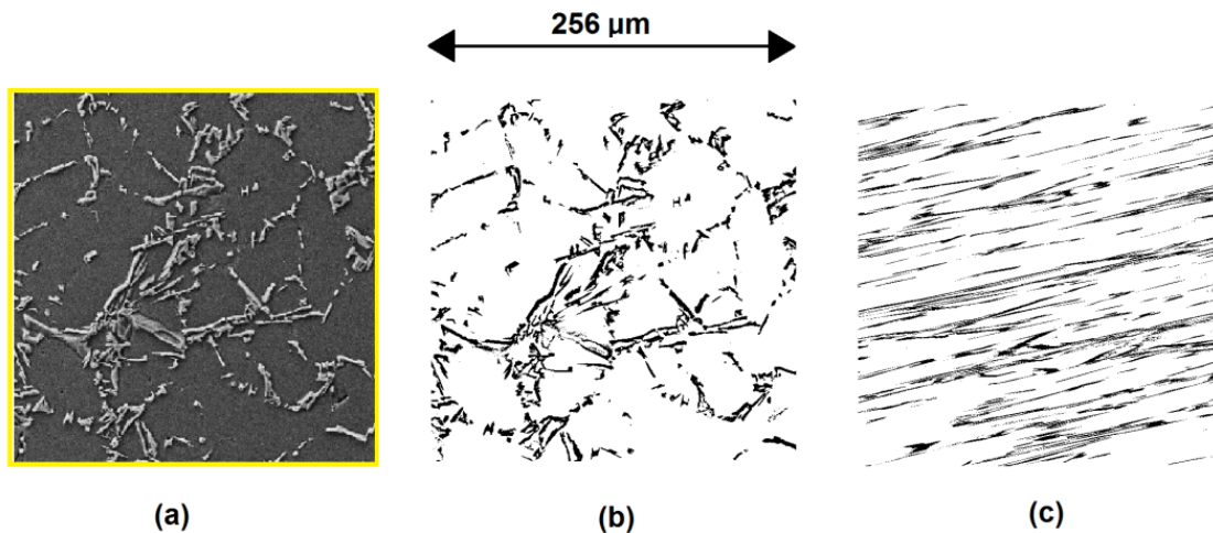
Figure 6.12 (a) Secondary electron image of as-cast AA356 (b) binary image of as-cast (c) binary image of AA-356 digitally sheared in a linear, monotonic strain gradient to a strain of 4.
