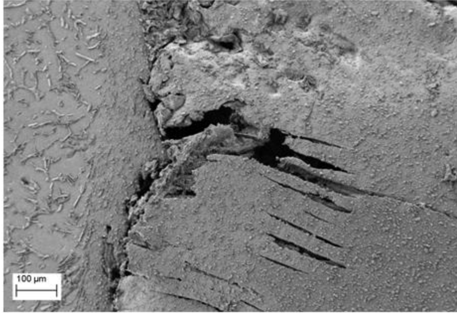
Figure 4.29 Secondary electron plan view image of insufficiently re-bonded void extrusion layers in the lower section of the stir along the advancing side for a 2000 RPM smooth pin approximately 5 mm back from the extraction site.
