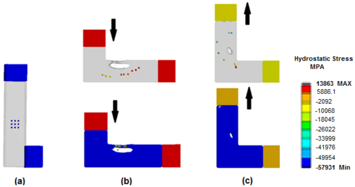
Figure 3.10 (a) Original billet configuration with an array of 9 particles (b) ECAP pass 1 using Route C at 0.7 T_{Melt} , strain rate of 10^{1.9} \text{ sec}^{-1} with a C_f = 0.9 and the corresponding hydrostatic pressure during shear (c) ECAP pass 2 with Route C at 0.7 T_{Melt} , strain rate of 10^{1.9} \text{ sec}^{-1} , C_f = 0.9 and the corresponding hydrostatic pressure gradient during shear.
