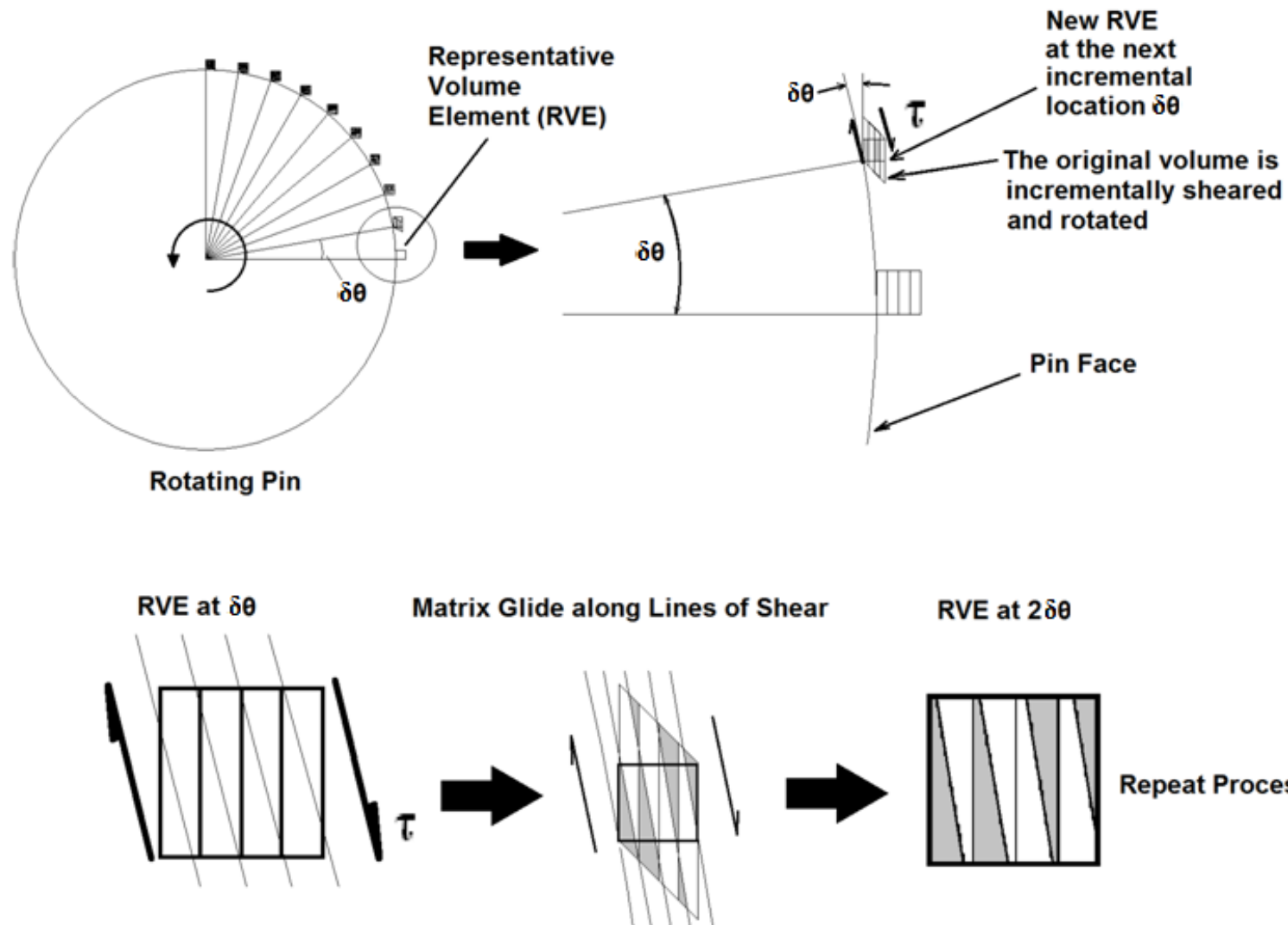
Figure 6.3 Schematic of an extrusion layer volume element with periodic boundary conditions at the pin-material interface experiencing an incremental rotation while subject to continuous shear.
