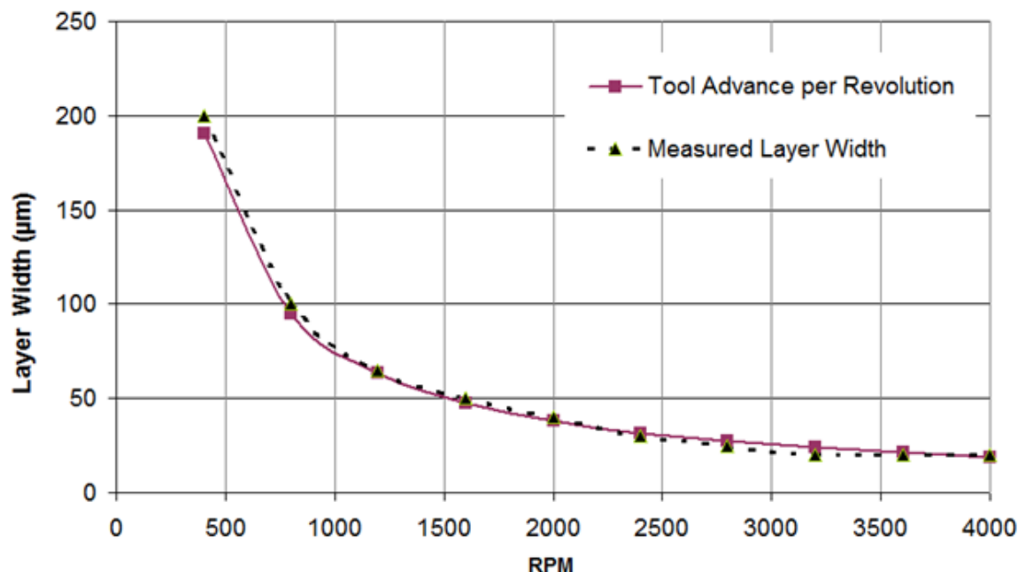
Figure 4.22 Tool translation distance per revolution and measured extrusion layer thickness plotted vs. RPM for the smooth tool.
