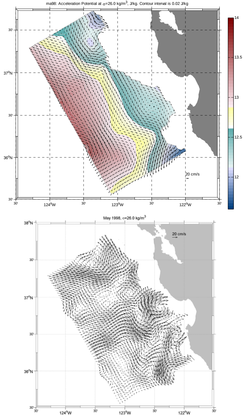
Figure 31. Acceleration potential in J/kg during May 1998 (upper) and ADCP velocities in cm/s (lower) for the 26.0 kg/m 3 density surface. Contour interval is 0.02 J/kg (upper) and the magnitude of flow is given by the arrow shown in the upper right corner (lower).
