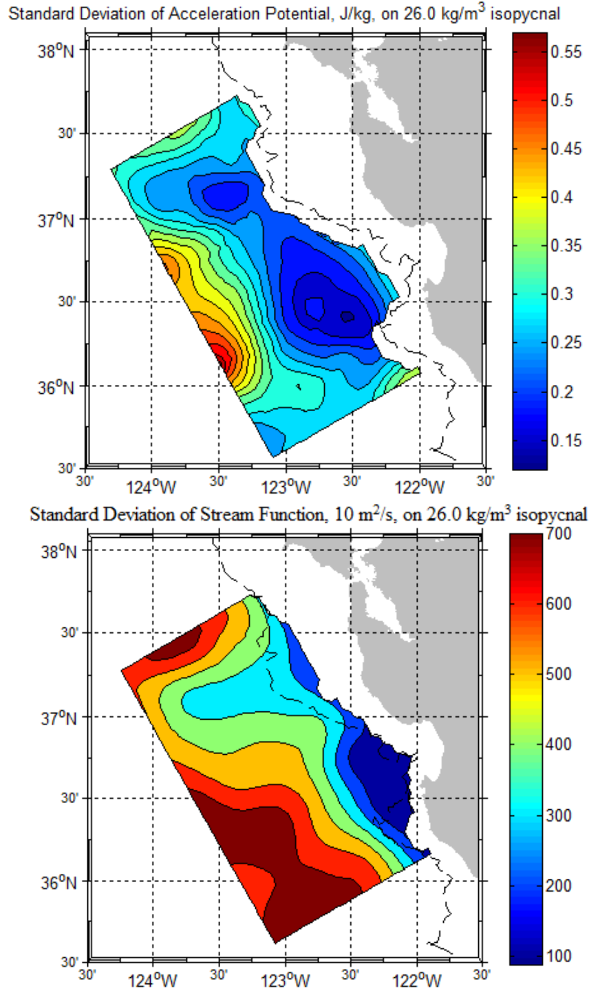
Figure 9. Standard deviation of mean acceleration potential in J/kg for the 26.0 \text{ kg/m}^3 density surface (upper) and standard deviation of mean stream function in 10 \text{ m}^2/\text{s} for the 26.0 \text{ kg/m}^3 density surface (lower). Contour interval is .03 J/kg (upper) and 50 10 \text{ m}^2/\text{s} (lower).
