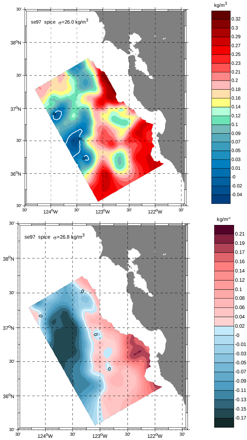
Figure 23. Spiciness in \text{kg/m}^3 during September 1997 for the 26.0 \text{ kg/m}^3 (upper) and 26.8 \text{ kg/m}^3 (lower) density surfaces. Contour interval is 0.018 \text{ kg/m}^3 (upper) and .019 \text{ kg/m}^3 (lower). White denotes zero spiciness contour.
