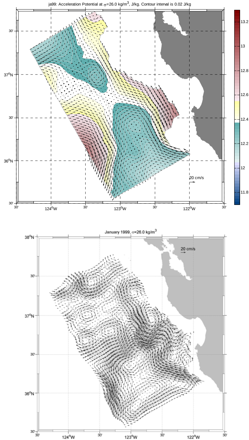
Figure 45. Acceleration potential in J/kg during January 1999 (upper) and ADCP velocities in cm/s (lower) for the 26.0 kg/m 3 density surface. Contour interval is 0.02 J/kg (upper) and the magnitude of flow is given by the arrow shown in the upper right corner (lower).
