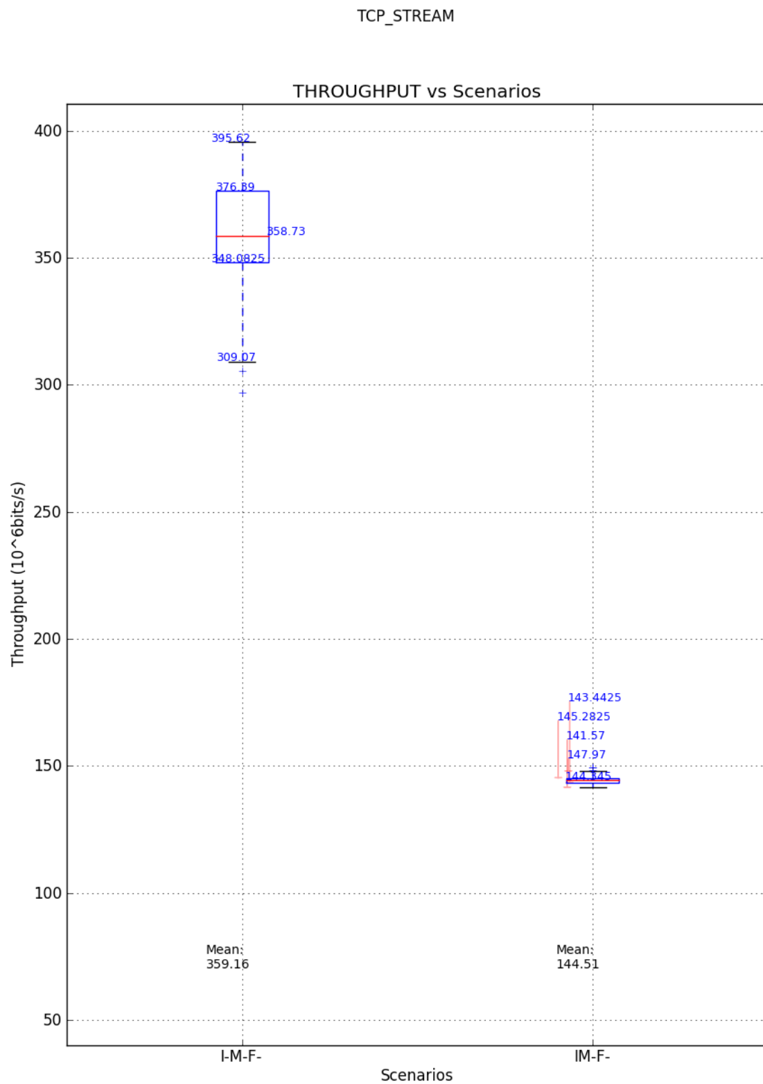
Figure D.1: Boxplots comparison of IPSec using TCP_STREAM Tests
