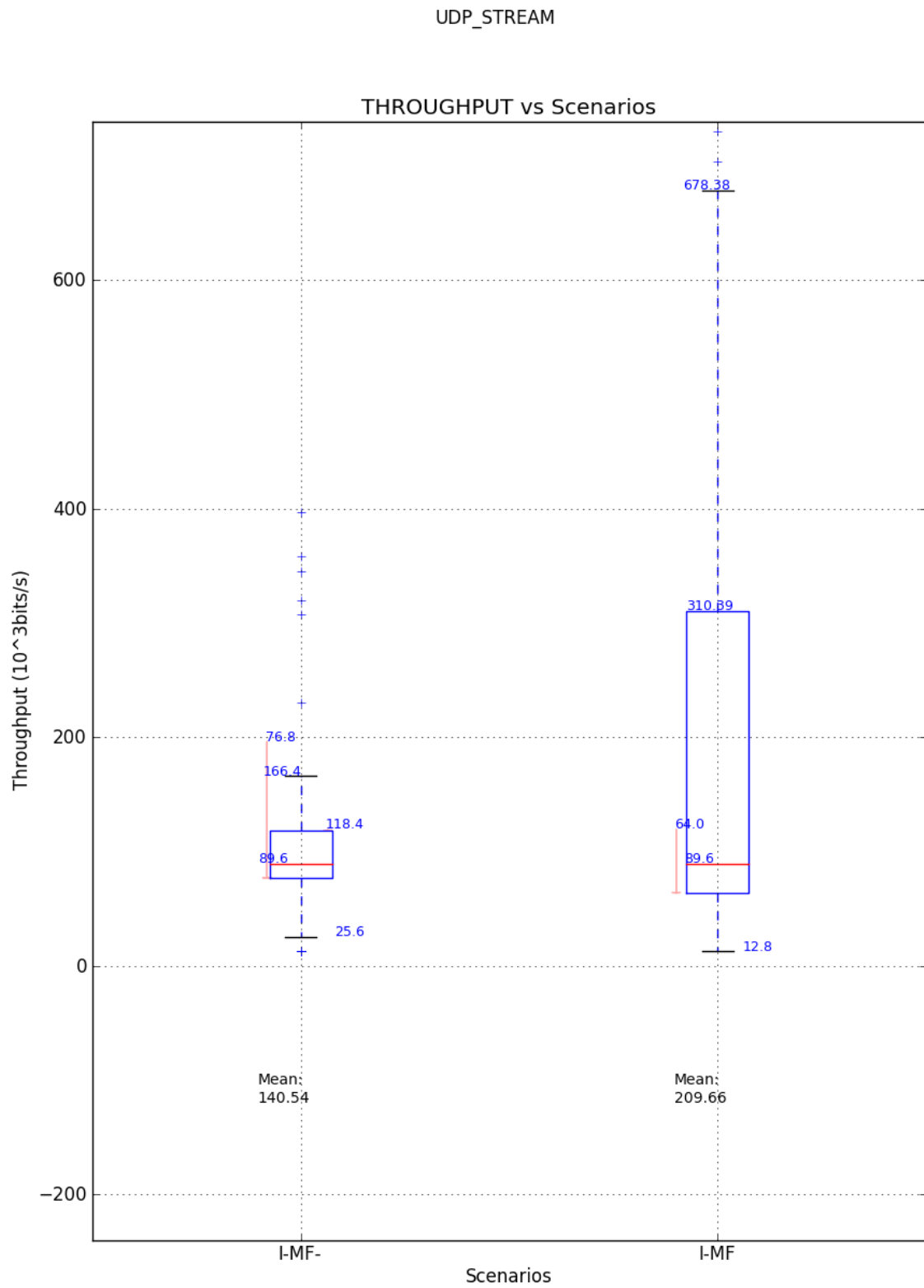
Figure F.4: Boxplots comparison of APS and TPS on different servers using UDP_STREAM Tests
