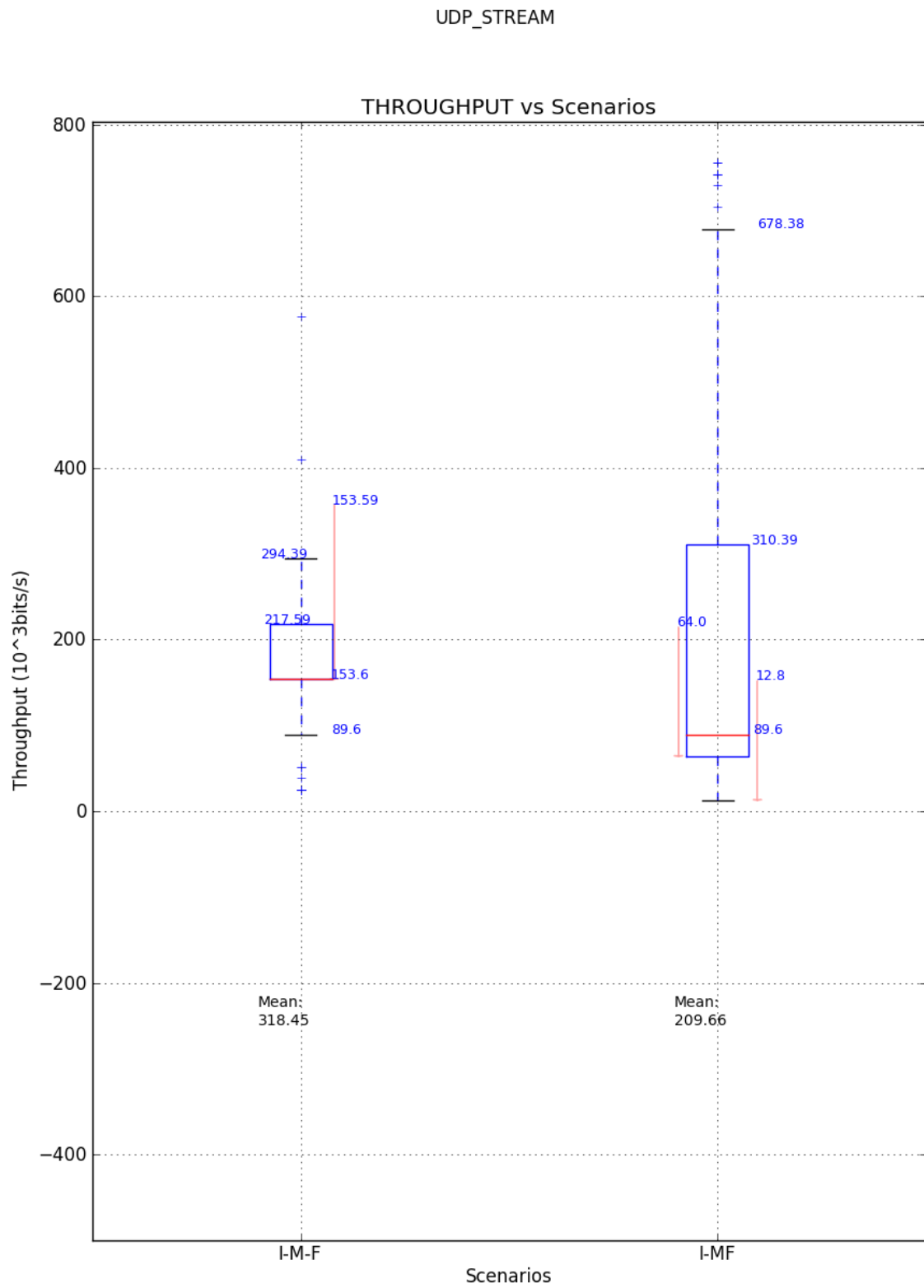
Figure E.19: Boxplots comparison of the performance of IPsec using UDP_STREAM Tests
