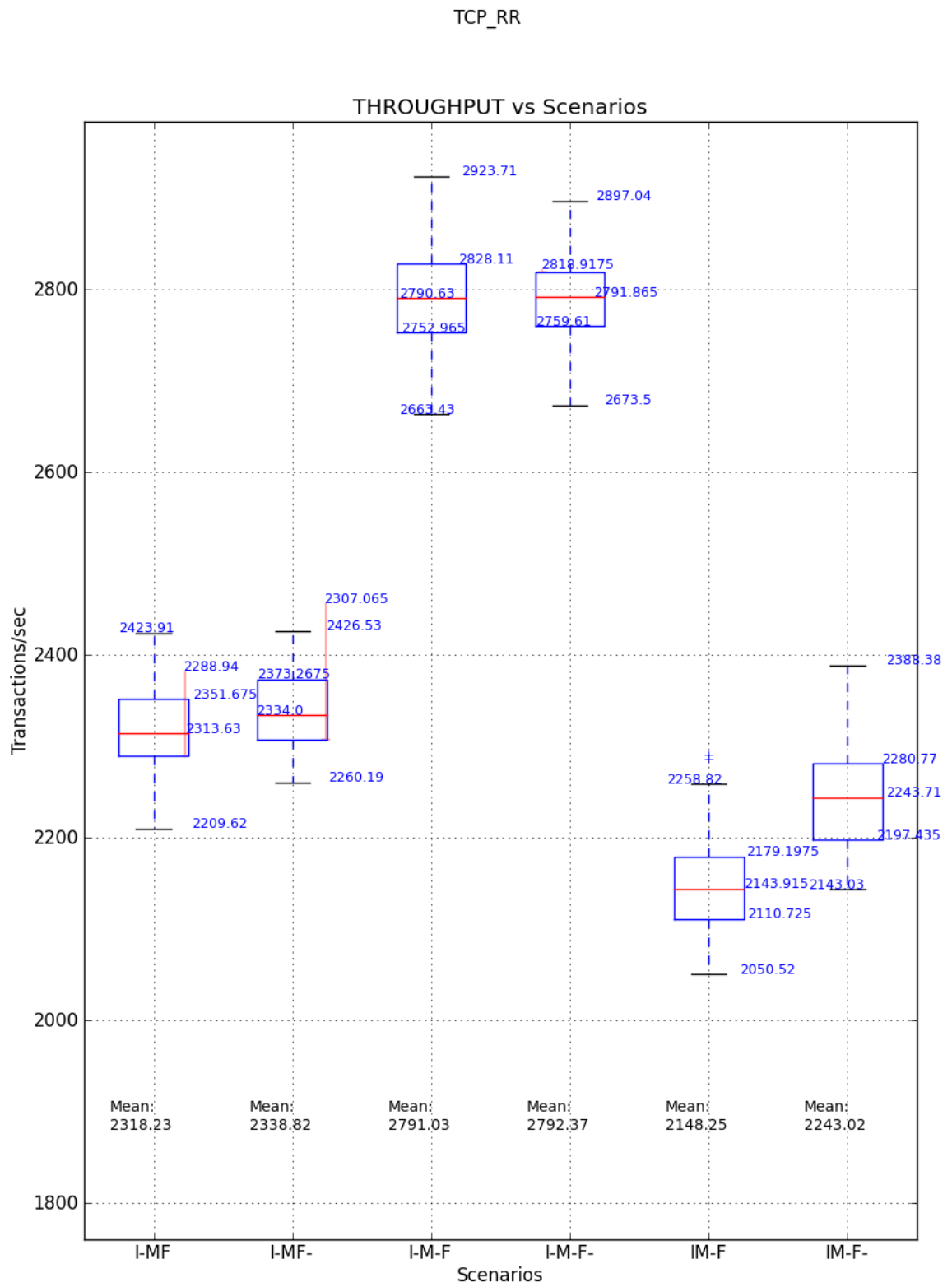
Figure 5.3: Boxplot showing the summary of TCP_RR request and response performance for the six setups
