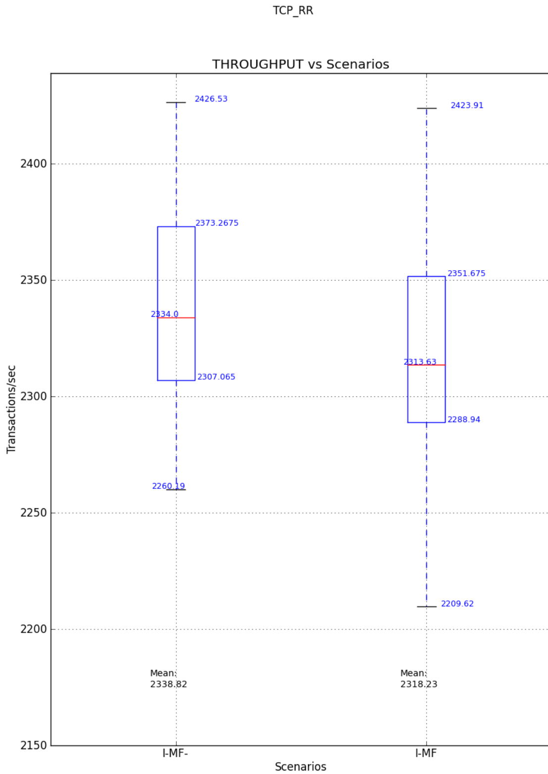
Figure F.13: Boxplots comparison of APS and TPS on different servers using TCP_RR Tests
