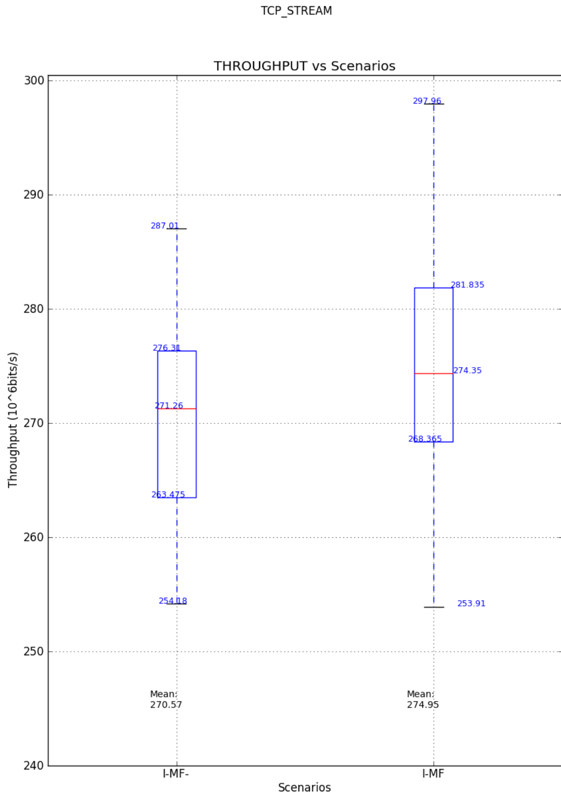
Figure F.1: Boxplots comparison of APS and TPS on different servers using TCP_STREAM Tests
