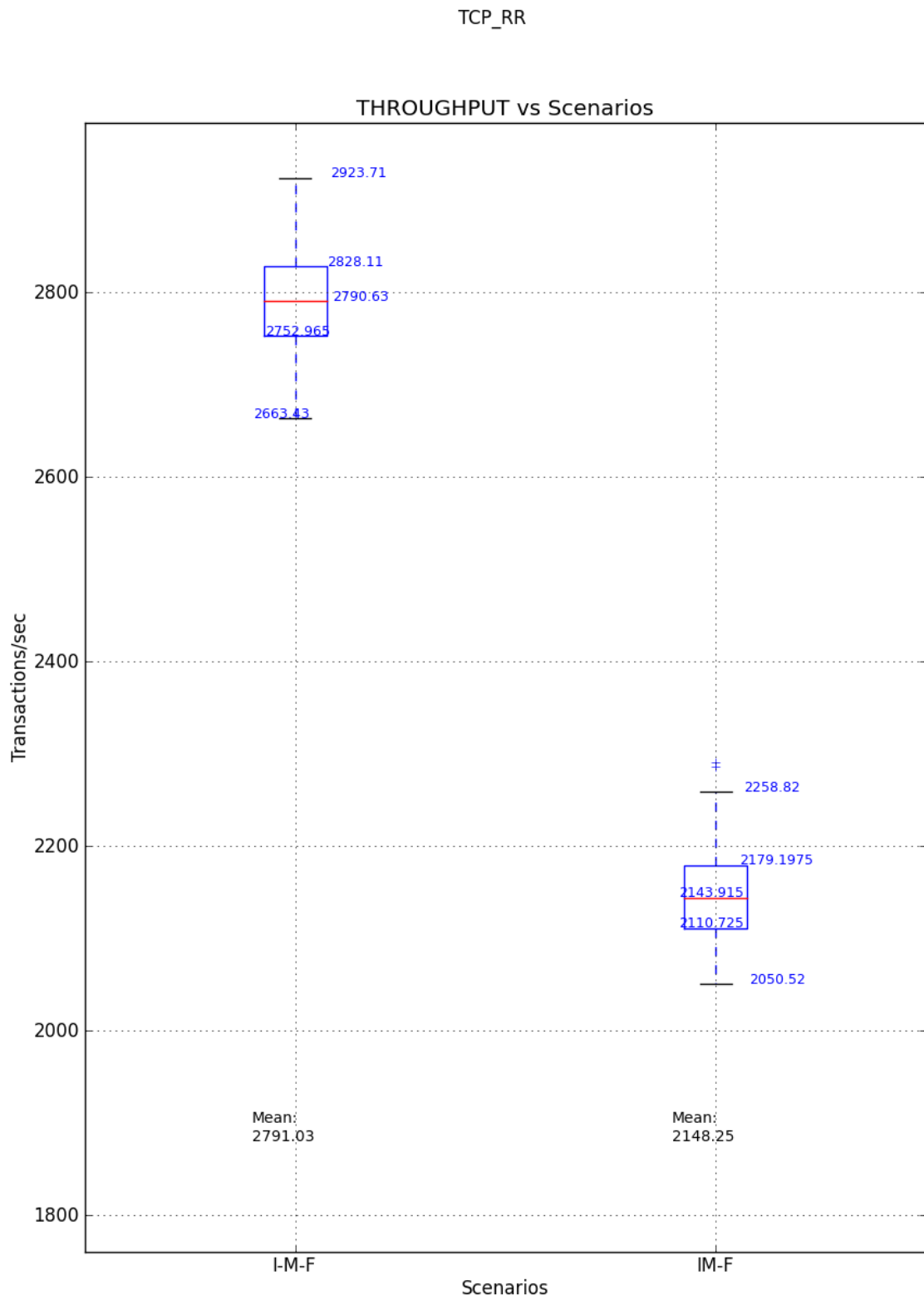
Figure D.28: Boxplots comparison of the performance of IPSec using TCP_RR Tests
