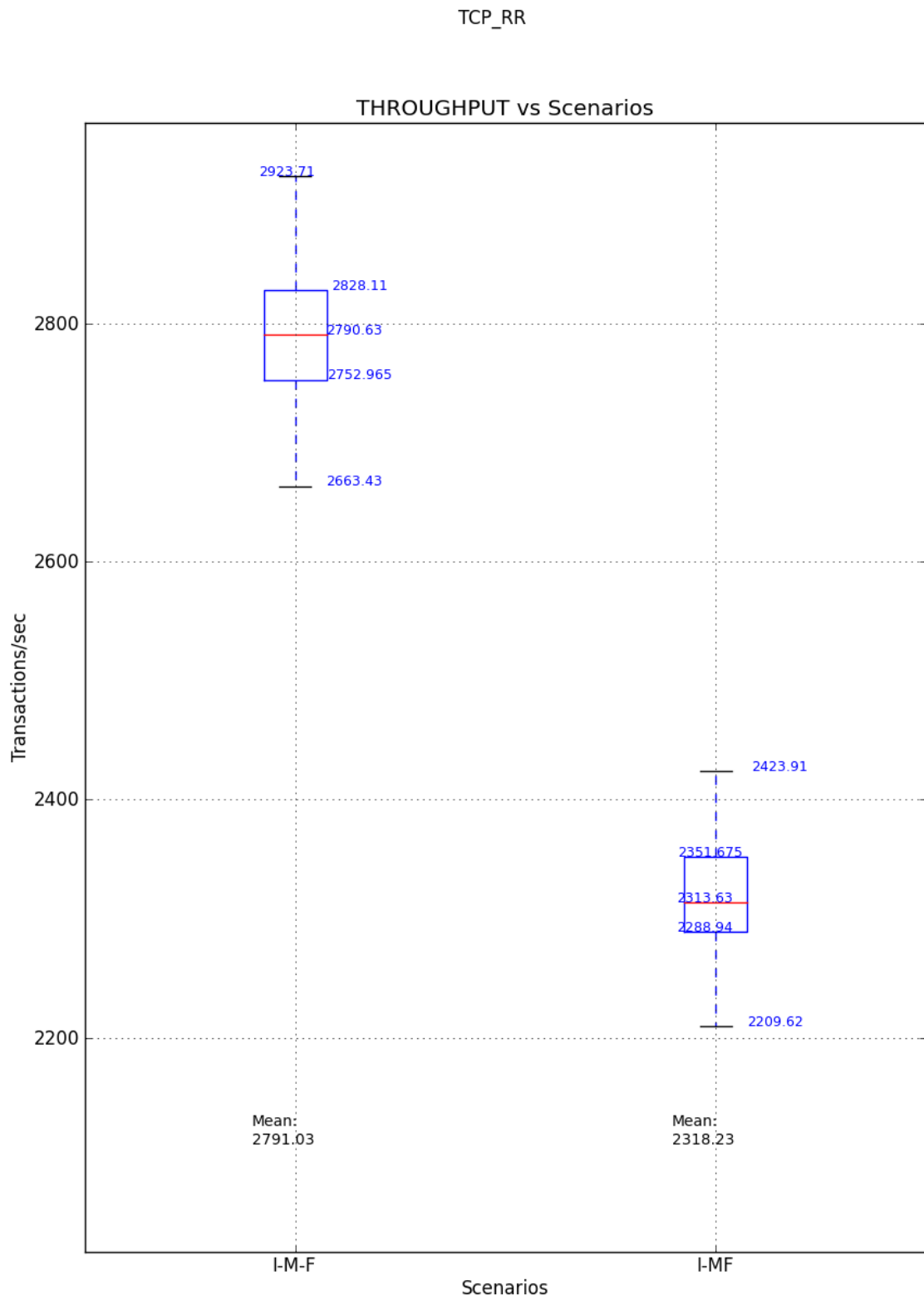
Figure E.28: Boxplots comparison of the performance of IPsec using TCP_RR Tests
