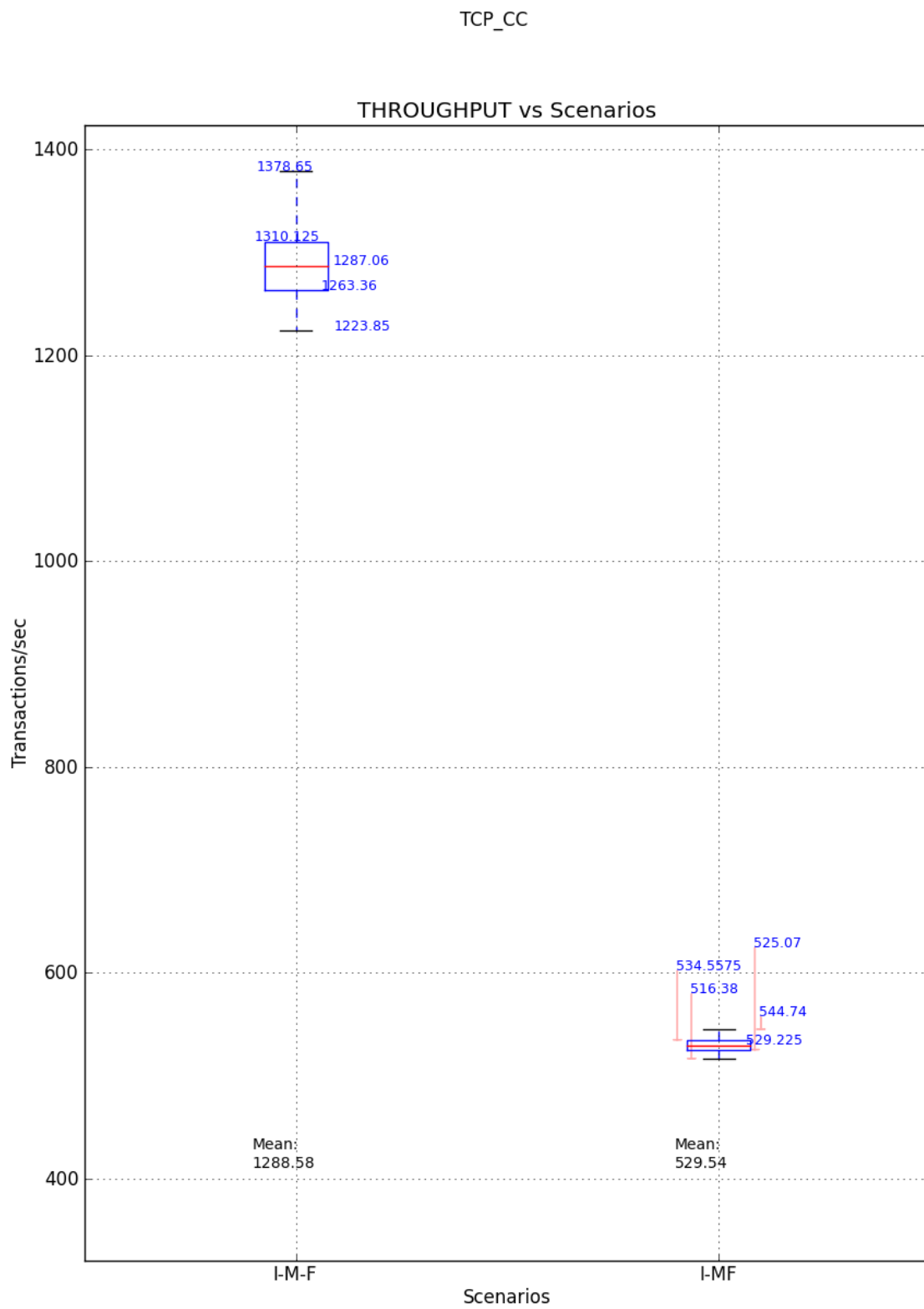
Figure E.22: Boxplots comparison of the performance of IPsec using TCP_CC Tests
