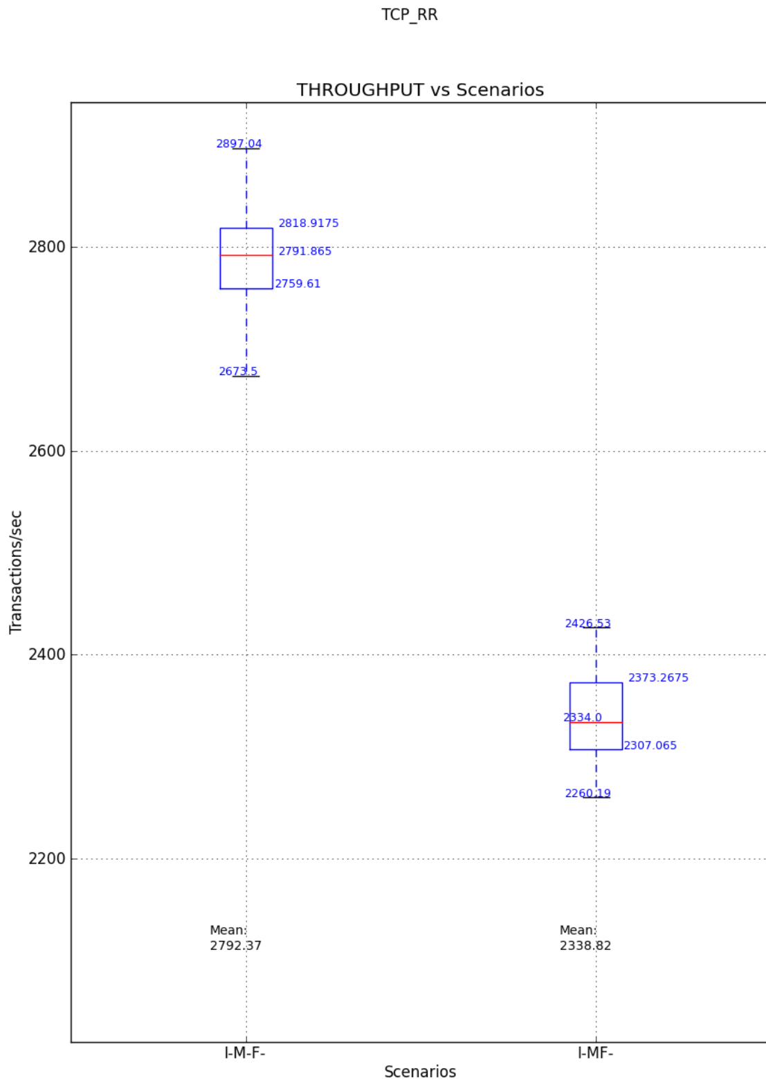
Figure E.13: Boxplots comparison of the performance of IPSec using TCP_RR Tests
