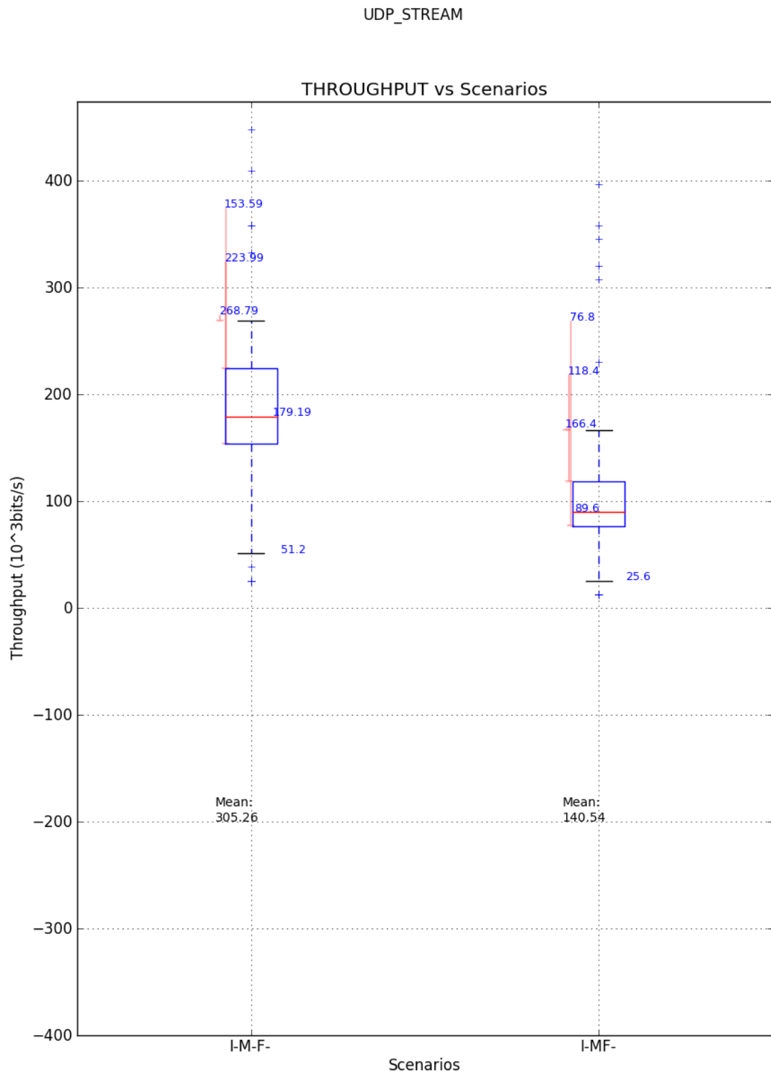
Figure E.4: Boxplots comparison of the performance of IPSec using UDP_STREAM Tests
