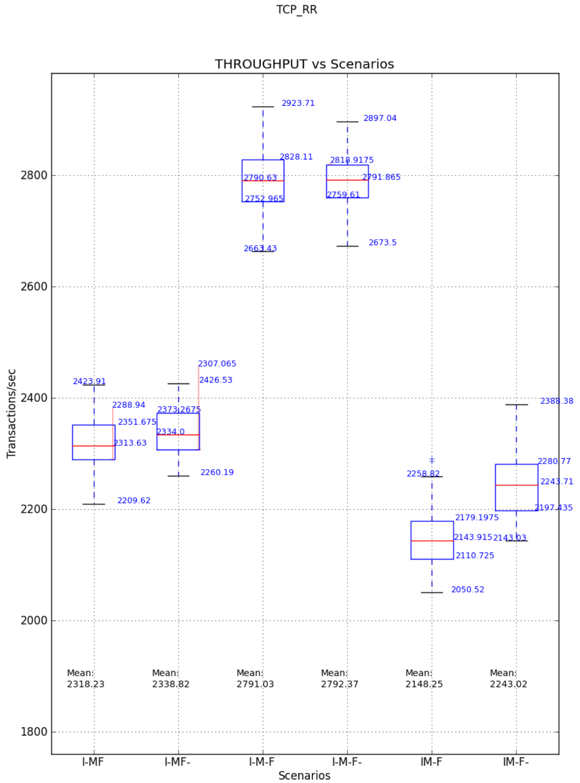
Figure C.5: Boxplots of TCP_RR Tests of all scenarios
