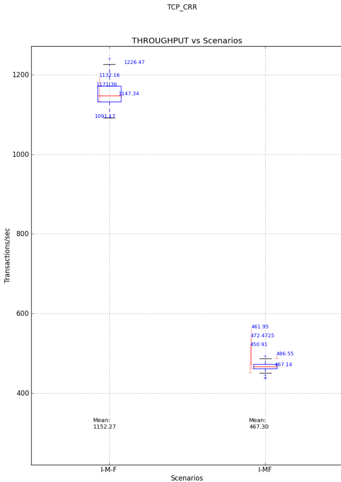
Figure E.25: Boxplots comparison of the performance of IPsec using TCP_CRR Tests
