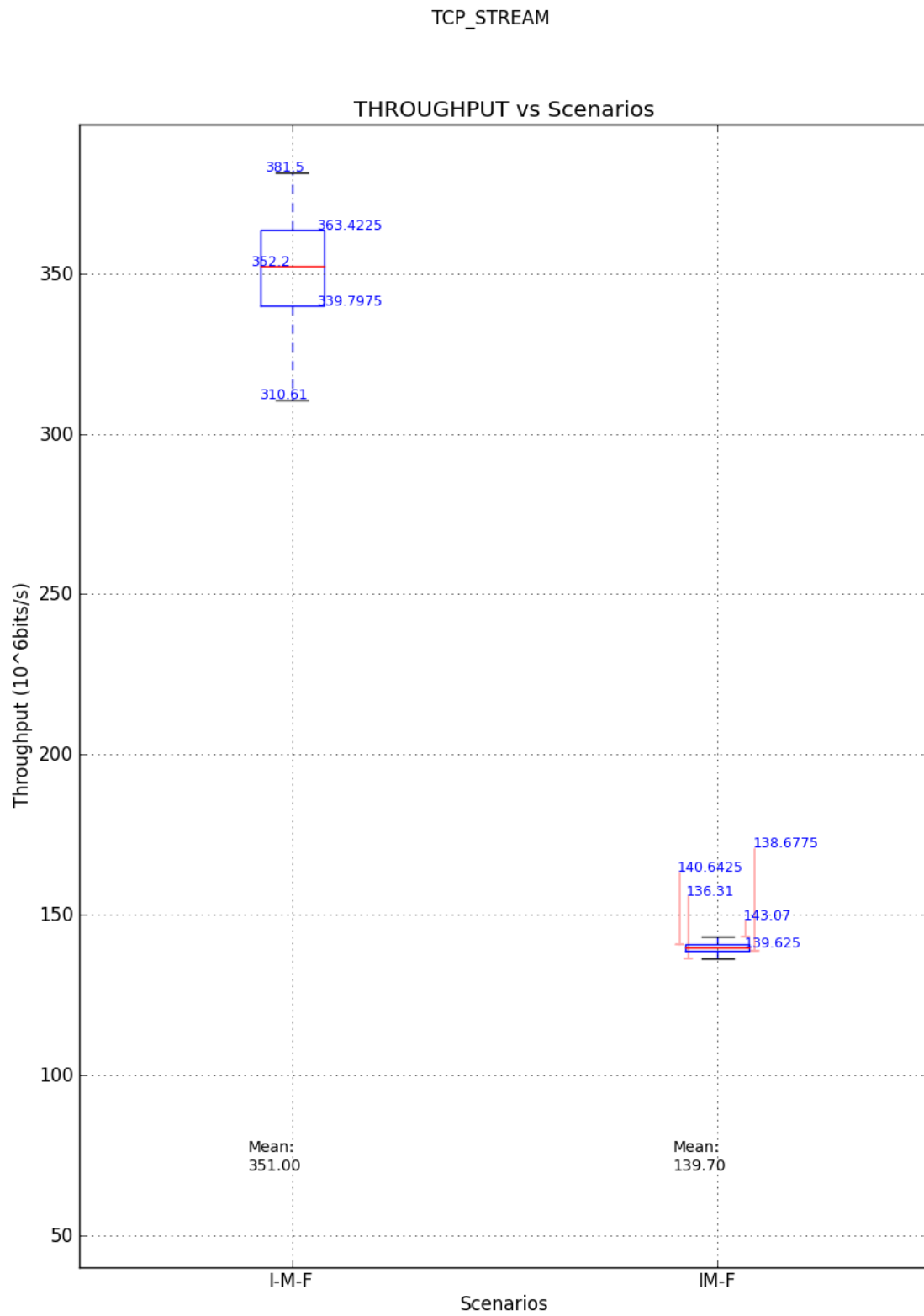
Figure D.16: Boxplots comparison of IPSec using TCP_STREAM Tests
