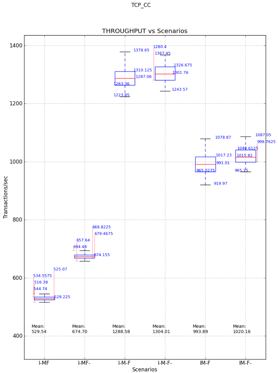
Figure C.3: Boxplots of TCP_CC Tests of all scenarios
