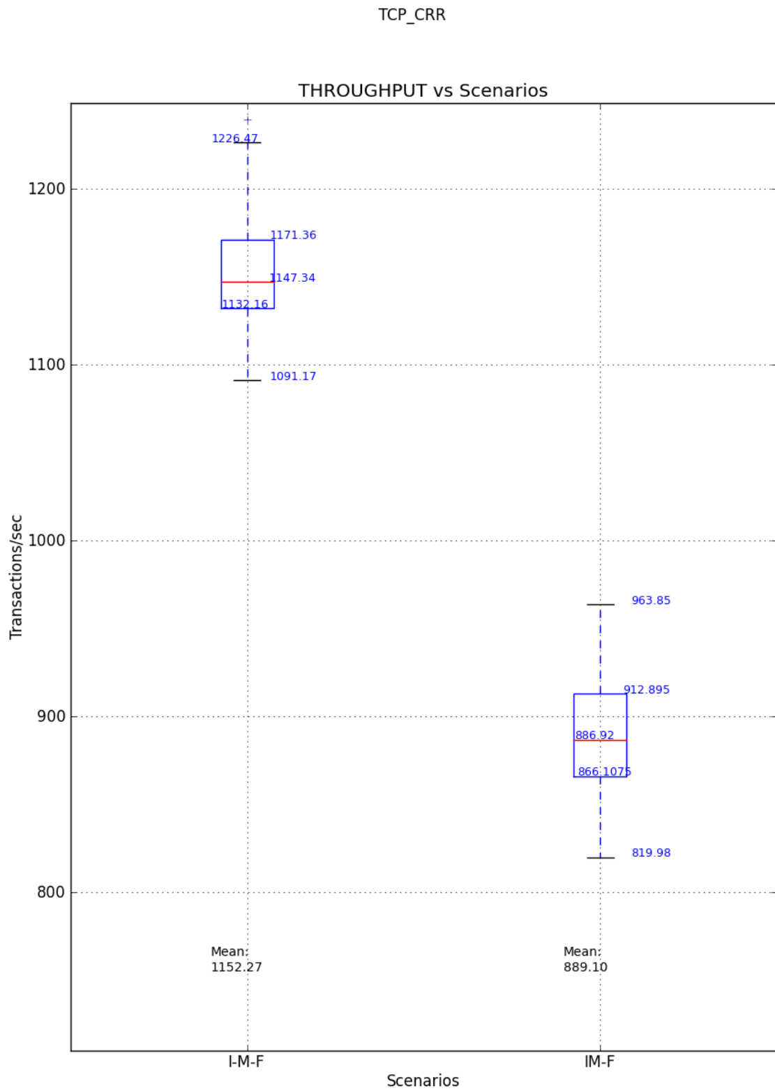
Figure D.25: Boxplots comparison of the performance of IPsec using TCP_CRR Tests
