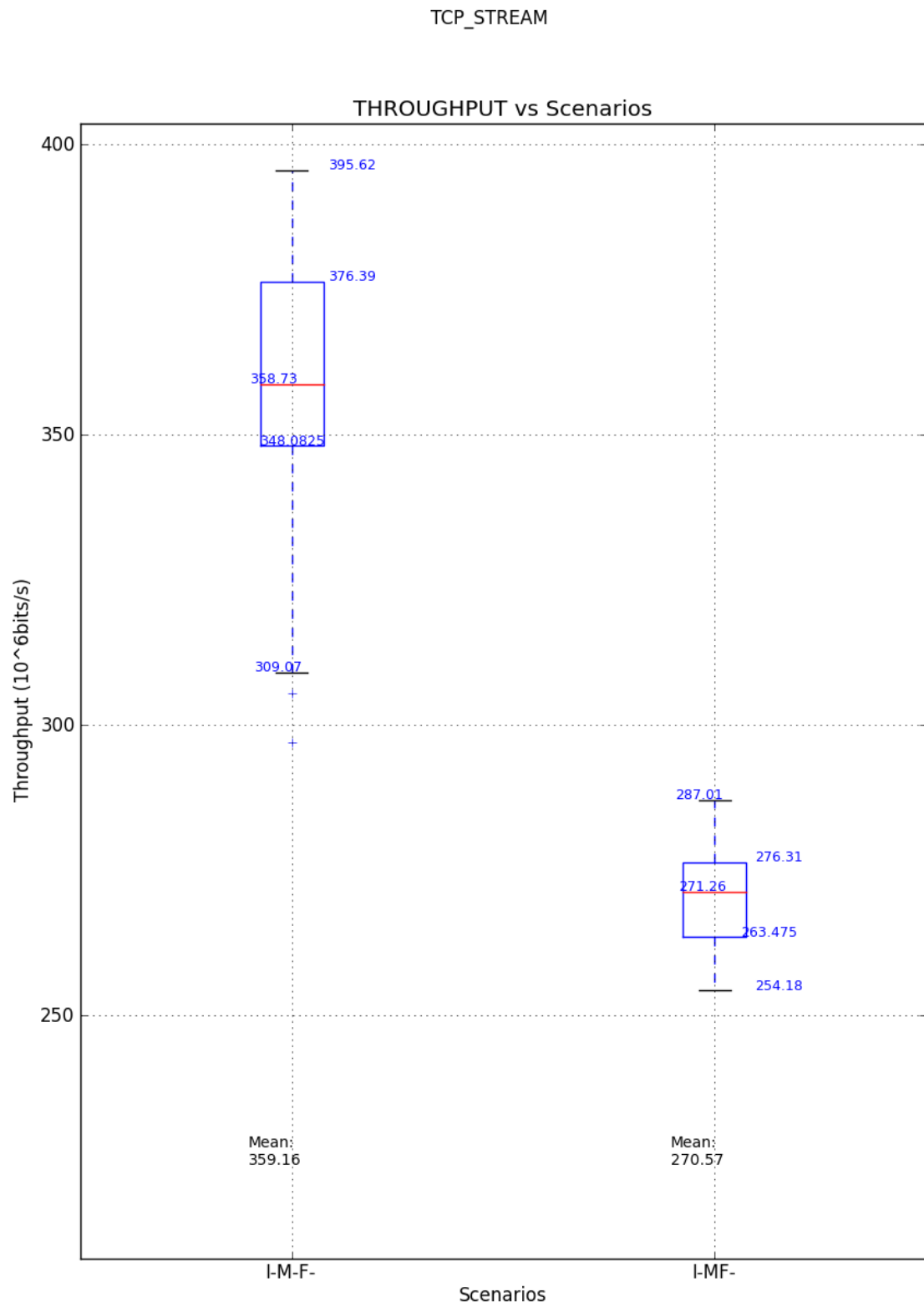
Figure E.1: Boxplots comparison of MYSEA processes using TCP_STREAM Tests
