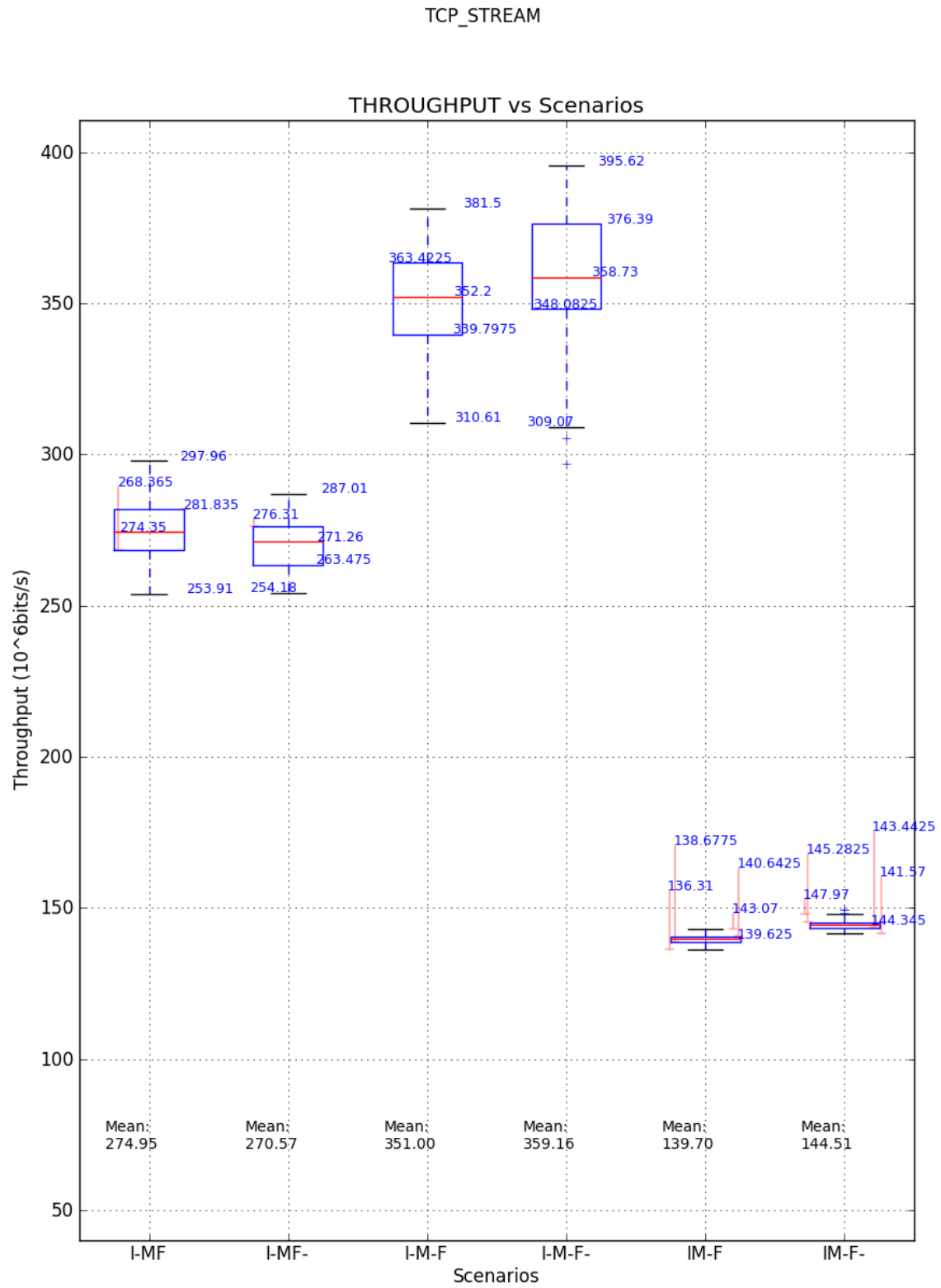
Figure C.1: Boxplots of TCP_STREAM Tests of all scenarios
