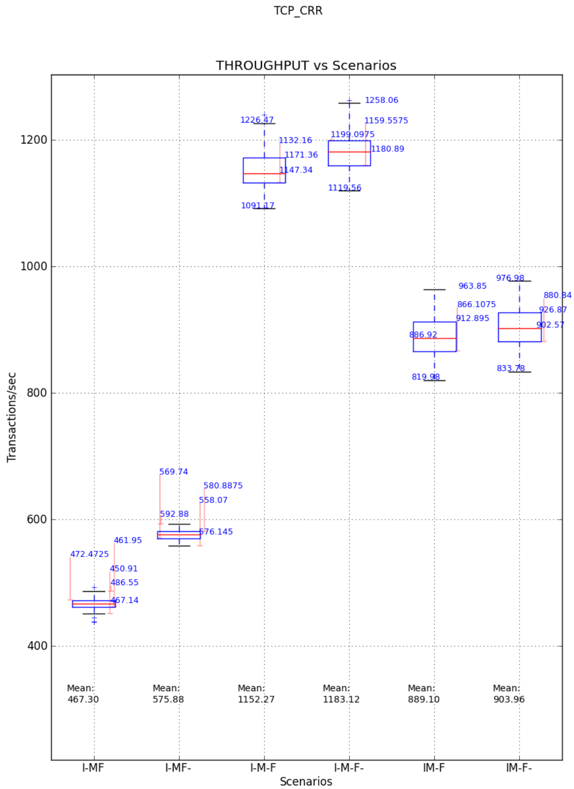
Figure C.4: Boxplots of TCP_CRR Tests of all scenarios
