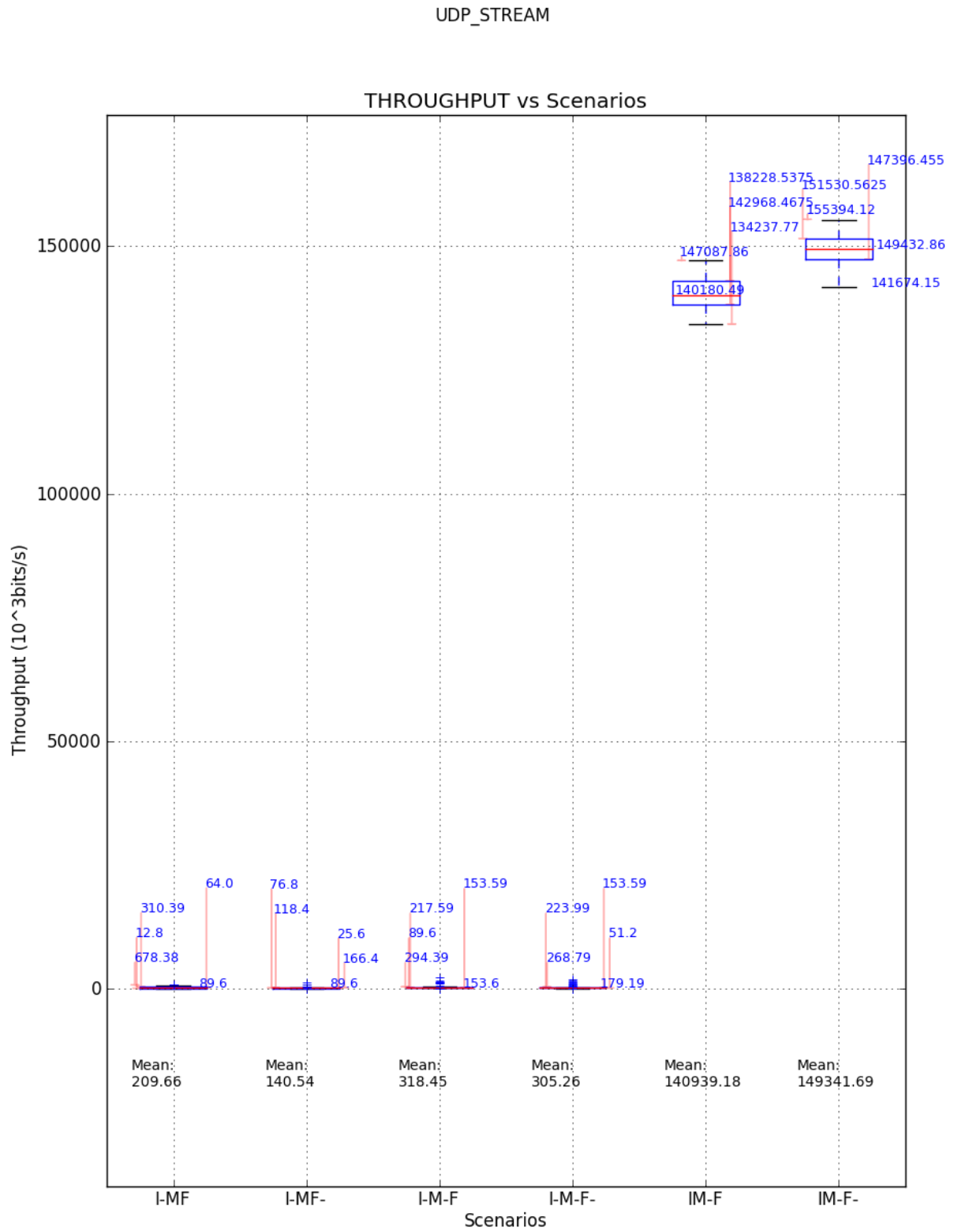
Figure C.2: Boxplots of UDP_STREAM Tests of all scenarios
