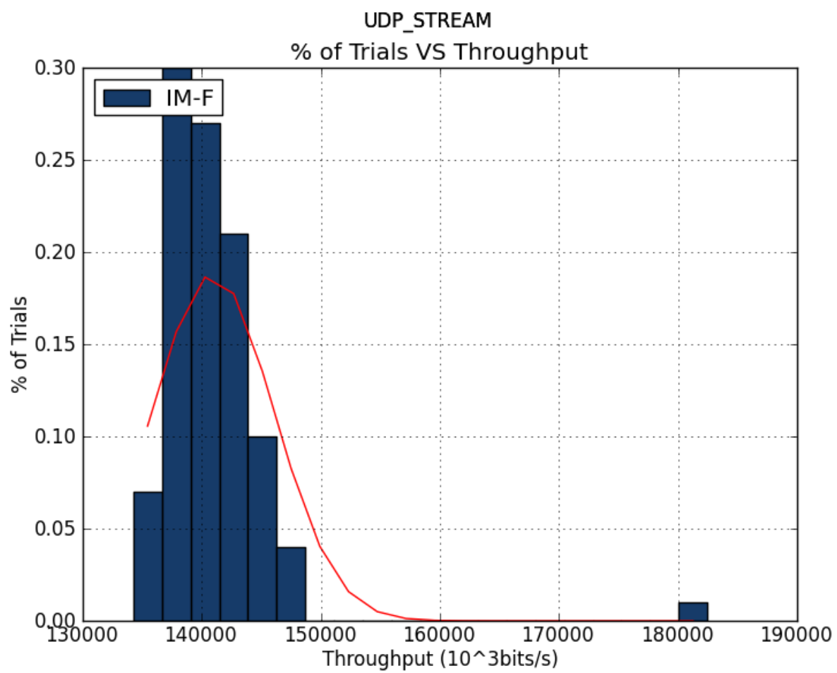
Figure D.20: Histogram comparison of the performance of IPSec using UDP_STREAM Tests
