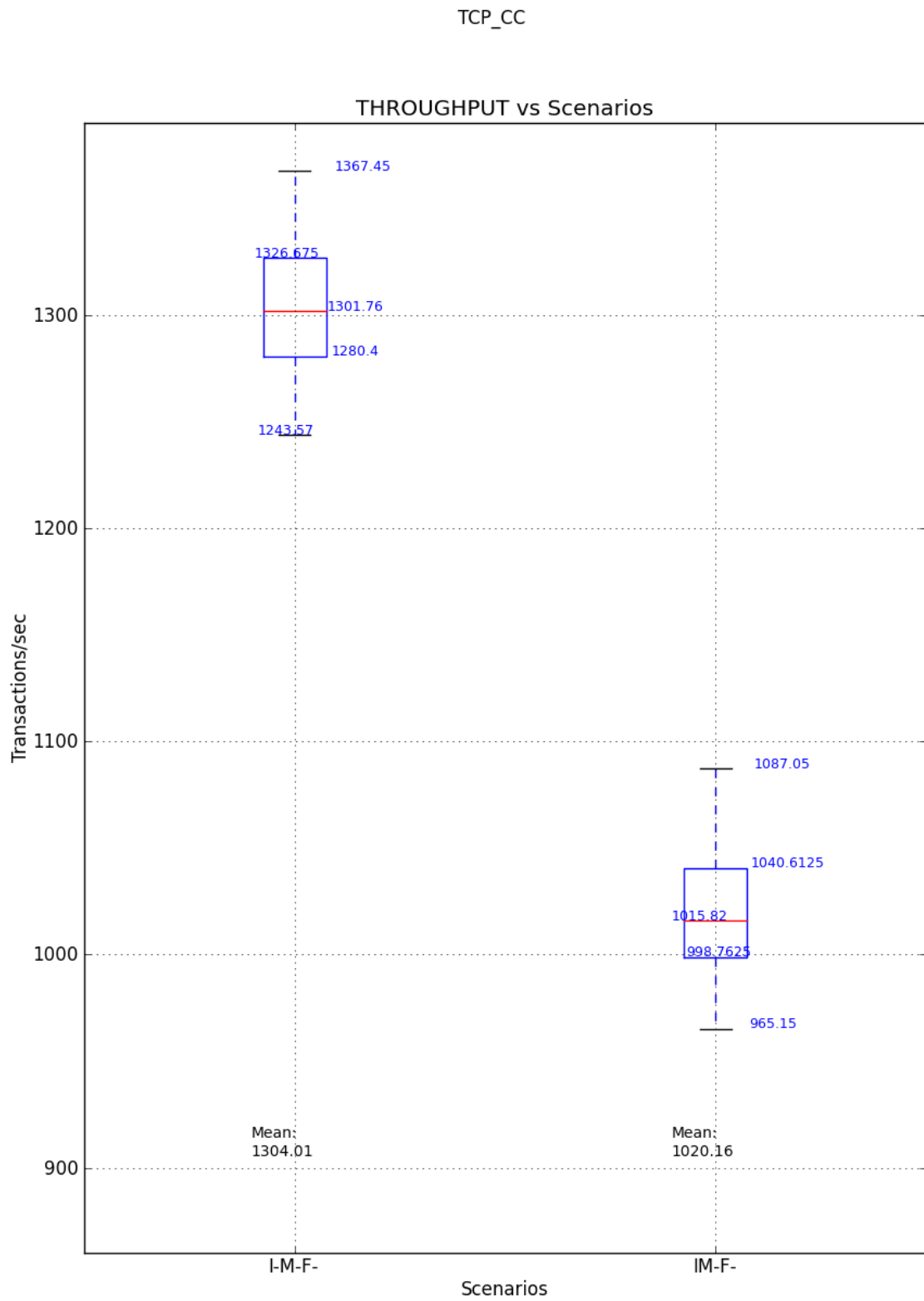
Figure D.7: Boxplots comparison of the performance of IPsec using TCP_CC Tests
