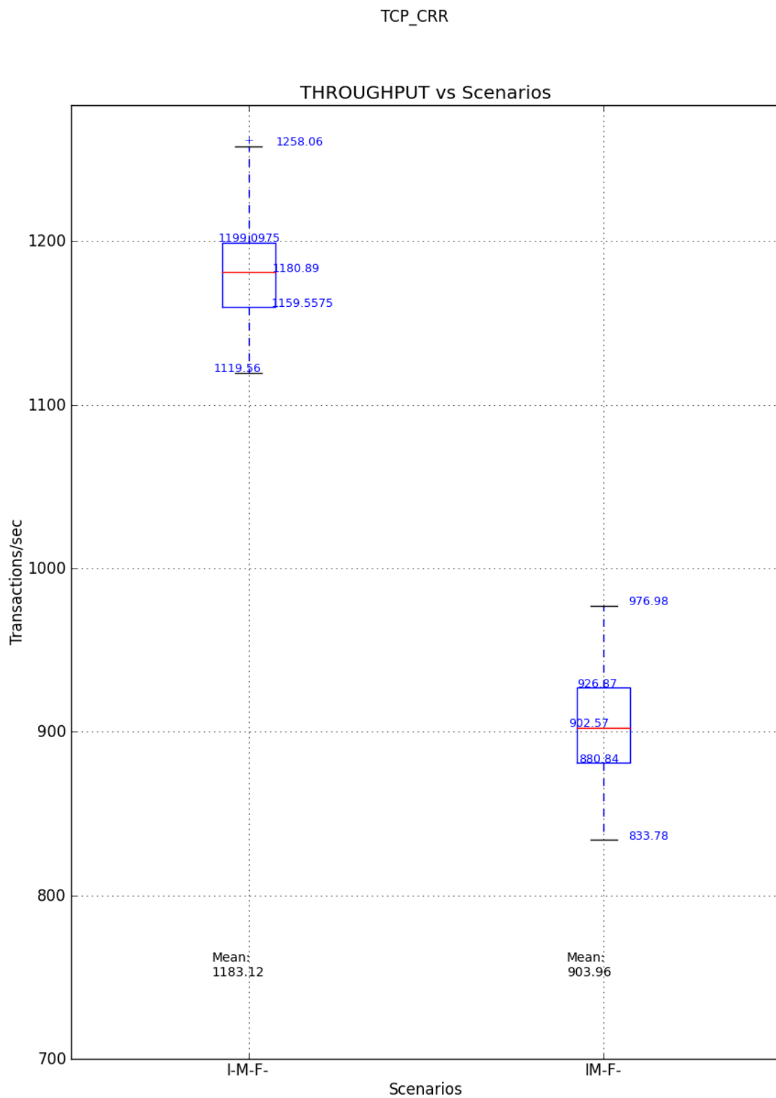
Figure D.10: Boxplots comparison of the performance of IPsec using TCP_CRR Tests
