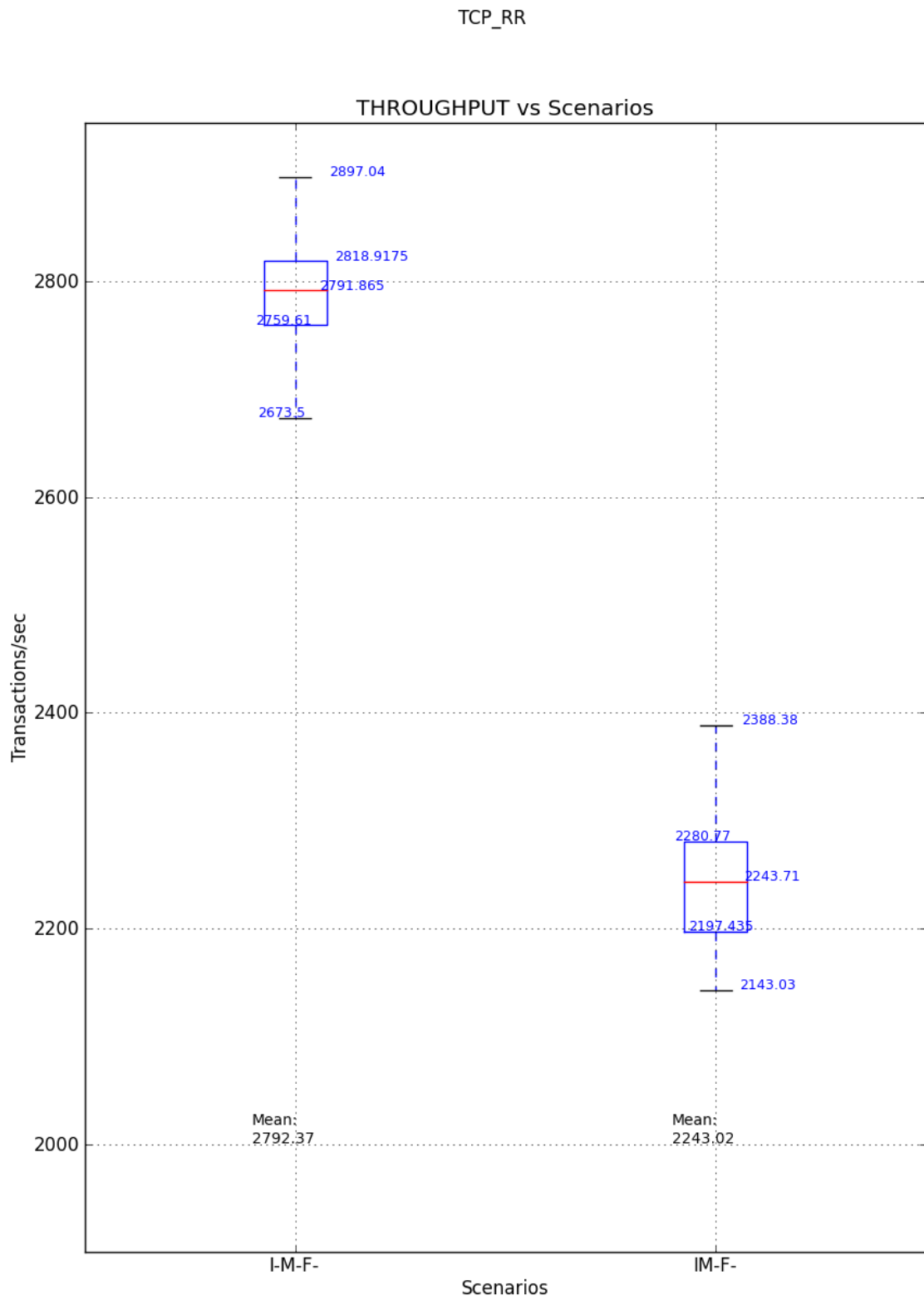
Figure D.13: Boxplots comparison of the performance of IPSec using TCP_RR Tests
