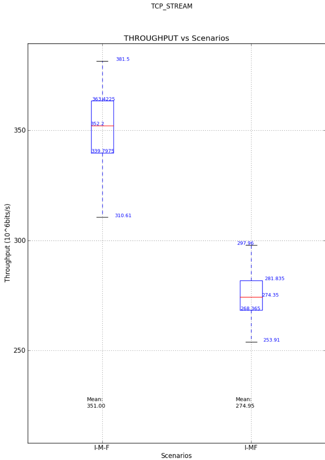
Figure E.16: Boxplots comparison of MYSEA processes using TCP_STREAM Tests
