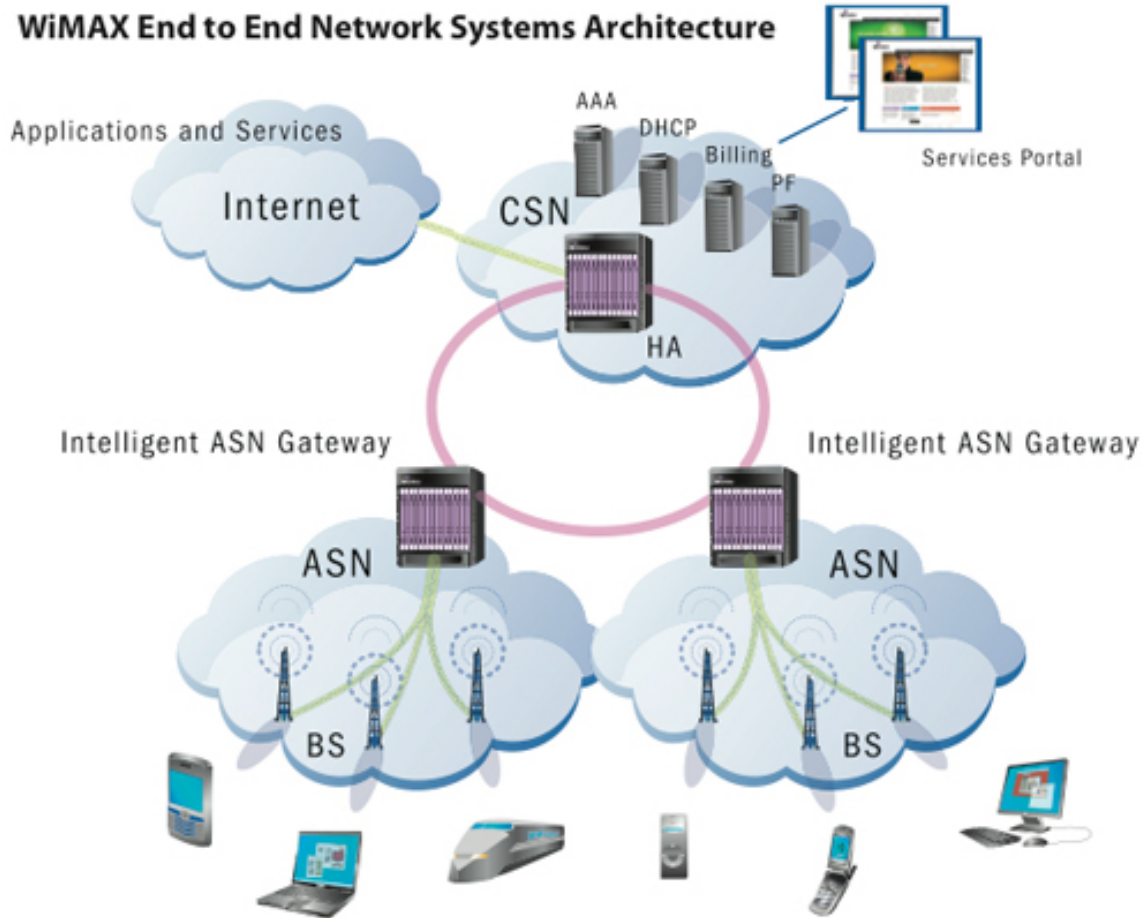
Figure 1. WiMAX architecture [From 2]
