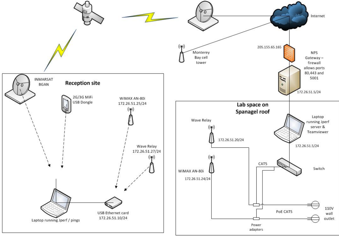
Figure 20. Experiment architecture
