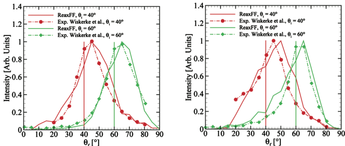
(a) (b) Figure 8 – Scattering angles for O 2 collisions with Pt(111) at incident angles of 40° (red) and 60° (green). ReaxFF predictions compared to experimental measurements for two incident energies: 0.46 eV (a) and 1.73 eV (b).
