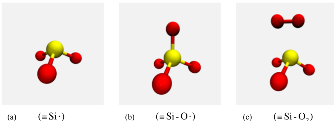
Figure 13 – Defects observed on annealed amorphous \text{SiO}_2 surfaces exposed to dissociated oxygen.
