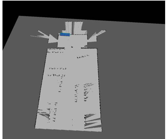
Fig. 1. Occupancy grid map with detected and modeled stairway superimposed (upper left).
