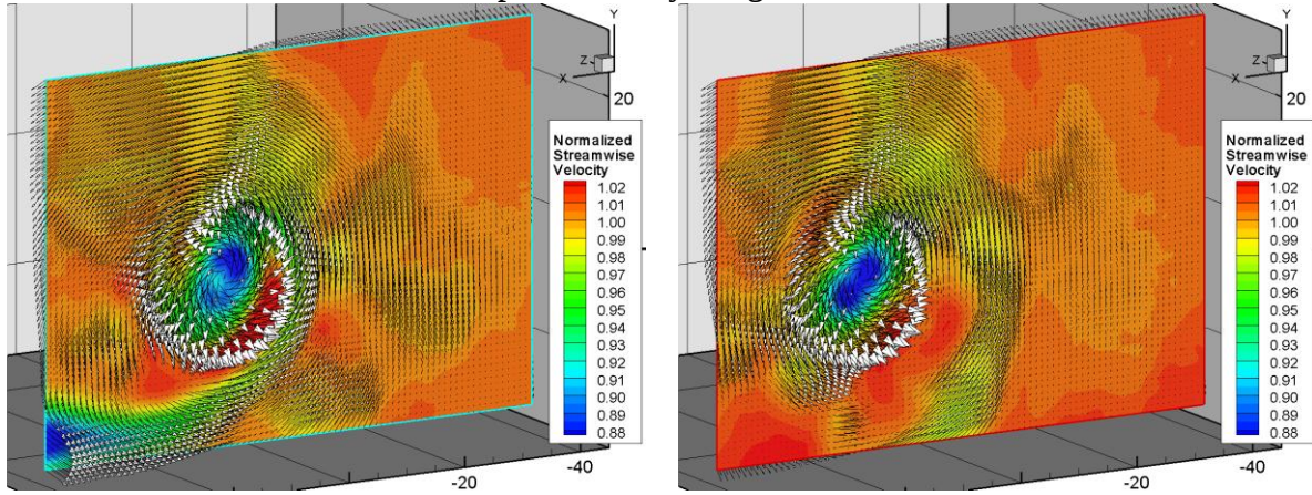
(a). 1.0 chord length downstream
