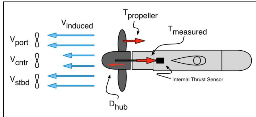
Figure 21: Thrust Data Sign Convention (all quantities positive as shown)
