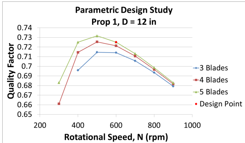
Figure 1: Prop 1 Parametric Design
