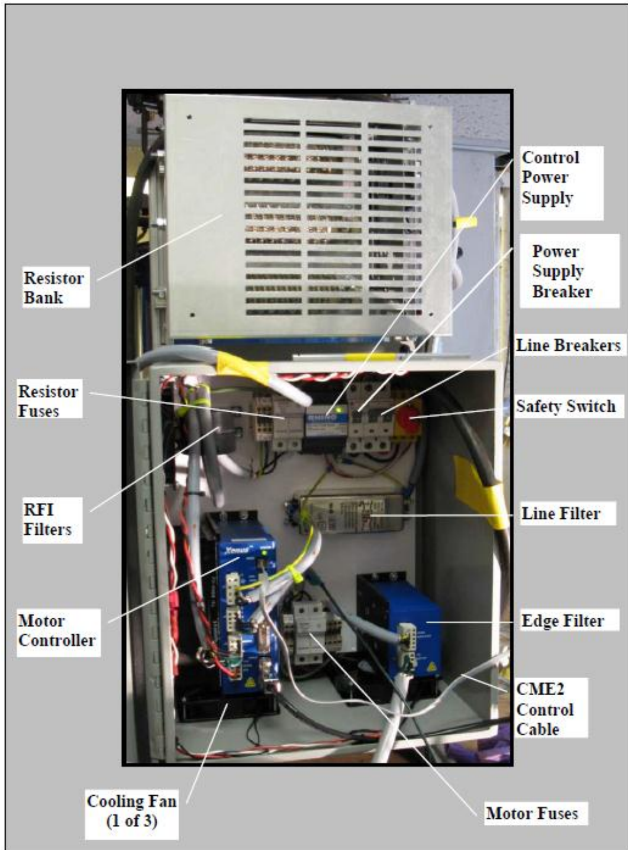
Figure 7: Electrical Components (Courtesy Ketcham)
