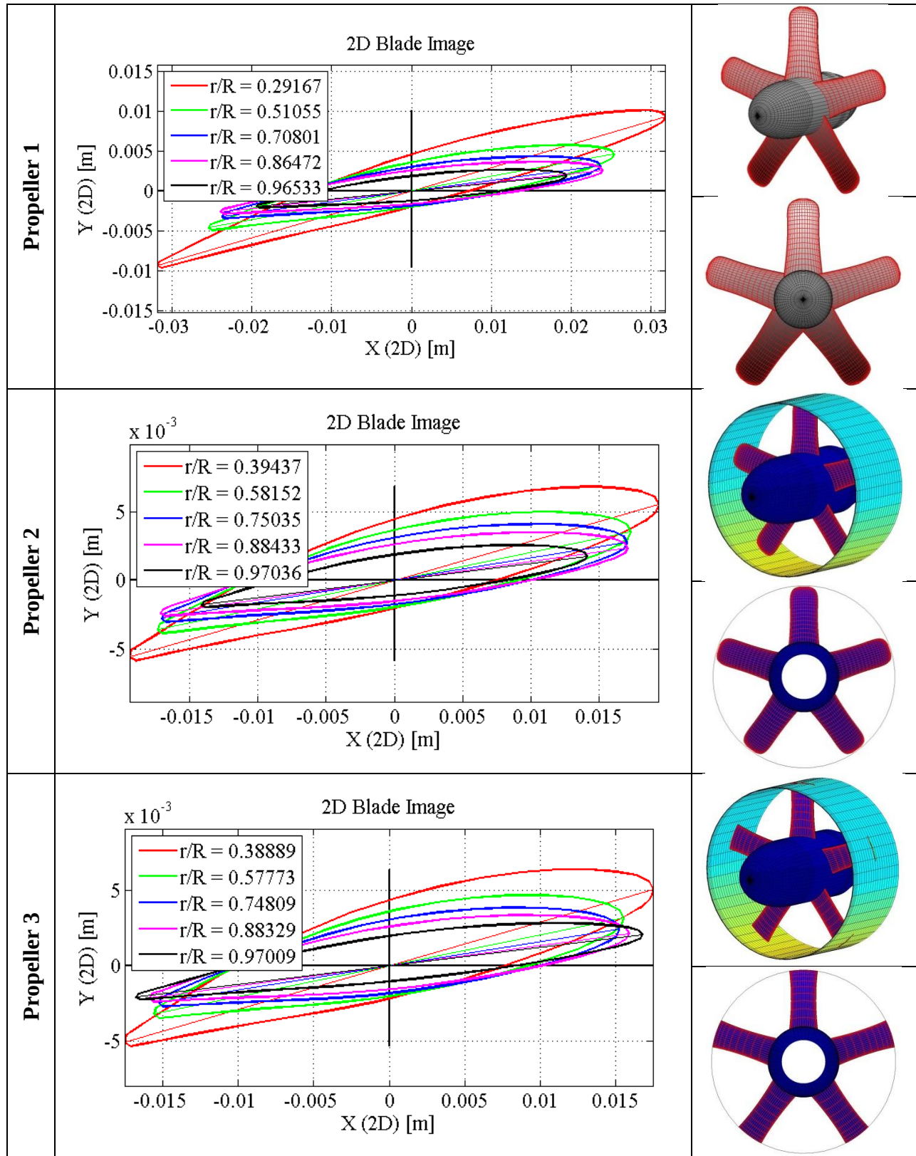
Figure 5: Propeller 2D and 3D Images
