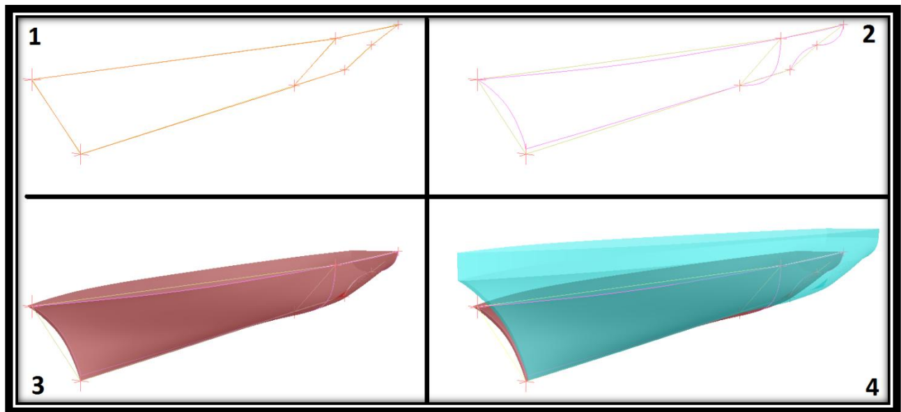
Figure 31: Illustration of Quick Hull Process
