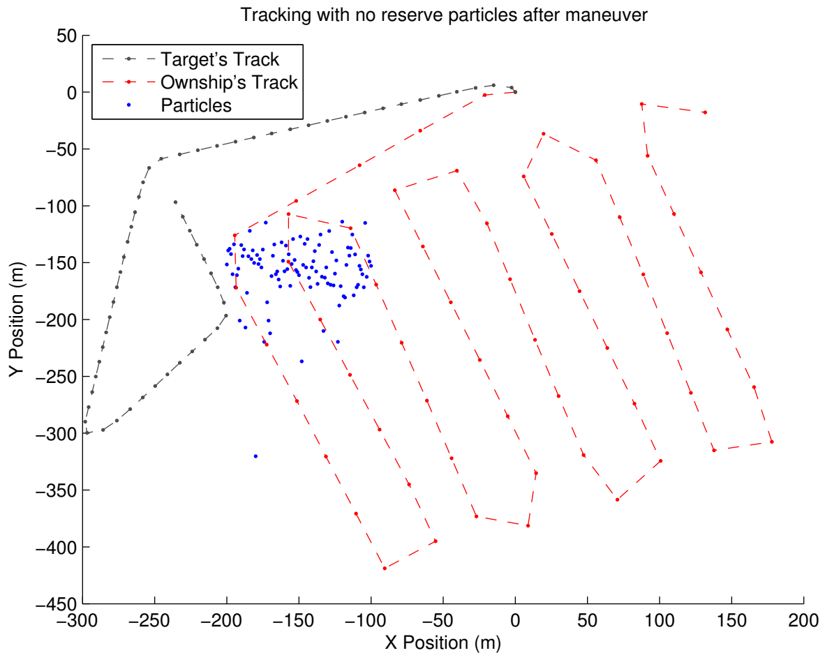
Figure 2-7: Momentum of Particles: As the target maneuvers, the particles are slow to regain the target's track. The particles initial continue on the previously projected track, the outliers close to the contact slowly gain weight and eventual resampling occurs to shift the particles closer to the actually track. If the particles deviated too far from the track they may not reconverge on the contact and instead converge on track with a parallel solution.
