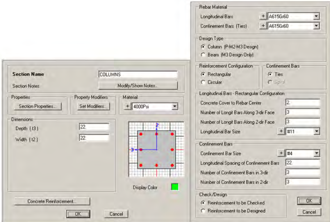
Figure 6: Column details
