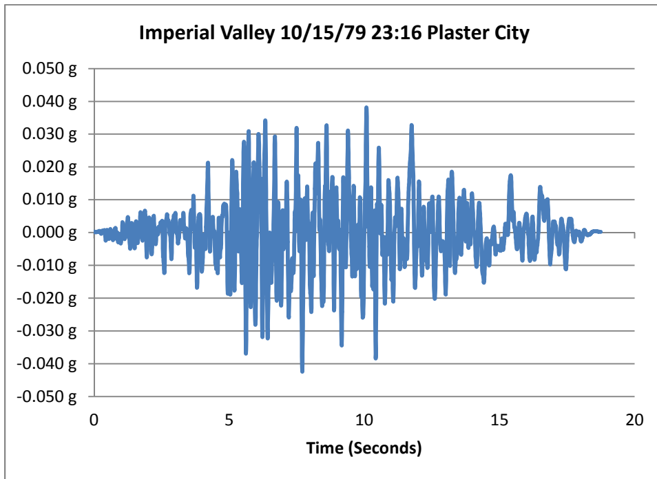
Figure 31: Time history for Imperial Valley 10/15/79 23:16 Plaster City earthquake
