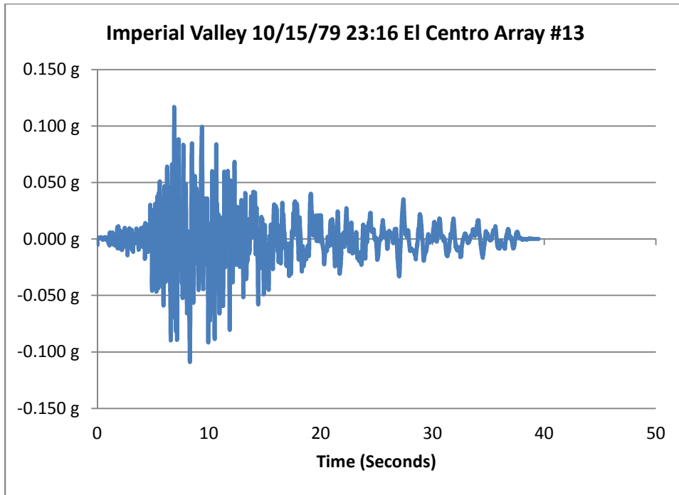
Figure 30: Time history for Imperial Valley 10/15/79 23:16 El Centro Array #13 earthquake
