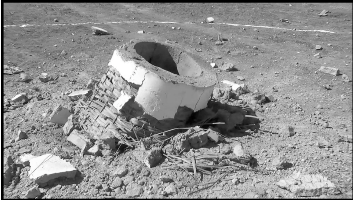
Figure 45. Successful bamboo reinforced ERW-CP field test photo series
