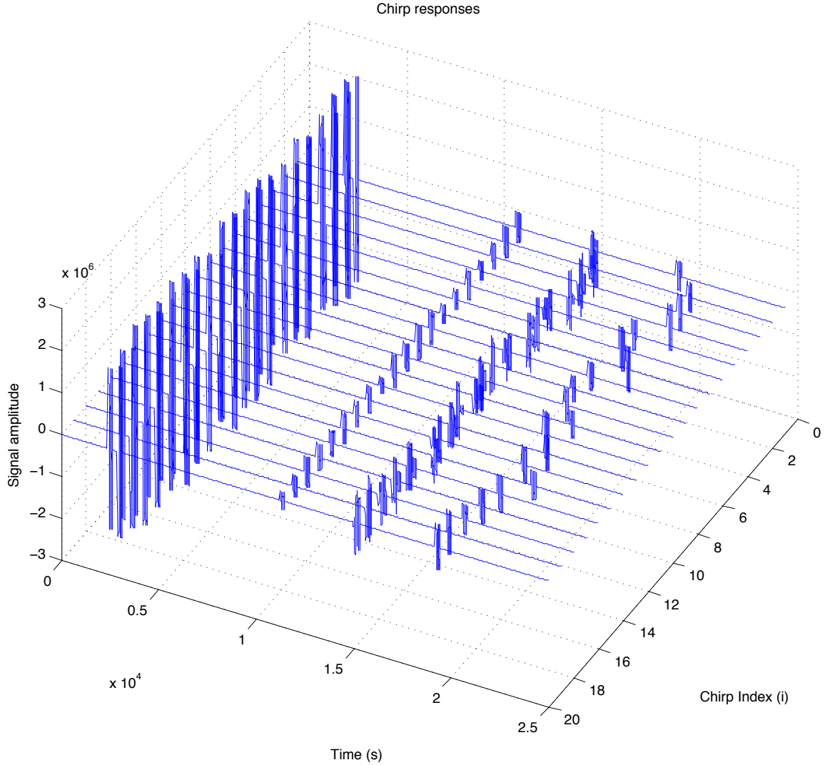
Figure 13. Ensemble of 20 chirp responses with no clock skew.
