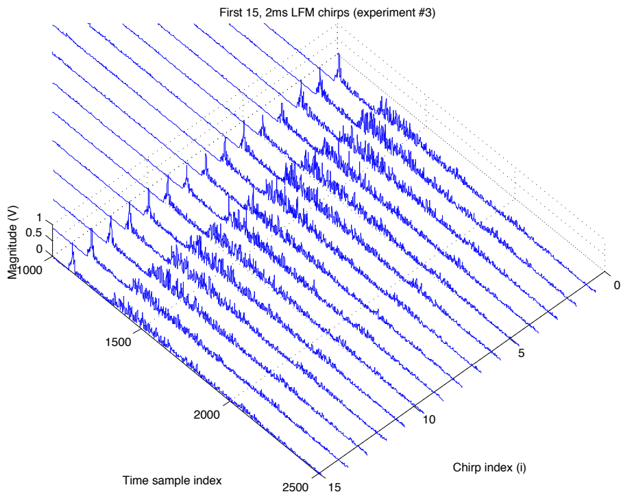
Figure 30. First fifteen 2 ms long LFM chirp responses at 50 m (experiment #3).
