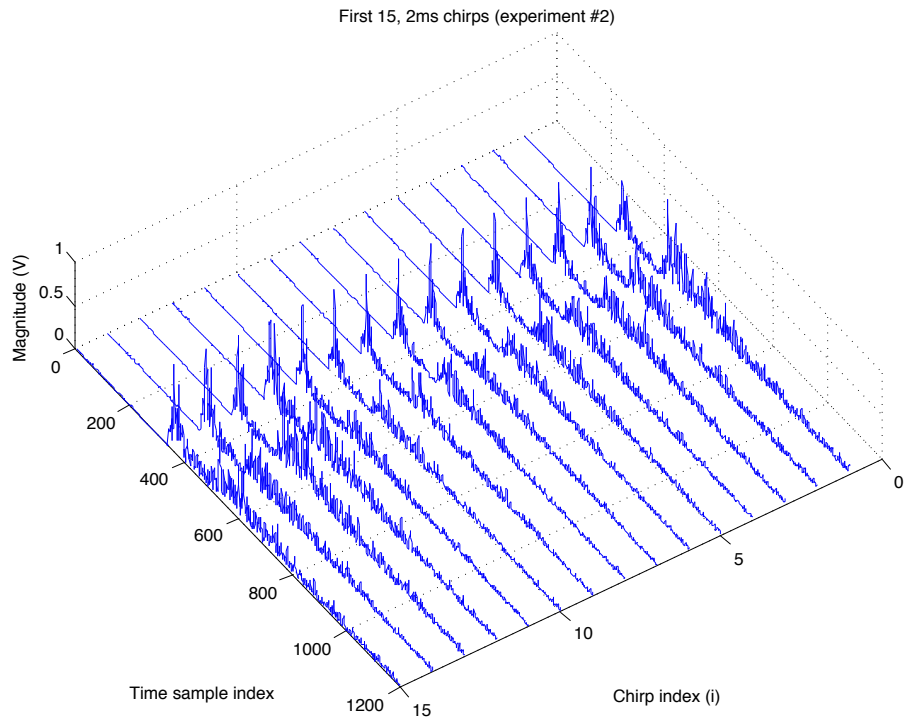
Figure 29. First fifteen 2 ms long LFM chirp responses at 2 m (experiment #2).
