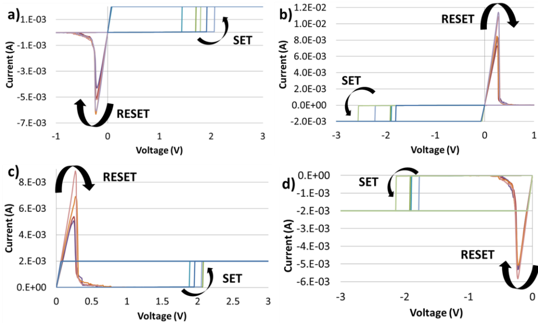
Figure 4.4.3 Complete nonpolar behavior over 4-5x cycles per switching style demonstrated on the same 70x70 μm TE device from the RIE 300 W sample, a) bipolar(+), b) bipolar(-), c) unipolar(+), and d) unipolar(-).
