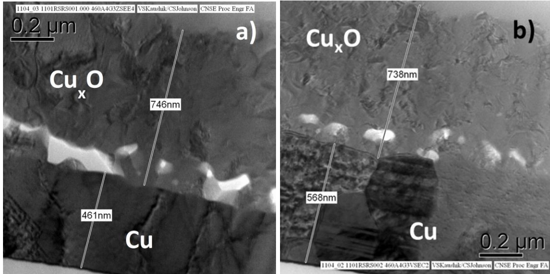
Figure 4.2.4 Significant voiding at the \text{Cu}_x\text{O}/\text{Cu} interface from the plasma oxidation process as seen in a) ECD wafer Slot 2 and b) PVD wafer Slot 2
