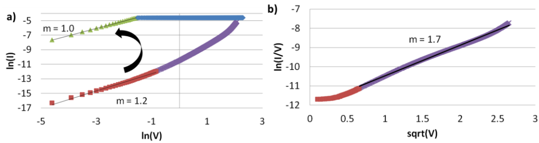
Figure 4.5.5 a) A double log I-V plot of a typical first SET of Cu biased, Al TE grounded device clearly indicated ohmic conduction for the first part of the HRS and the entirety of the LRS. b) Pool-Frenkel emission was indicated after the ohmic conduction for the HRS during the first SET.
