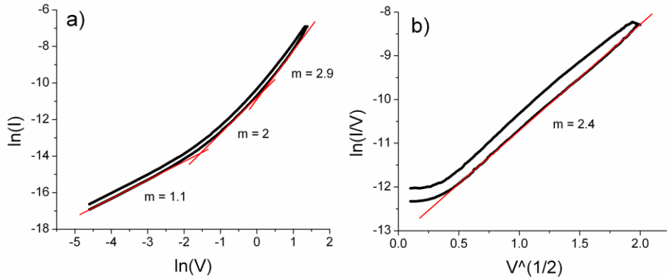
Figure 4.5.3 a) Double-logarithmic I-V plot clearly indicated ohmic conduction at low voltages. SCLC type fits may be imposed on the curve, but the transition points were not well defined. b) Poole-Frenkel emission clearly indicated in the figure.
