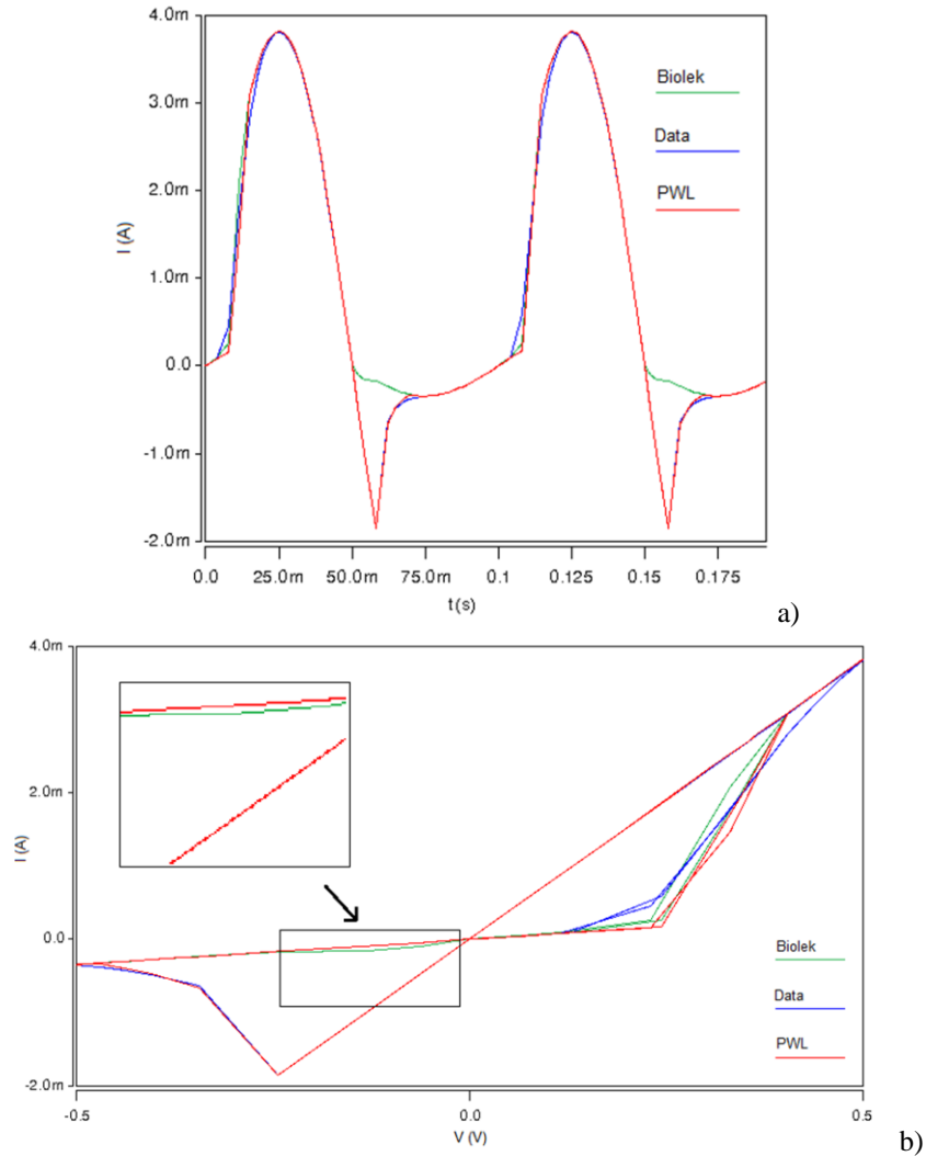
Figure 5.4.1 a) Figure depicts the current response of a chalcogenide memristive device to a 10 Hz signal. b) The model I-V plot derived from the data in a)
