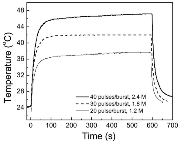
Fig. 2. Temperature increases due to the application of 1.2 M, 1.8 M, and 2.4 M pulses. Here, “M” stands for a million. The pulses were applied in the burst-mode with 20, 30, and 40 pulses/burst. The repetition rate in each burst was 10 kHz and each burst repeated every 10 ms (100 Hz). The exposure time for each of these three exposure conditions was 10 min. The starting temperature was 24^{\circ}\text{C} \pm 1^{\circ}\text{C} .
