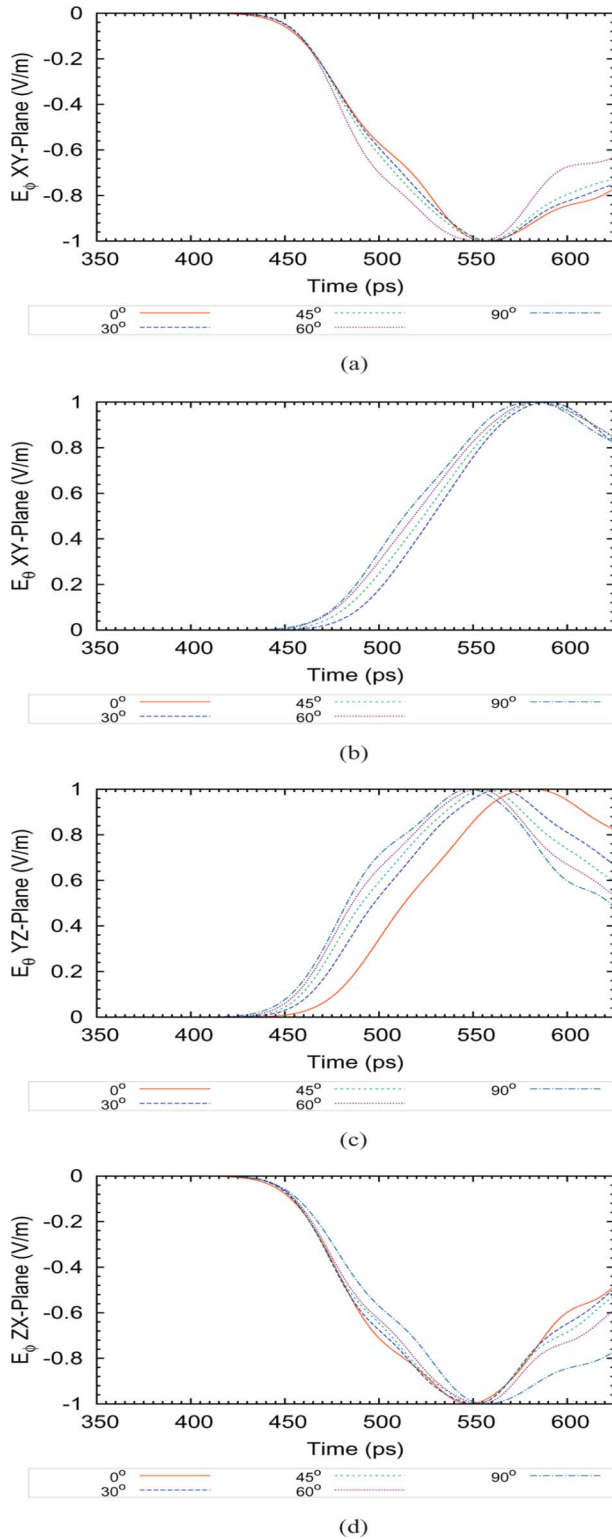
Fig. 12. Normalized E_\theta and E_\phi components of the responses from the electric field probes on the xy -, -yz -, and -zx -planes for the T4FASC-SPV configuration. (a) Normalized E_\phi in the xy -plane (b) Normalized E_\theta in the xy -plane (c) Normalized E_\theta in the -yz -plane (d) Normalized E_\phi in the -zx -plane.
