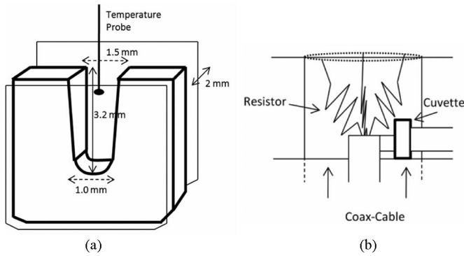
Fig. 1. Subnanosecond exposure system. (a) Cuvette with a loading volume of 6\ \mu\text{L} . The electrodes are 70\text{-}\mu\text{m} -thick stainless steel foils. (b) Cuvette was placed at the end of a coax-cable (RG 217). A conical resistor array was connected in parallel with the cuvette for matching the 50\text{-}\Omega coaxial, subnanosecond pulse delivery cable.
