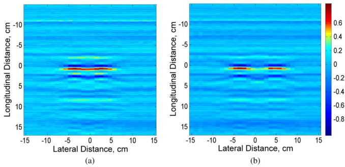
Fig. 7. Images of two identical metallic objects ( 2.5 \times 1.5 \times 4.5 \text{ cm}^3 ) that are separated by (a) 3.5 cm and (b) 5.5 cm. The two objects can be resolved at a lateral spacing of 5.5 cm, but are irresolvable for 3.5 cm.
