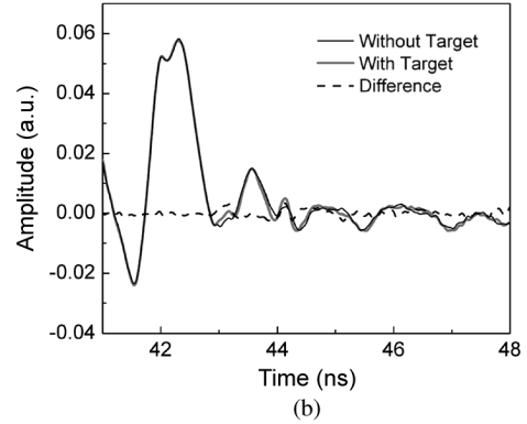
Fig. 3. Received signal for different orientations of a target when the antenna is vertically polarized. (a) The rod is placed at the focus vertically (copolarized). (b) The rod is placed at the focus horizontally (cross-polarized).
