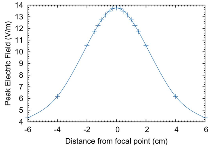
Fig. 14. Spot size for the T4FASC-SPV configuration.
