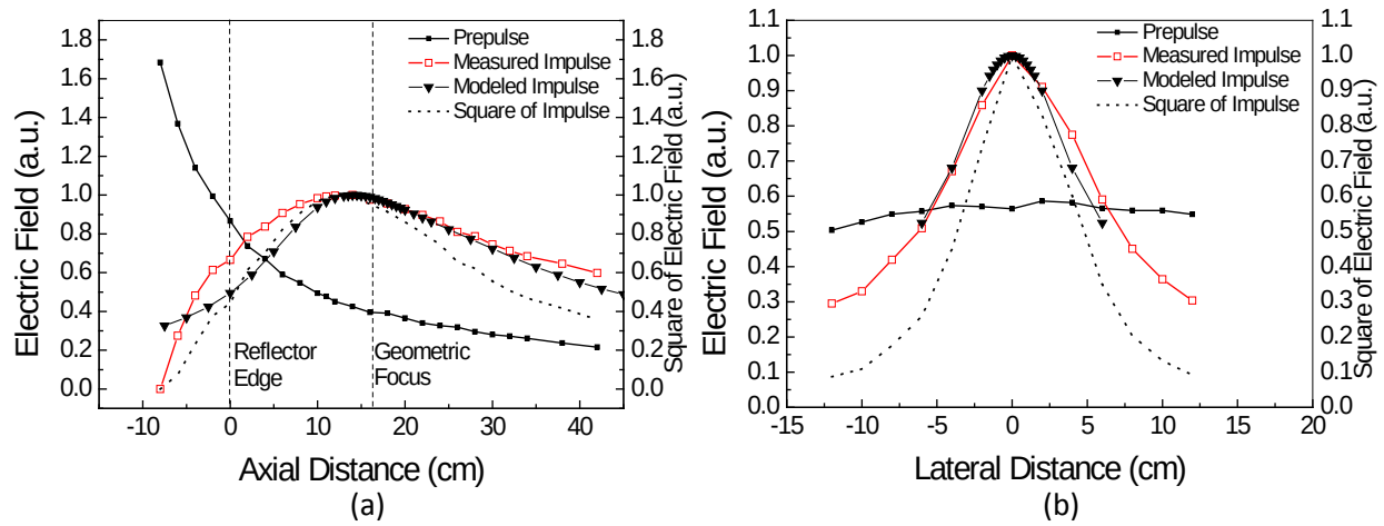
Fig.3. (a) Measured electric field (x-directed) distribution along the axis (z-axis). The prepulse, the impulse, and the square of impulse are shown. The curve with down-triangle symbols is the modeled impulse distribution along the z-axis. (b) The measured electric field (x-directed) distribution in the lateral direction (along the y-axis) at the focal plane. The prepulse, the impulse, and the square of impulse are shown. The curve with down-triangle symbols is the modeled impulse distribution in y-axis.
