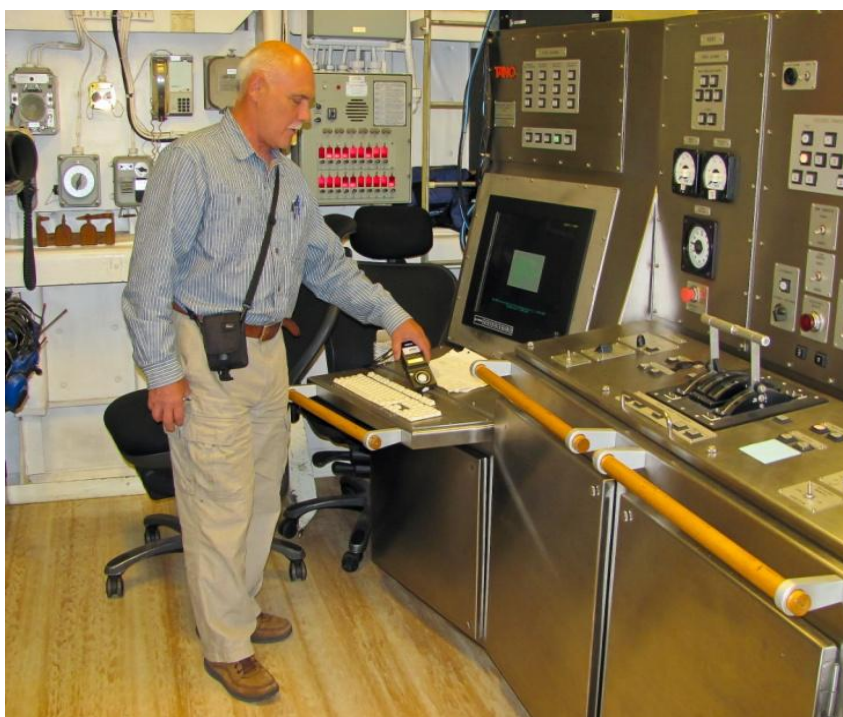
Figure 5. CGC IDA LEWIS ECC with fluorescent lighting illuminance measured at 350 lx.
