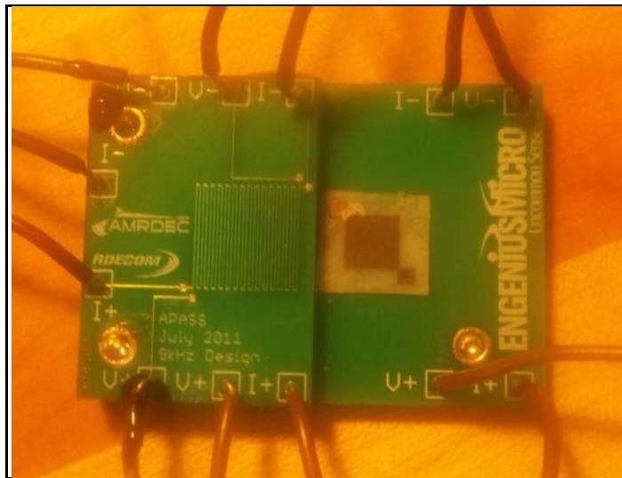
Figure 8. Experimental Board with Heater Element
