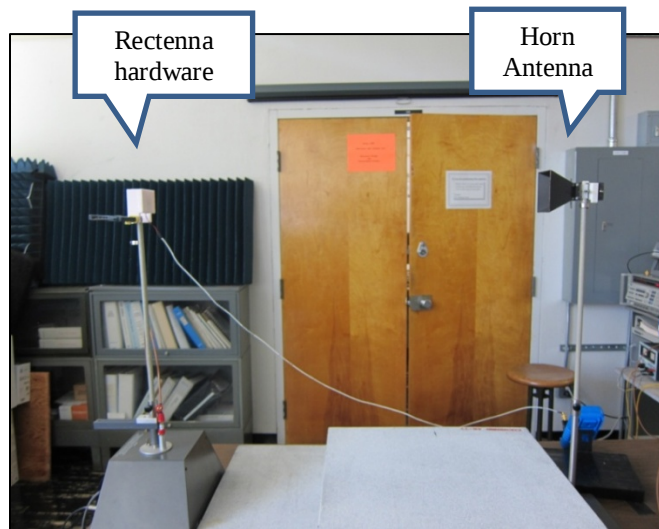
Figure 46. Hardware test setup in the microwave laboratory.
