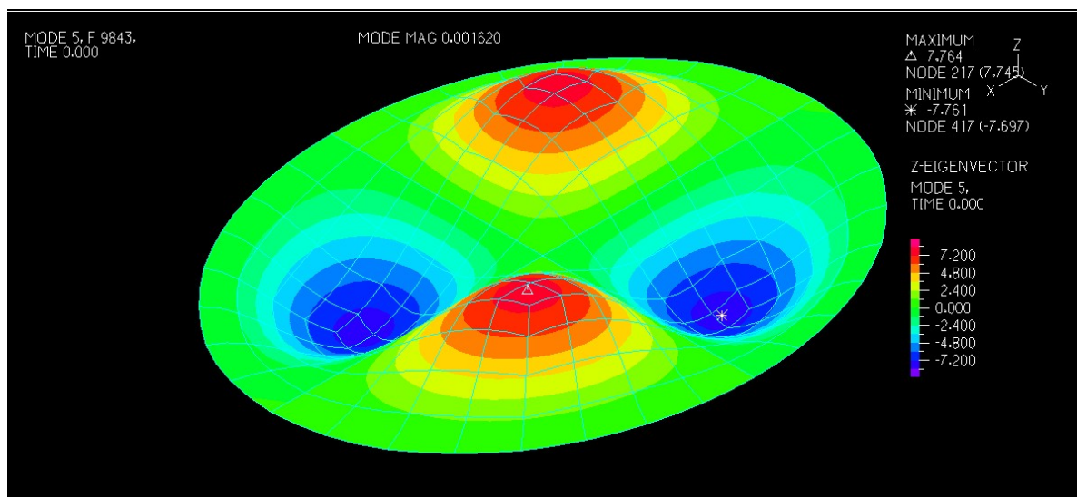
Figure D10: Finite element analysis representation of fifth vibration mode (notional to show mode shape, units negligible)
