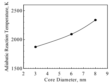
Fig. 3. Adiabatic reaction temperature vs. core size for a 1 nm thick shell
