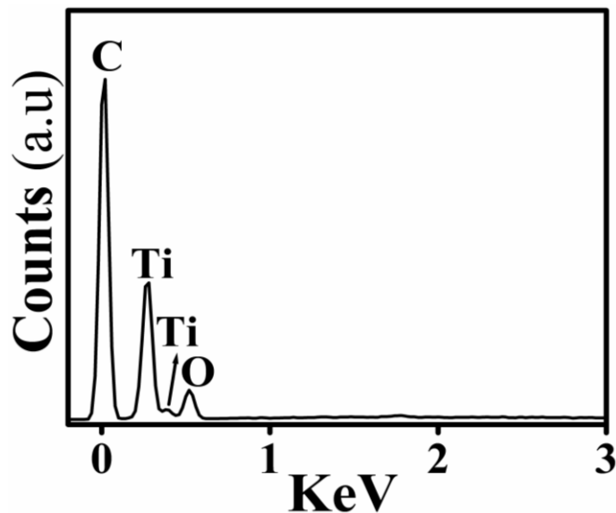
Figure 4: ED spectrum of SWCNTs- \text{WO}_3 composite.
