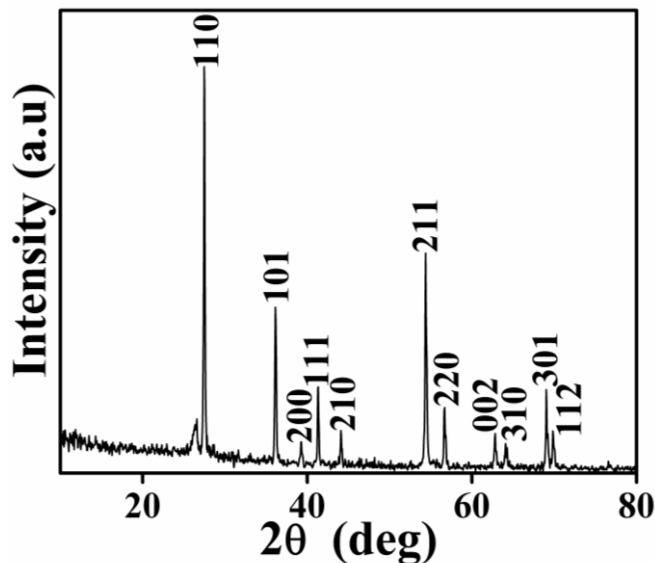
Figure 3: XRD spectrum of \text{TiO}_2 thin film.
