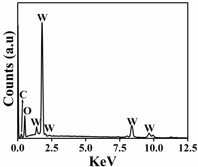
Figure 4: ED spectrum of SWCNTs- WO_3 composite.
