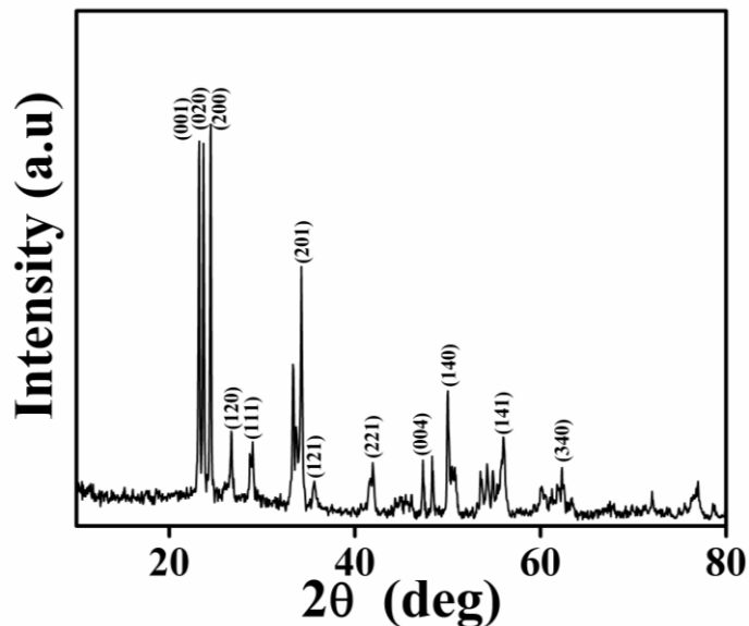
Figure 3: XRD spectrum of WO_3 thin film.
