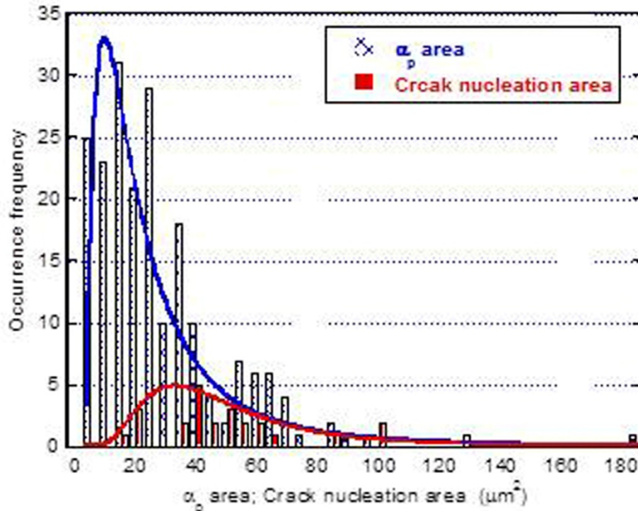
Figure 11. Histograms of primary \alpha particle sizes ( \alpha_p ) sizes (blue) as measured from metallurgical section and sizes of crack initiation regions (red) measured as projected normal to the fracture surface.
