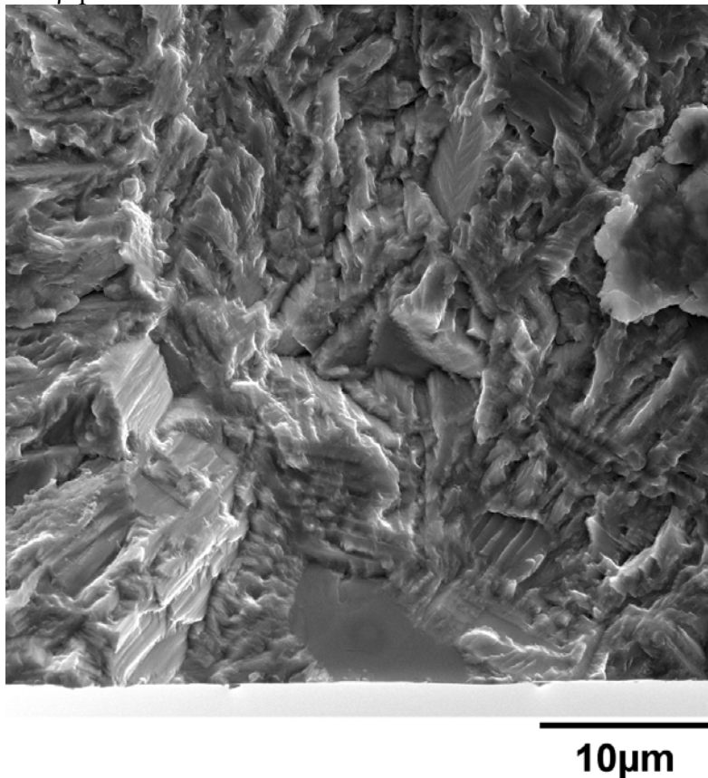
Figure 4. Typical fatigue crack origin (lower edge) showing a single, surface-connected, alpha grain facet where crack nucleation occurred.
