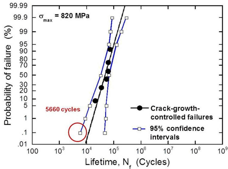
Figure 10. Lognormal regression of the Type I, shortest-life, points from alone, showing that the slope of the regression is much steeper and the B0.1 extrapolated life is much greater than shown in from the full dataset in Fig. 8.
