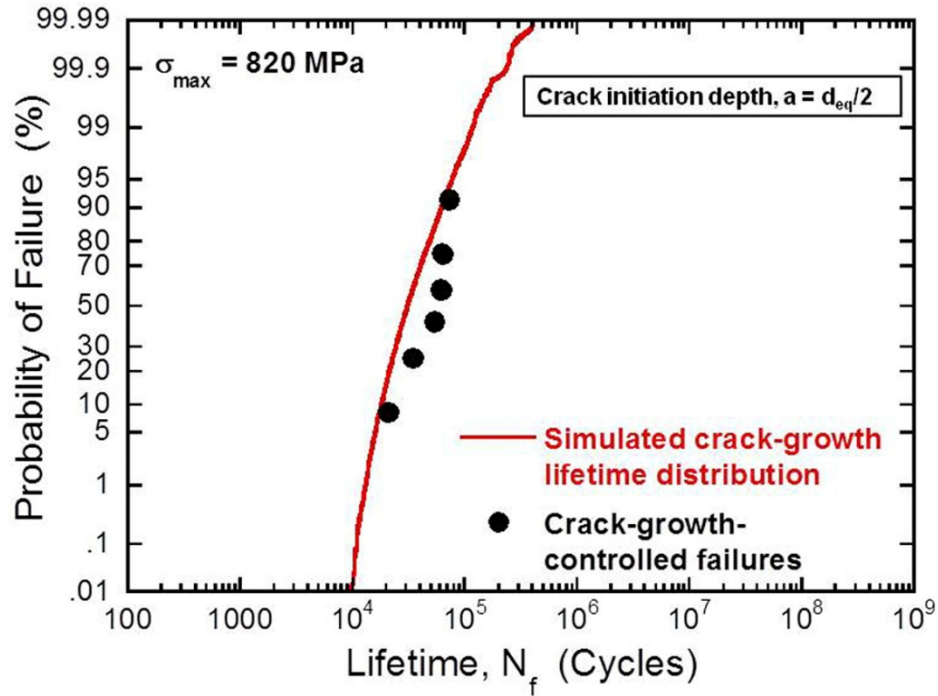
Figure 13. Probability plot of Monte Carlo model simulation of Type I fatigue lifetimes based only on microstructure (Fig. 12) and small + large crack (Fig. 13) results plotted vs. the short life data from the \sigma_{\max} = 820 MPa experiment (Fig. 9).
