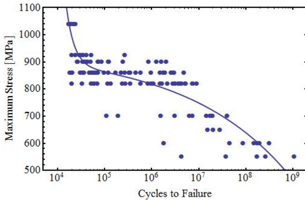
Figure 5. Ti-6246 stress vs. life (S-N) with plot showing individual specimen lifetimes and a regression line representing mean behavior. Tests above 750 MPa performed at 20 Hz, and tests below 750 MPa performed at 20 KHz.
