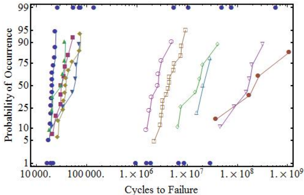
Figure 8. Lognormal probability plot of Type I and Type II fatigue lifetime data alone for individual stress levels shown in Fig. 5. From left to right: \sigma_{\max} = 1040, 925, 900, 860, 820, 860, 820, 700, 650, 600, & 550 MPa. Note that 820 and 860 MPa data each appear twice, since these stress levels exhibited both Type I and Type II behavior. As shown in Fig. 6, data from 700 and 900 MPa tests also exhibited both types of behavior, but to a lesser extent than at 820 and 860 MPa.
