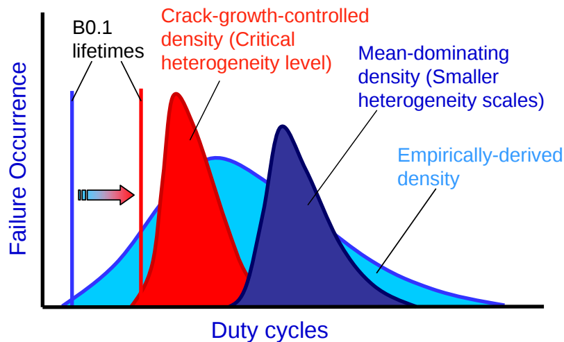
Figure 2. Expanding on the concept of “Expected Material Properties” highlighted at the upper left of Fig. 1, it is commonly assumed that fatigue variability is well described by a single probability distribution (light blue) as show above. Traditional methods of design and life management derive material life limits by extrapolation to the lower tail of the single distribution. However, it now appears that such fatigue may actually arise from at least two separate underlying probability distributions. In this sense, the identification of two distributions appears to offer substantial opportunity for improved understanding of the fundamental material behavior and a reduction in predictive uncertainty.
