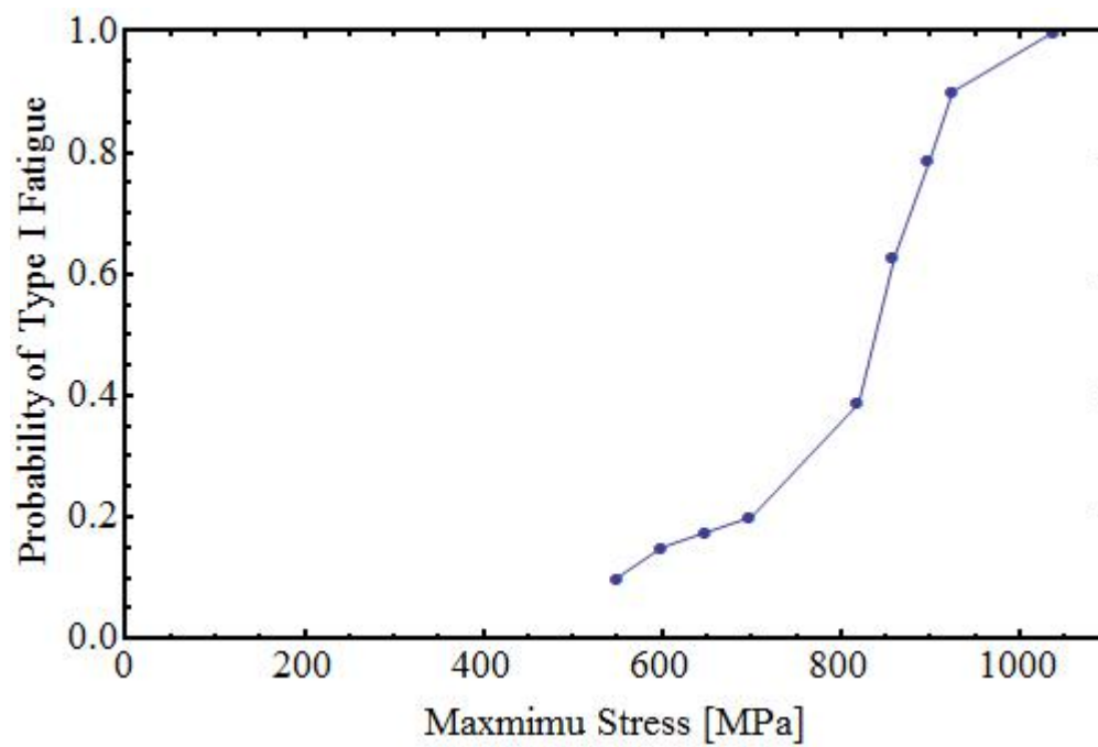
Figure 15. Probability of occurrence of Type I (short-life) fatigue based on bimodal regression analysis of fatigue lifetime data from Fig 14.
