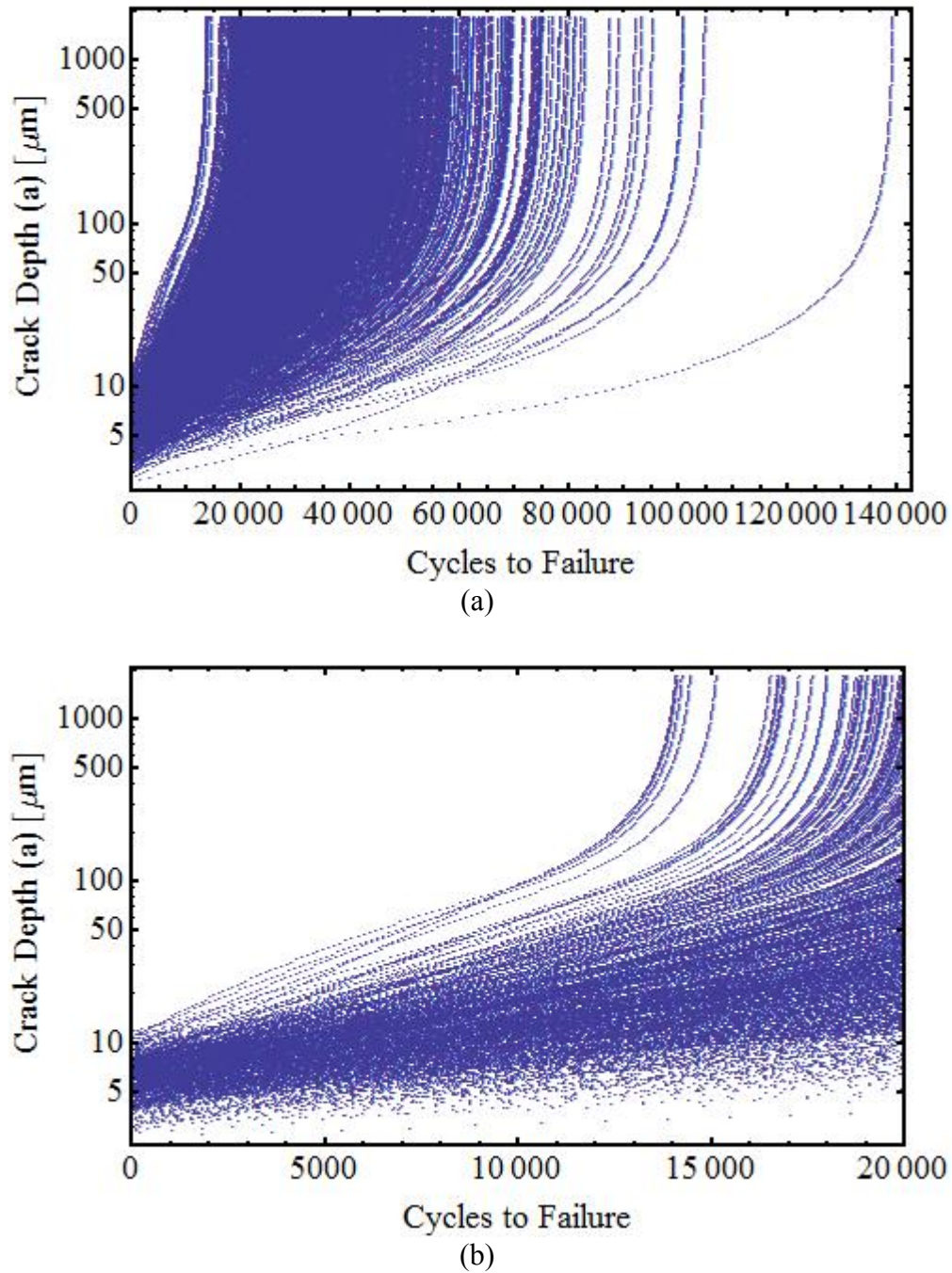
Figure 16. (a) 1000 Monte Carlo model predictions of crack depth vs. life (a-N) for a maximum stress of 820 MPa, and (b) and the same predictions on an expanded scale that shows the area of primary interest for design and life management of rotor components designed to a total lifetime of 8000 cycles (TACs)
