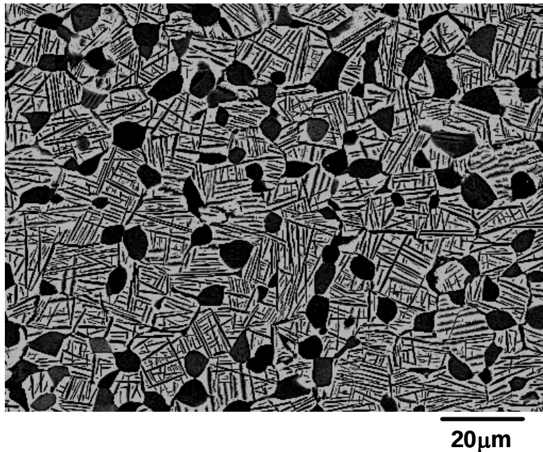
Figure 3. Nominal duplex microstructure of Ti-6Al-2Sn-4Zr-6Mo alloy processed to in the \alpha+\beta phase field, containing approximately 20% primary \alpha grains and fine \alpha -phase platelets in a matrix of transformed \beta phase.
