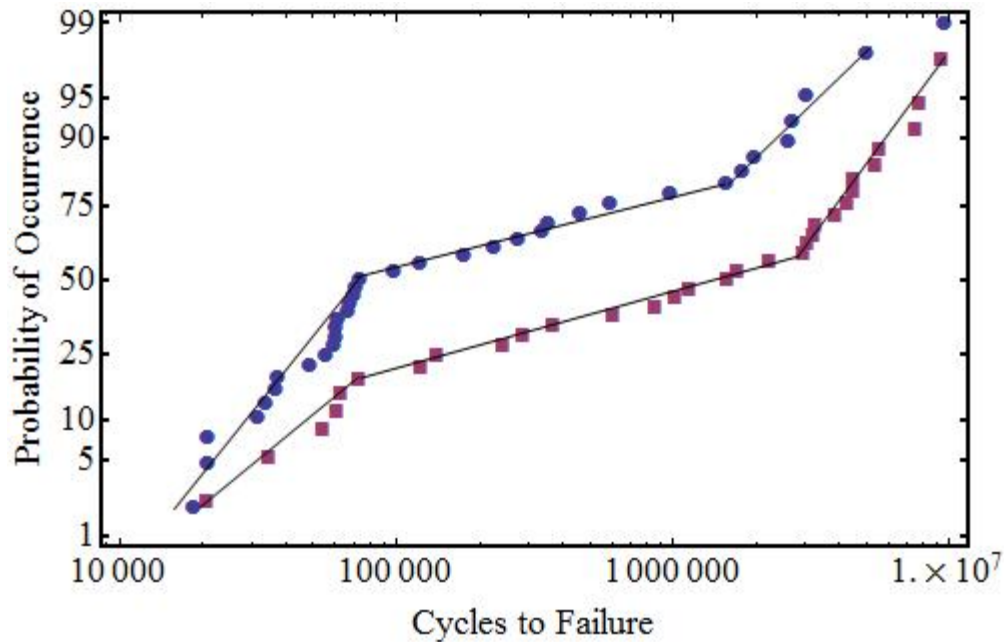
Figure 7. Lognormal probability plot showing 820 MPa and 860 MPa data from Fig. 5, highlighting three regions of the bimodal trend (Type I, transition, Type II).
