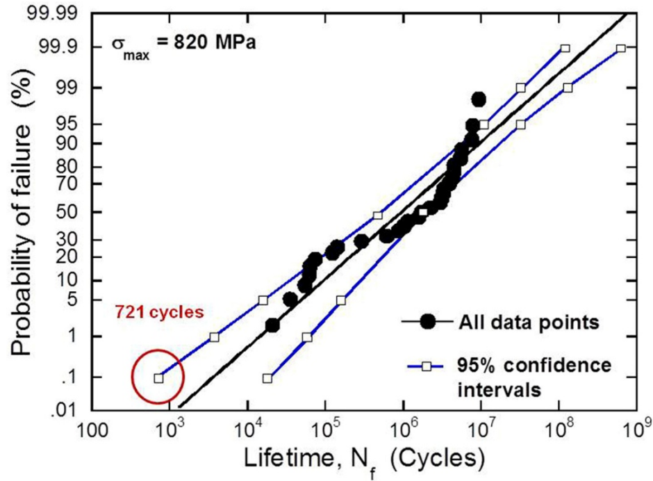
Figure 9. Lognormal probability plot of lifetime data for tests with \sigma_{\max} = 820 MPa, showing a regression extrapolation to the B0.1 (1/1000) probability of failure, along with 95% confidence bands for the fit.
