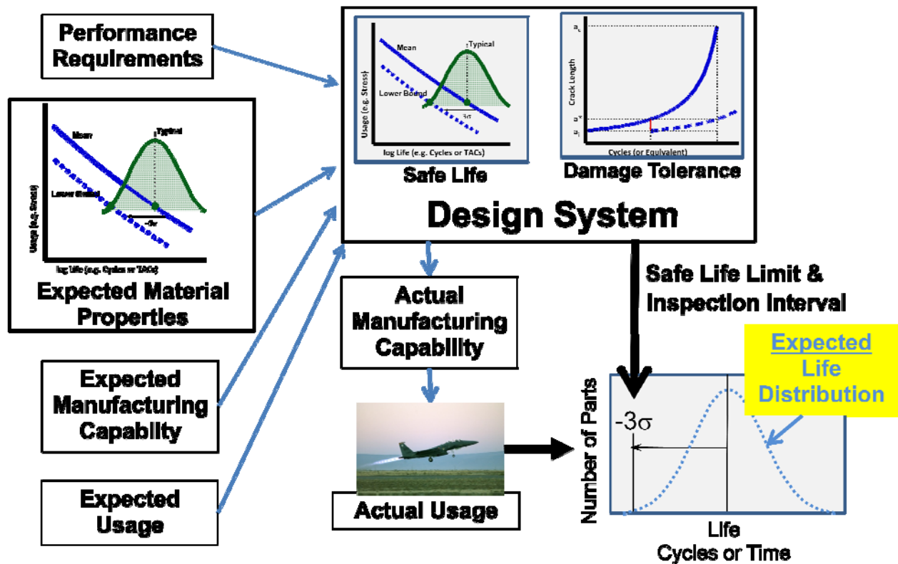
Figure 1. Schematic of design requirements and expected material/component response specified by the Department of Defense Propulsion System Integrity Program (PSIP).
