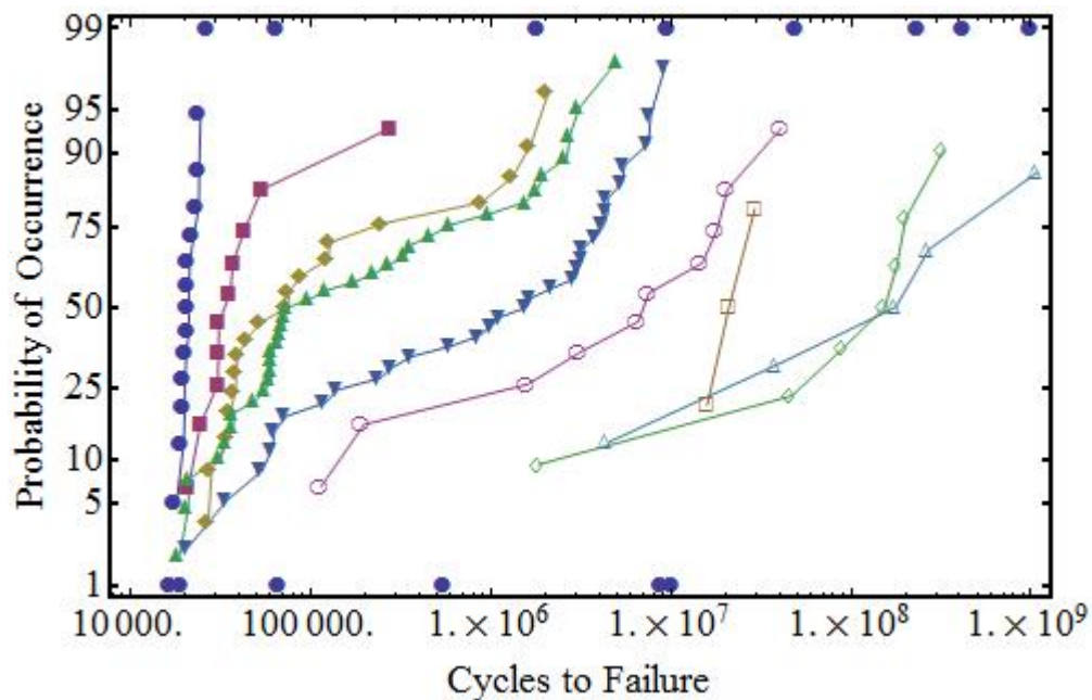
Figure 6. Lognormal probability plot of fatigue lifetime data for individual stress levels shown in Fig. 5. From left to right: \sigma_{\max} = 1040, 925, 900, 860, 820, 700, 650, 600, & 550 MPa.
