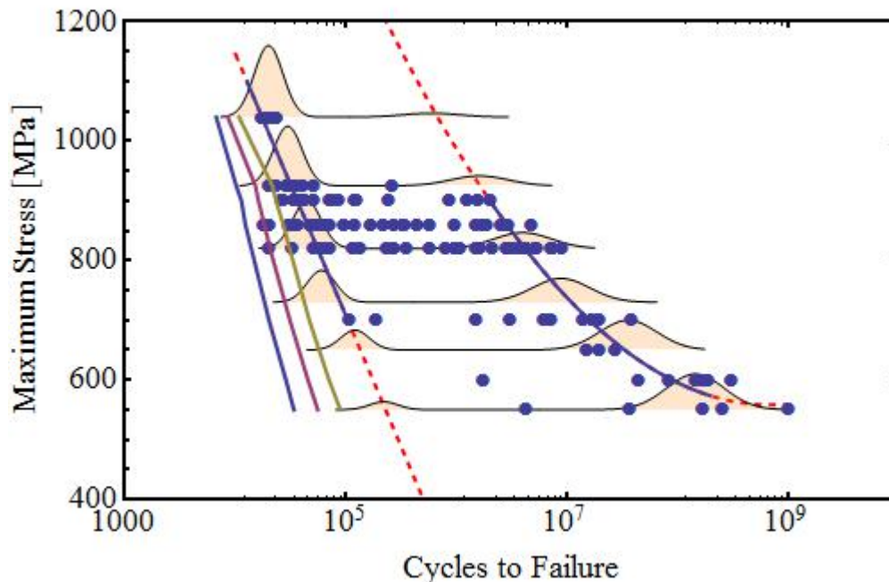
Figure 14. S-N plot showing (i) individual regression lines (blue and dashed) to Type I and Type II data, (ii) schematic bimodal probability distribution transitioning from Type I to Type II dominance with decreasing stress, and (iii) Monte Carlo predictions of 50%, 10%, and 0.1% probabilities of failure for the minimum lifetimes.
