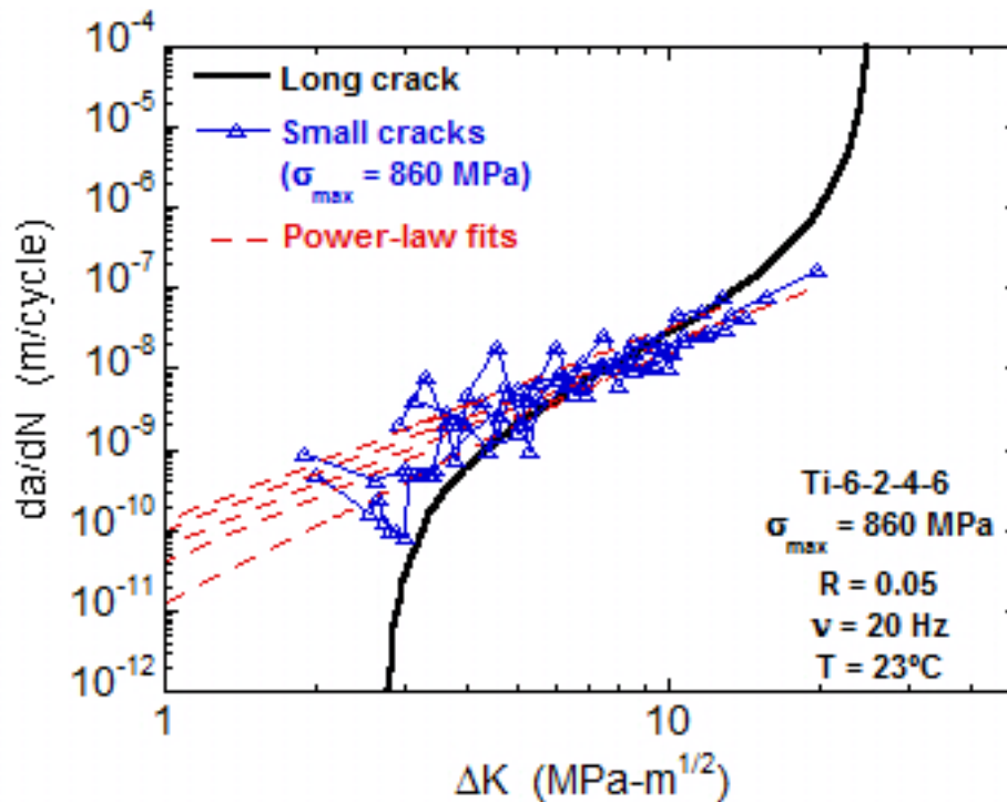
Figure 12. Plot of da/dN vs. \Delta K for several naturally initiated small surface cracks measured via acetate replication of the specimen surface, and regression trend from similar data on large cracks in conventional compact type C(T) specimens.
