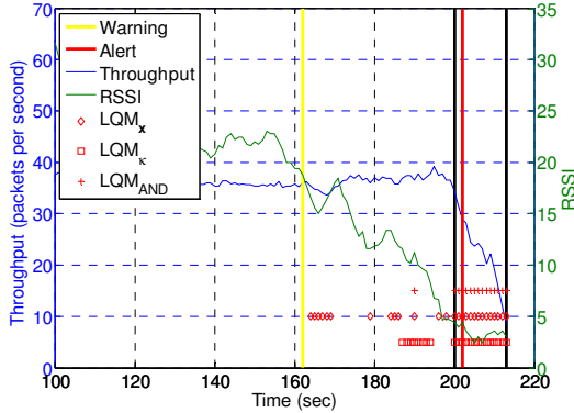
Figure 8: LQ estimator warning and alert. A warning is issued based on RSSI and an alert based on throughput.
