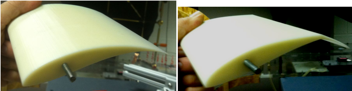
Figure 14. Fabricated RP airfoils: a) Continuous morphed profile, b) Discontinuous flap.
