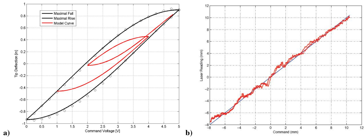
Figure 7. Hysteresis nonlinearity: a) Example of MFC bimorph hysteresis loop, b) Inversion of hysteresis nonlinearity resulting in near linear output.
