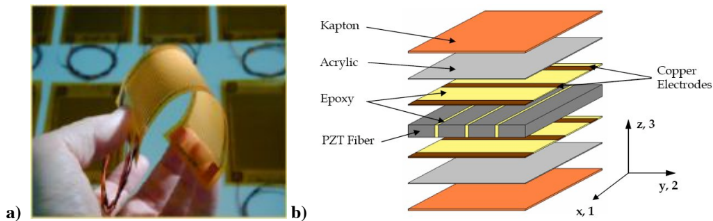
Figure 1. Macro Fiber Composite (MFC): a) Flexible nature of MFC b) Exploded view of construction [1].
