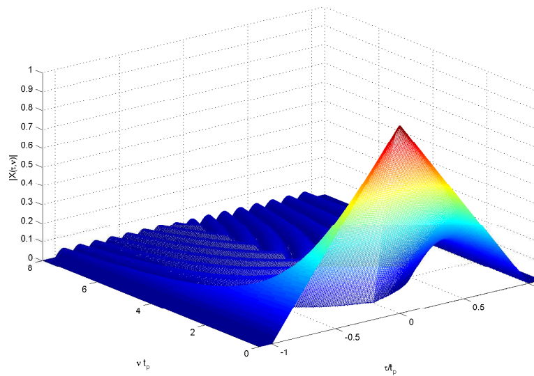
Figure 1a: Ambiguity function of a constant frequency rectangular pulse of length t_p .
