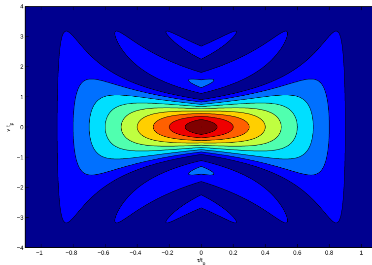
Figure 1b: Ambiguity function contours of a constant frequency rectangular pulse of length t_p .
