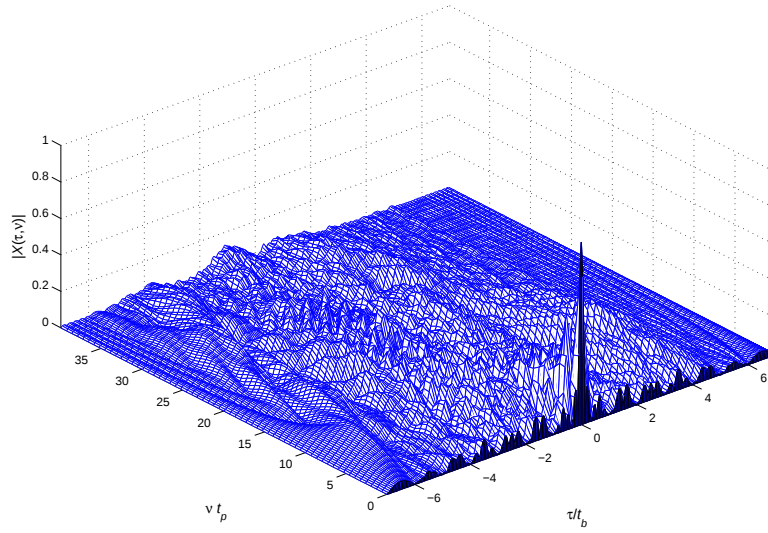
Figure 4a: Ambiguity function of a Costas signal with coding sequence (3, 6, 0, 5, 4, 1, 2).
