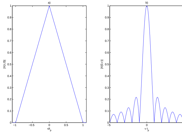
Figure 1c: Ambiguity function of a constant frequency rectangular pulse of length t_p . a) Zero-Doppler cut. b) Zero-delay cut.
