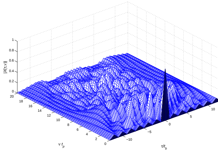
Figure 7b: Ambiguity function for a 13-element Barker code.
