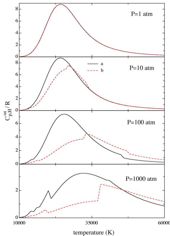
Fig. 1.2. Internal specific heat of atomic hydrogen as a function of temperature at different pressures (curves a-b as explained in the text).
