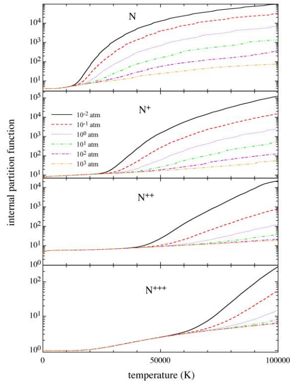
Fig. 1.8. Electronic partition function of N, N + , N 2+ , N 3+ species as a function of temperature at different pressures.
