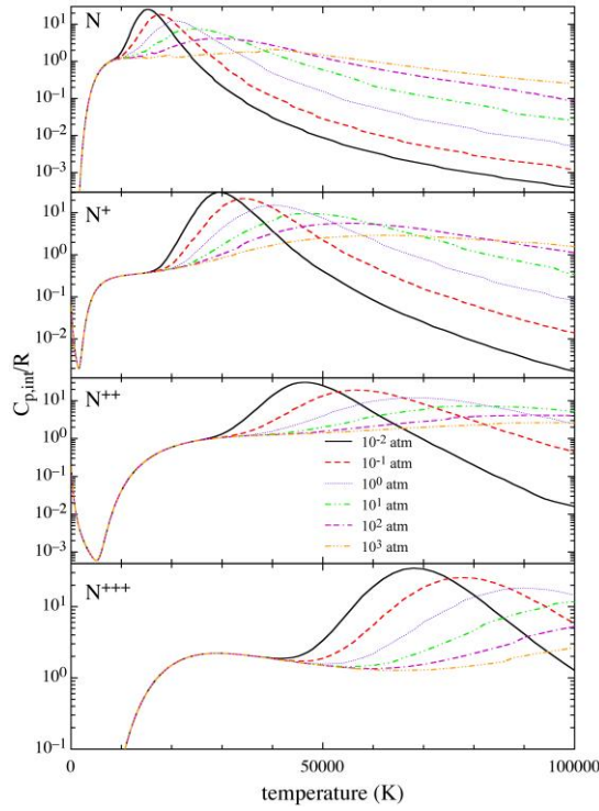
Fig. 1.9. Internal specific heat of of N, N + , N ++ , N +++ species as a function of temperature at different pressures.
