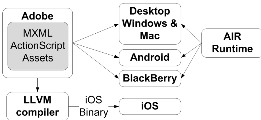
Exhibit 7 Cross-platform development methodology using the Adobe AIR runtime
