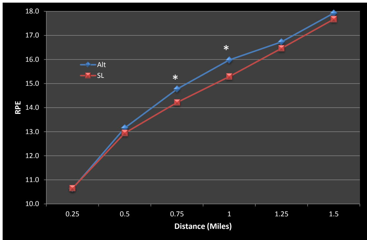
Figure 11 – RPE's during 1.5 mile runs at ALT and SL. Significant differences ( p < 0.05 ) were seen between runs at the .75 and 1.0 mile intervals.
