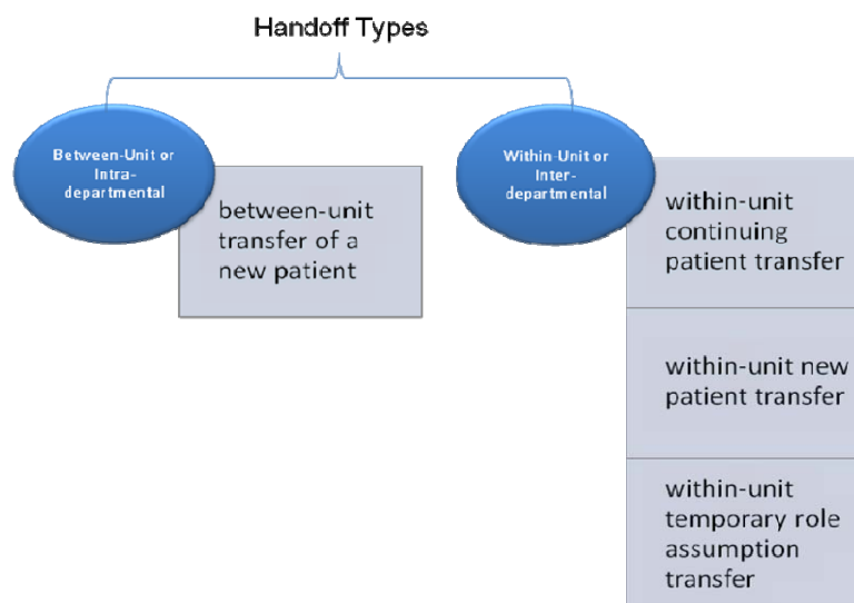
Figure 1: Handoff Types
