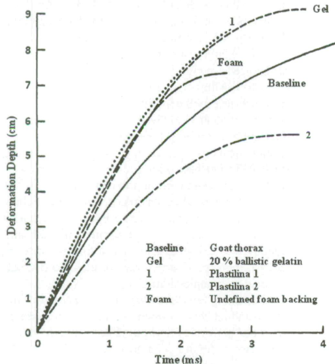
FIGURE 2. Assessment of potential backing materials. 23
