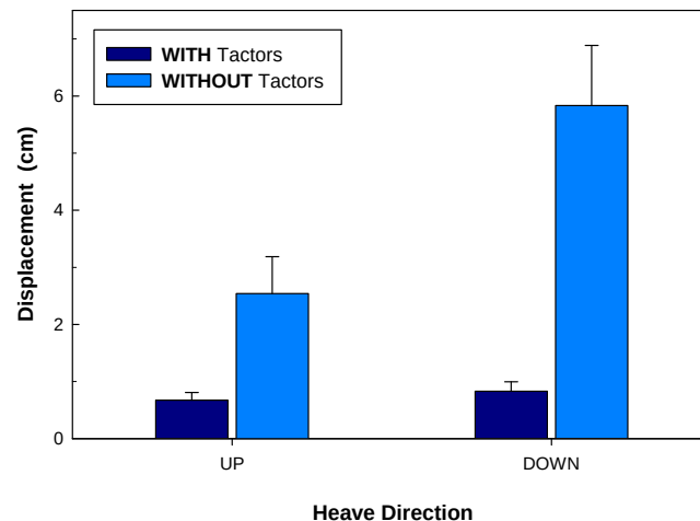
Figure 4: Final displacement with and without tactors in the two heave directions.
