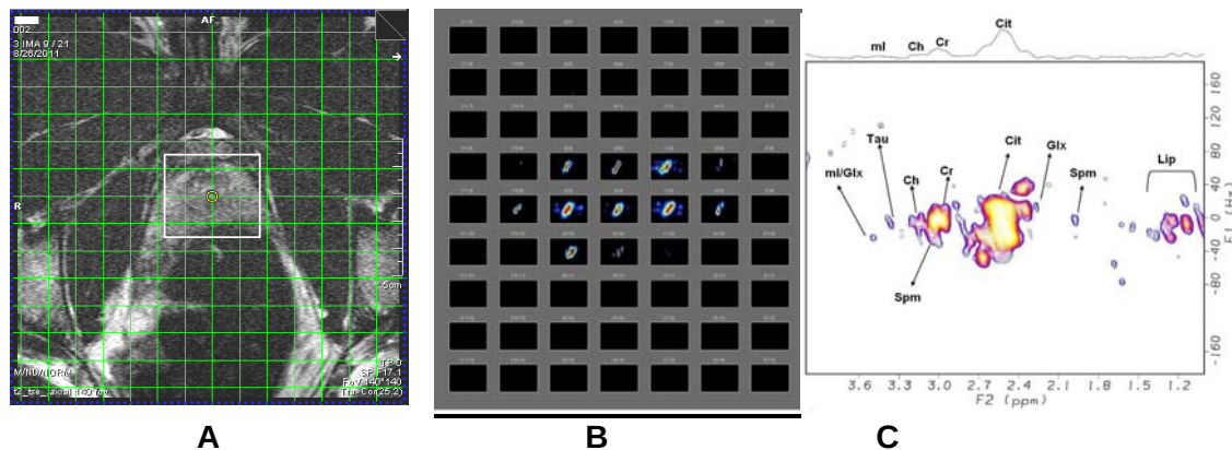
Figure 3. A. An axial MRI slice of the 32y.o. healthy male subject showing the VOI and MRSI grids. B. Expanded multi-voxel 2D spectra showing the Cit multi-voxels. C. The 2D J-resolved spectrum extracted from a 2ml voxel of the peripheral zone.
