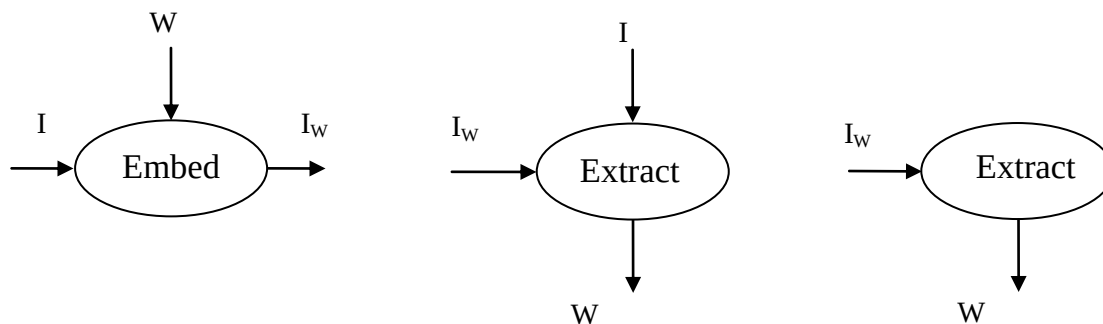
Figure 1: (a) Embedding the information I with the watermark W creates I_w . (b) Extraction of W from I_w is done with information from I . (c) Extraction of W from I_w is done without any information from I .
