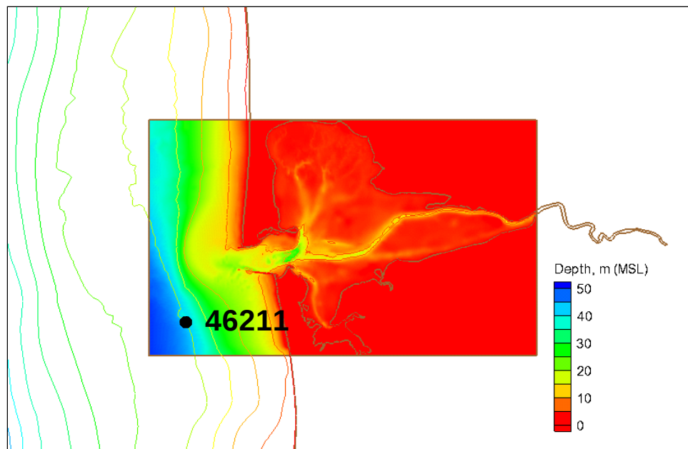
Figure 3-5. Model domain for the Grays Harbor CMS-Wave model.
