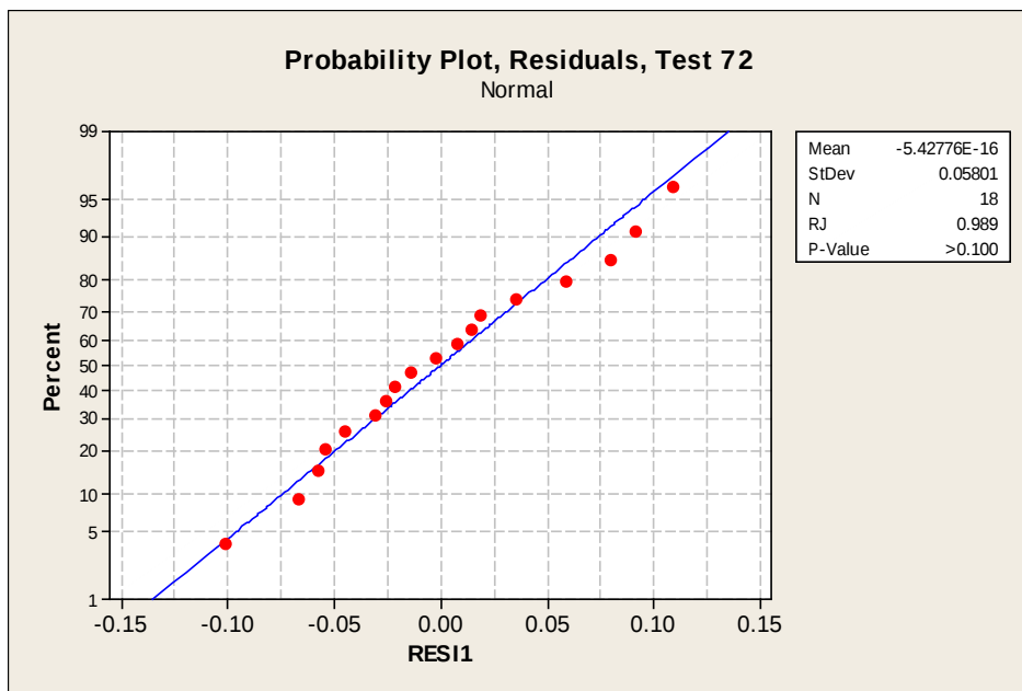
Figure 2- 29 – Test 72 residual probability plot
