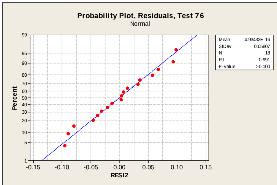
Figure 2- 30 – Test 76 residual probability plot
