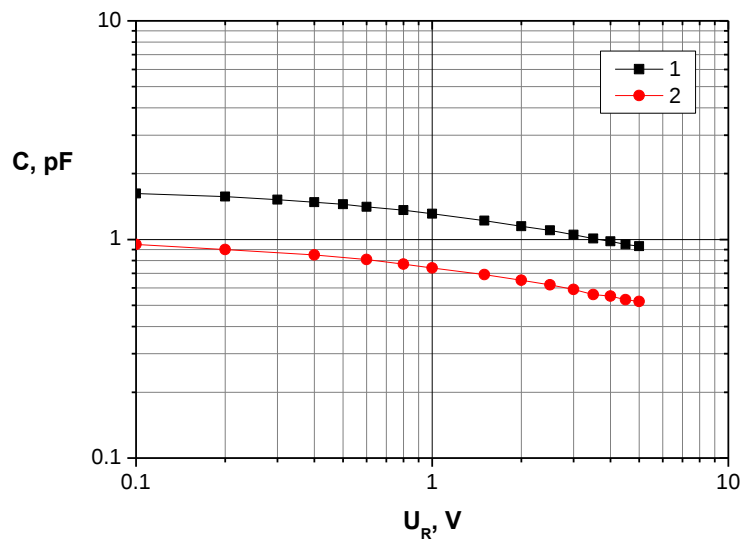
Figure 35. Capacitance ( C ) of beam-lead IMPATT diodes as function of reverse voltage ( U_R ). 1 – before etching, 2 – after silicon mesa etching for 7 sec.
