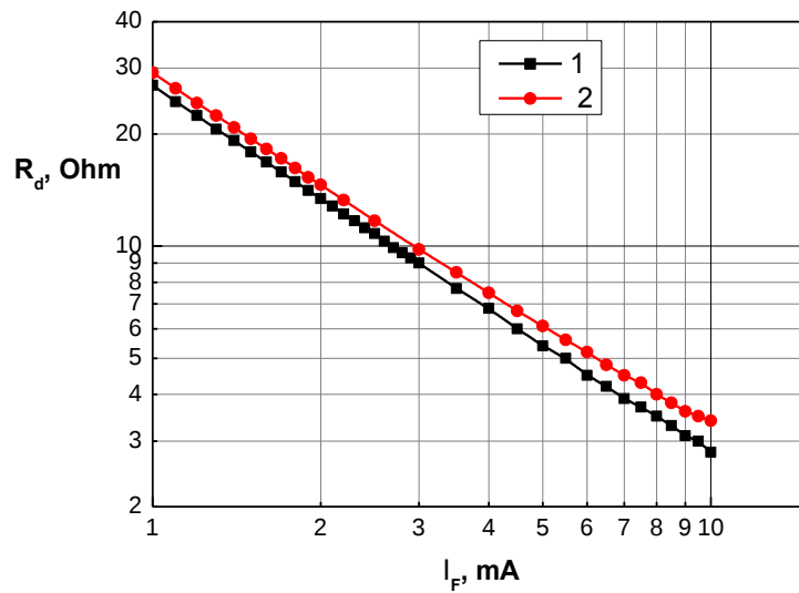
Figure 36. Differential resistance ( R_d ) of beam-lead IMPATT diode model as function of forward current ( I_F ). 1 – before etching, 2 – after silicon mesa etching for 7 sec.
