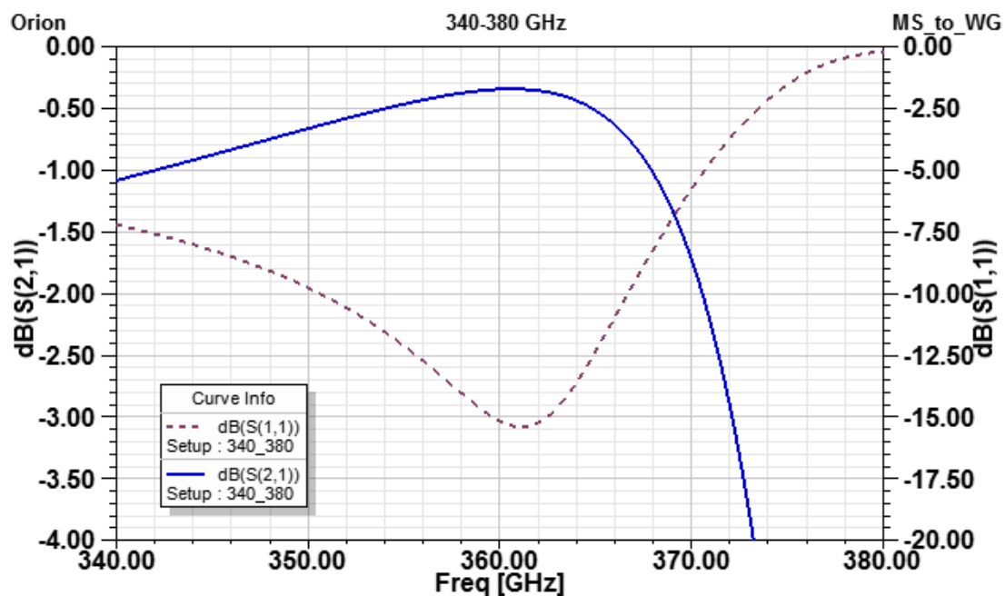
Figure 15. Transmission ( S_{21} ) and reflection ( S_{11} ) coefficients of a transition from a microstrip line to rectangular waveguide WR-2.8 obtained with HFSS.
