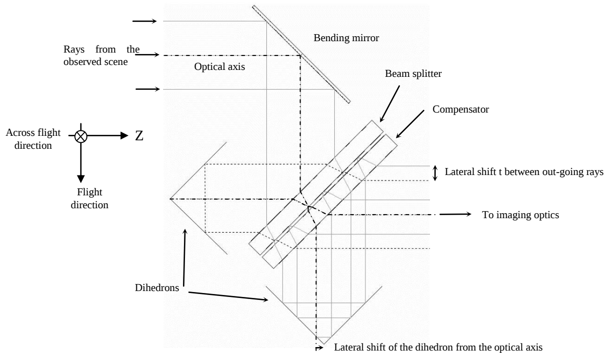
Figure 3. Interferometer principle
