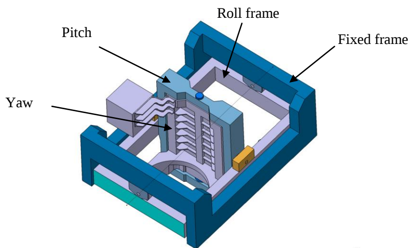
Figure 6. Stabilization platform mechanical design
