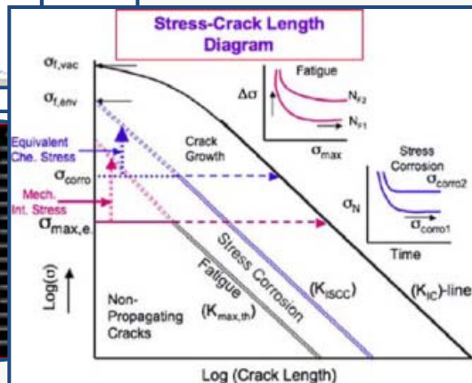
Modified Kitagawa Diagram
