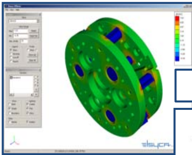
Corrosion rates on complex structures
