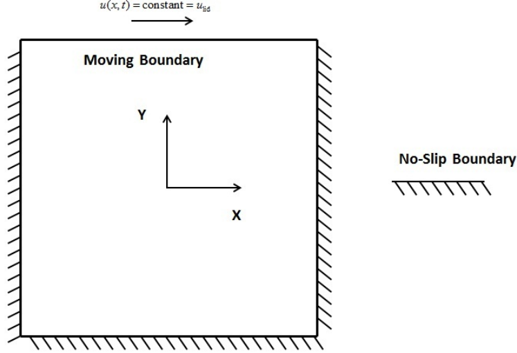
Figure 23: Schematic of the two-dimensional lid-driven cavity problem.
