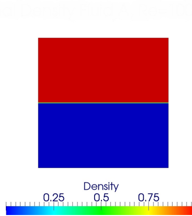
Figure 73: Density for Fluid 1 of a two-component immiscible fluid flow in a lid-driven cavity. Initial configuration.
