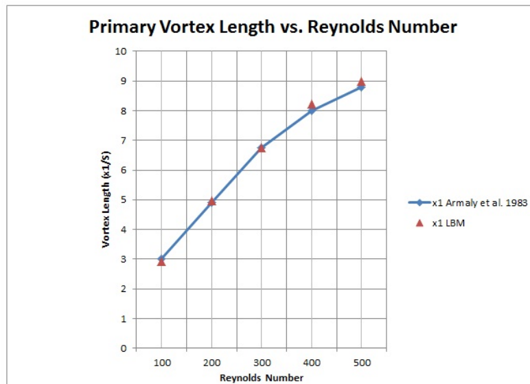
Figure 22: Comparison of primary vortex re-attachment length normalized by step height with results reported in [35].
