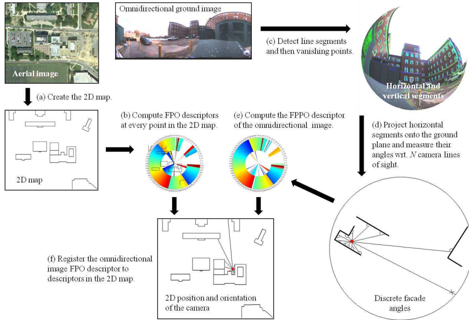
Figure 1. Overview of our localization approach. A 2D map is manually created from an aerial image and FPO descriptors are computed at each point in this map. Given an omnidirectional ground image for an unknown camera location, line segments and vanishing points are detected in the image. Horizontal line segments are projected onto the ground plane and from these the query FPO descriptor is computed. The query FPO descriptor is registered to those of the 2D map to determine the position and orientation of the camera.
