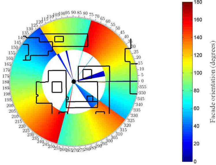
Figure 5. The color-coded relative orientations computed for the map point at the star. At every viewing direction from 0 to 359°, up to two facade orientations (between 0 and 180°) are identified. Each ring represents a cluster of facade orientations for each of the 360 viewing directions. The entry for a viewing direction is white when no clusters are identified for that viewing direction. The inner ring only is white when only one cluster of orientations is identified.
