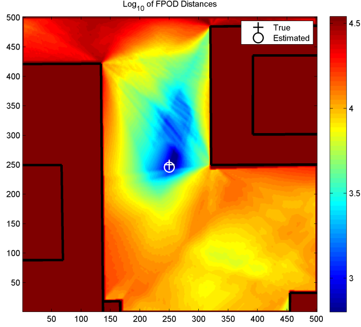
Figure 8. Logarithm of the distances between the FPO descriptor computed for the image in figure 6 and the FPO descriptors for the map shown in figure 5.
