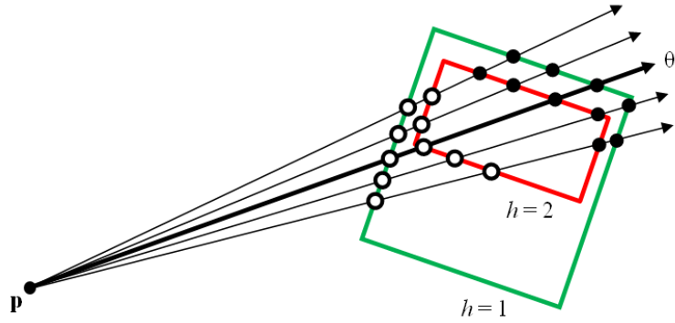
Figure 4. Sampling the rays emanating from a point \mathbf{p} in the direction \theta_i . Segments on the green facade have relative height 1 and segments on the red facades have relative height 2. The white points contribute to the angles measured for direction \theta_i of point \mathbf{p} , but the black points do not because their heights do not increase relative to points closer to \mathbf{p} ; the black points are not visible because they are on the back side of the building. In this case, the angles associated with the white points will form two clusters, one cluster corresponding to the seven points on the two left-side facades and one cluster corresponding to the three points on the bottom red facade.
