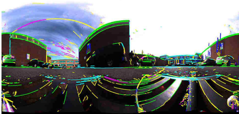
Figure 6. An omnidirectional image (acquired from the position shown in figure 5) and detected image line segments color-coded according to their 3D orientation. Yellow line segments do not align with any vanishing point. All other colors correspond to a known vanishing point and 3D orientation.
