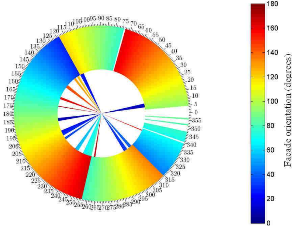
Figure 7. FPO descriptor computed from the omnidirectional image shown in figure 6.
