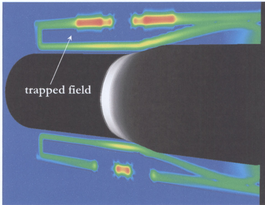
Figure 2. Helical MFC at later time (device not pictured).
