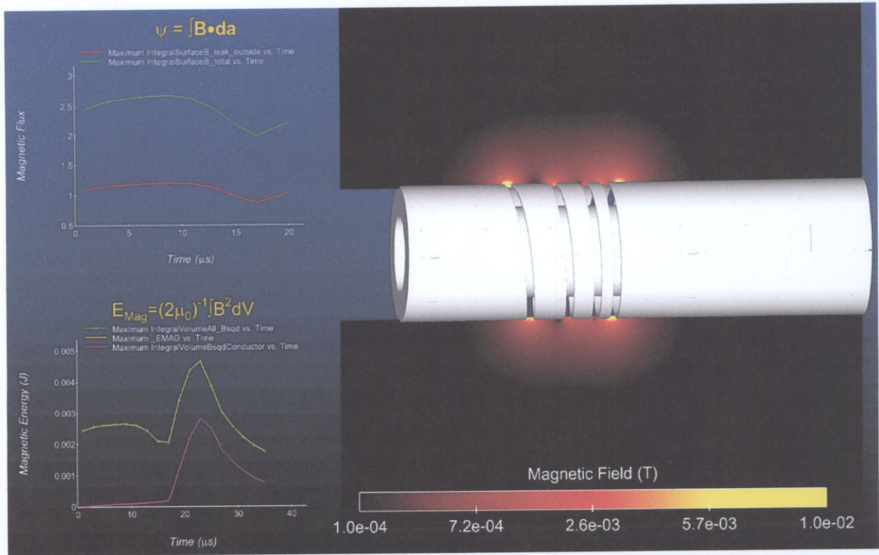
Figure 9. Quantifying magnetic energy partitioning.
