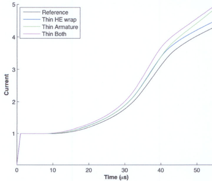
Figure 8. System performance as a function of armature velocity.
