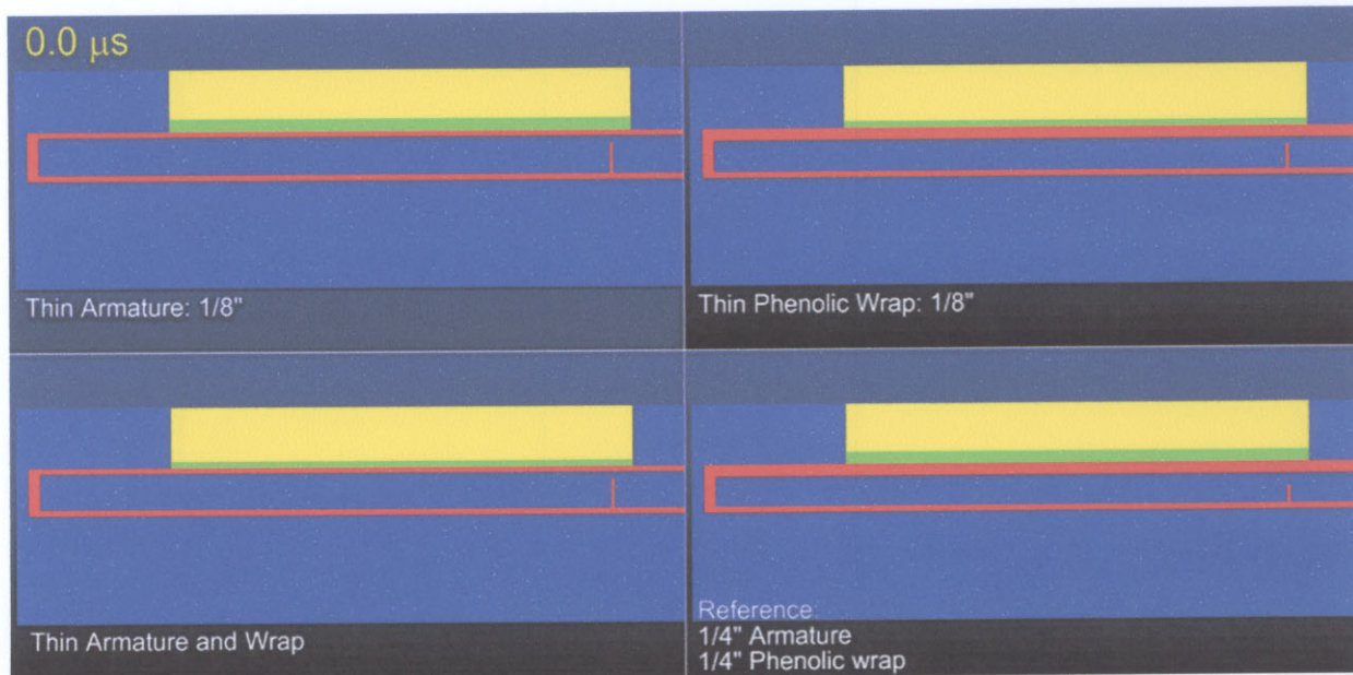
Figure 7. Configurations for evaluating the effects of armature velocity on system performance.
