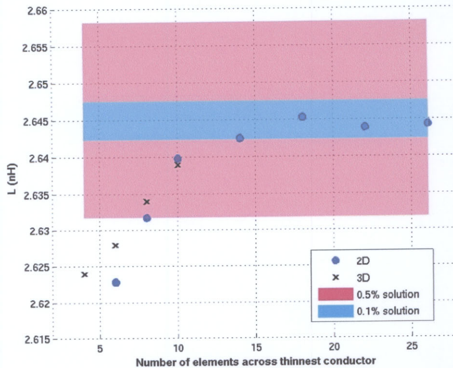
Figure 3. Inductance convergence for a 2-D and 3-D coaxial cable.
