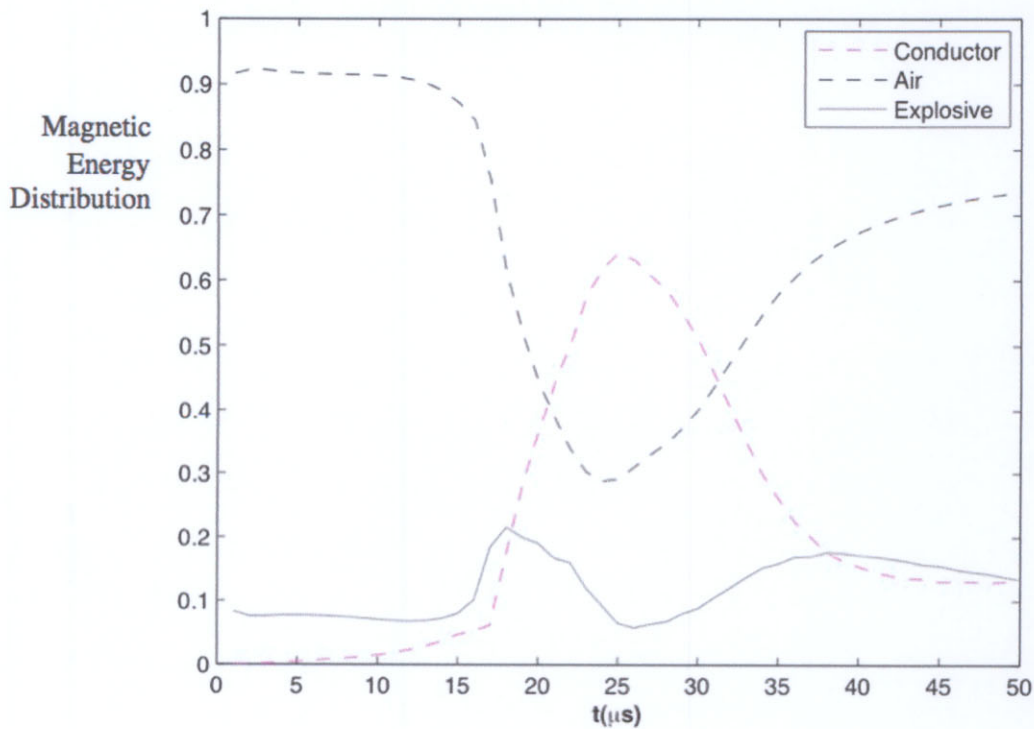
Figure 10. Normalized magnetic energy partitioning.
