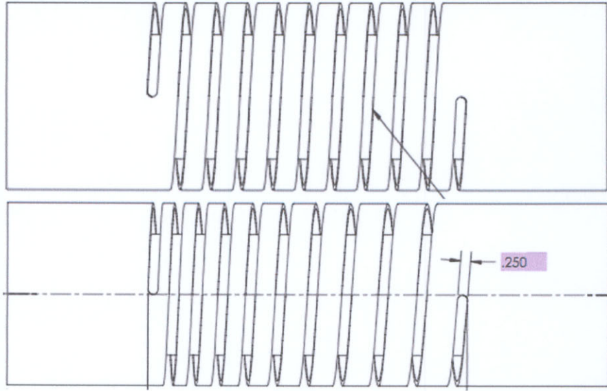
Figure 4. Typical constant and variable pitch Helicoils.
