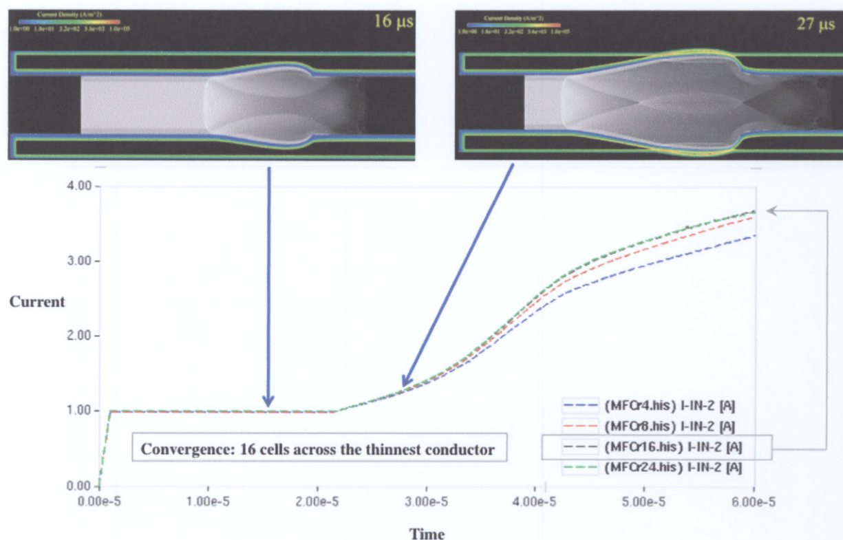
Figure 6. Impact of mesh resolution on current gain for a 2-D coaxial MFC.
