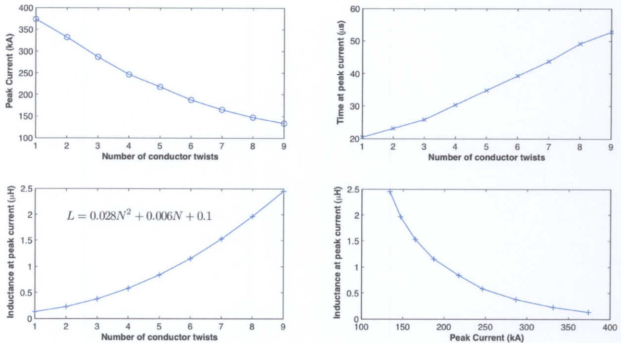
Figure 5. Inductance and current scaling behavior for a Helicoil.
