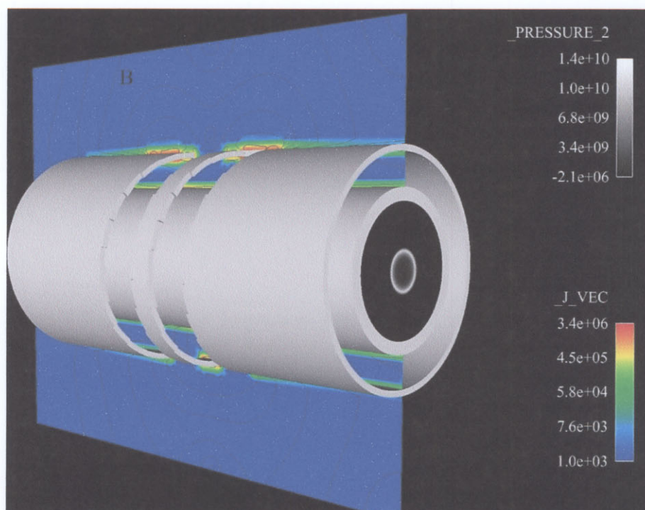
Figure 1. Helical MFC at early time.
